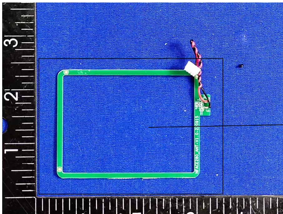
13.56MHz Antenna
