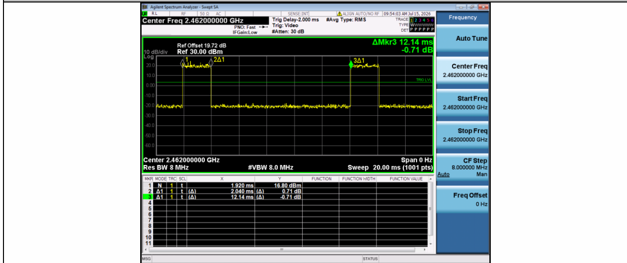
NTNV-11G-Ant1-2462
