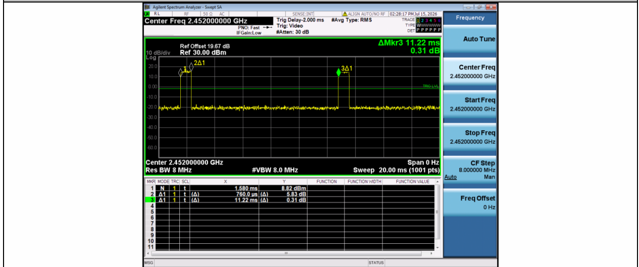
NTNV-11AX40SISO-Ant1-2452
