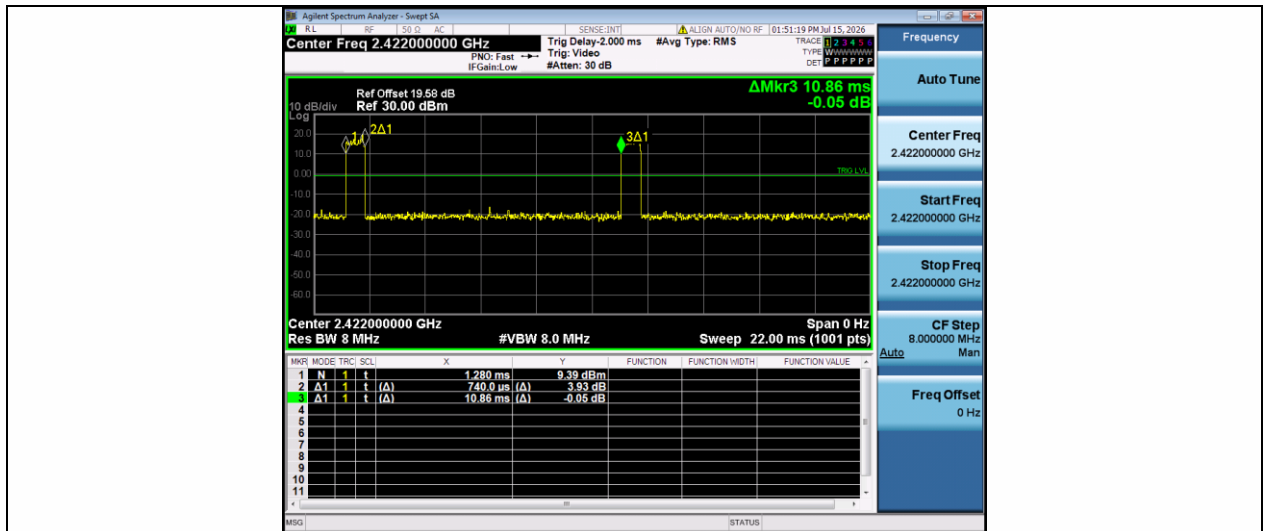
NTNV-11AX40SISO-Ant1-2422
