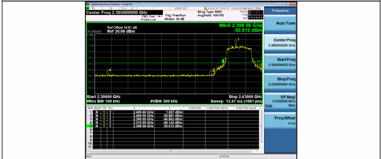
11AX20SISO-Ant1-2412-PASS
