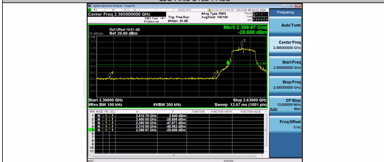
11N20SISO-Ant1-2412-PASS
