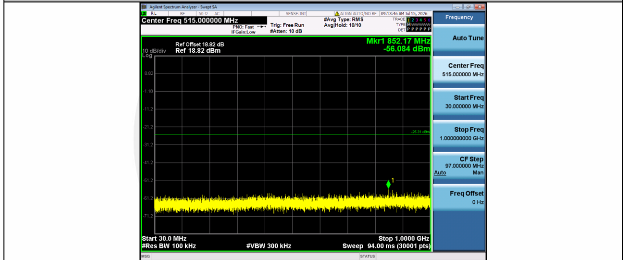
11B-Ant1-2412-30~1000-PASS
