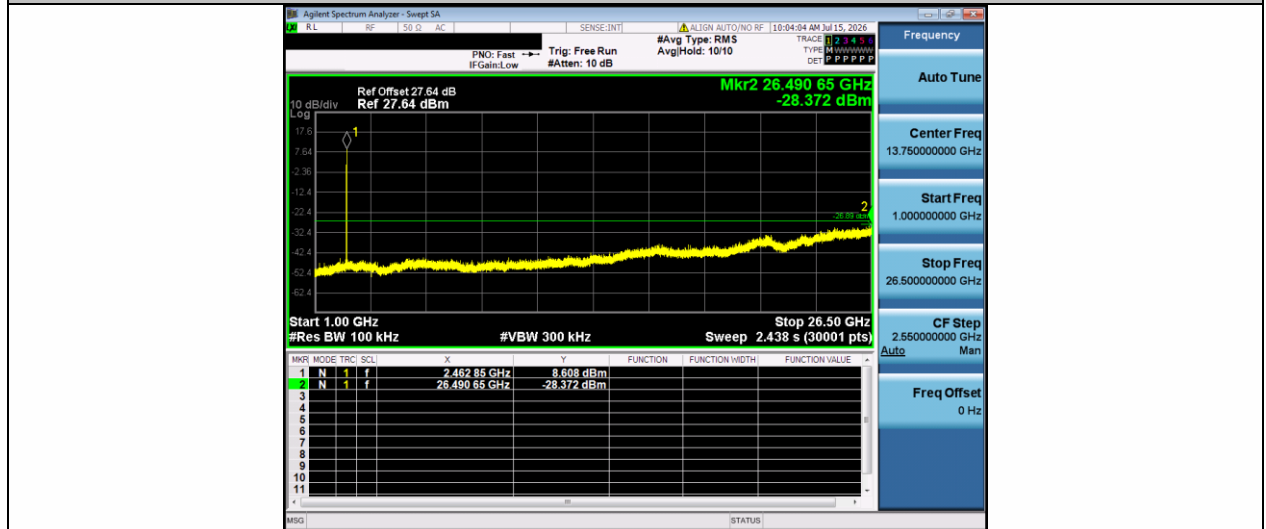
11G-Ant1-2462-1000~26500-PASS
