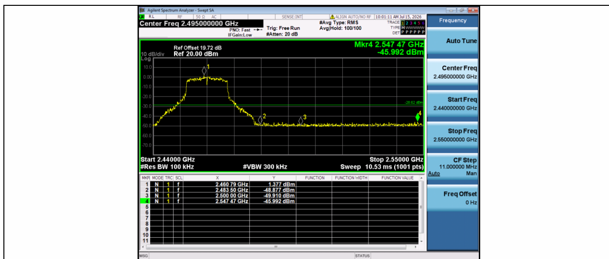
11G-Ant1-2462-PASS
