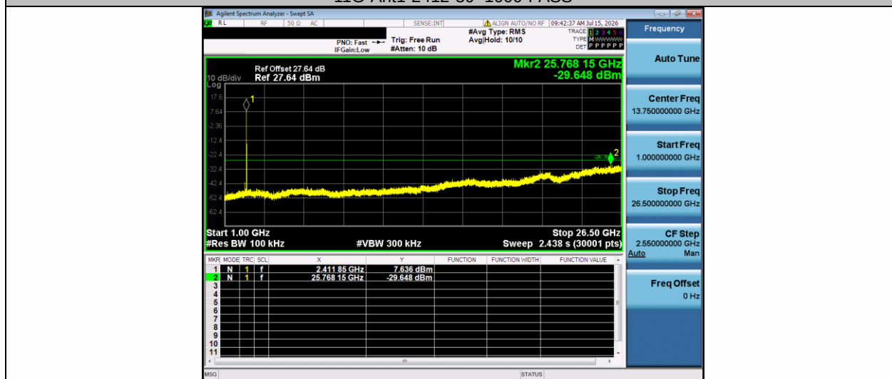
11G-Ant1-2412-1000~26500-PASS
