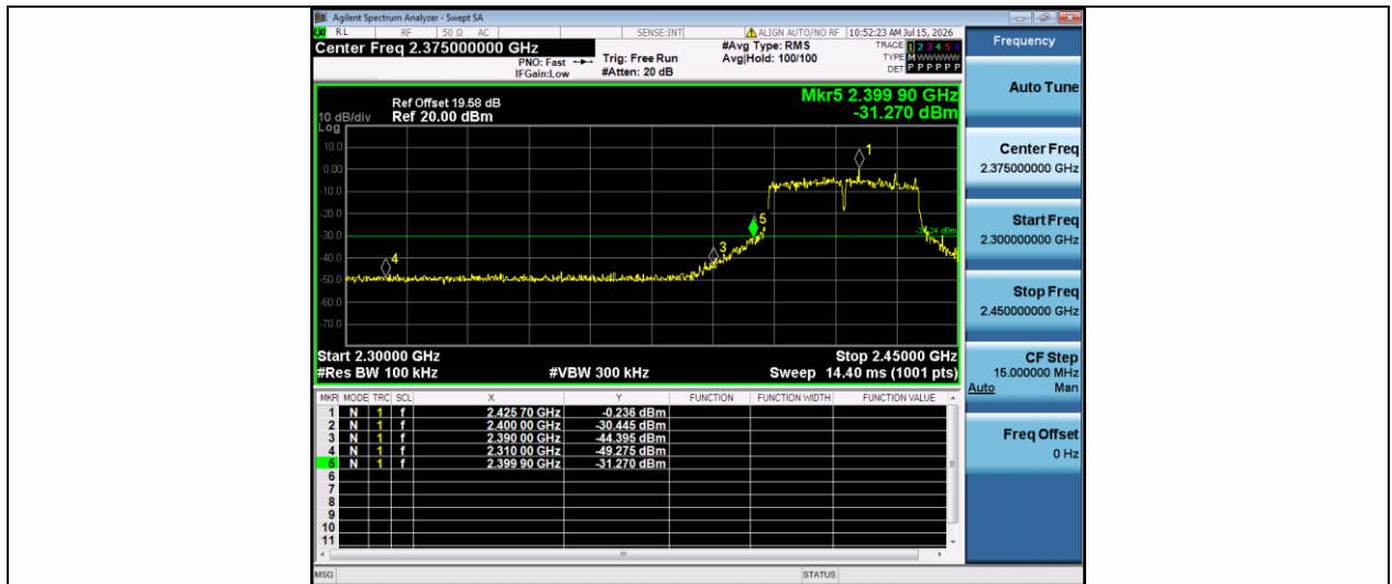
11N40SISO-Ant1-2422-PASS
