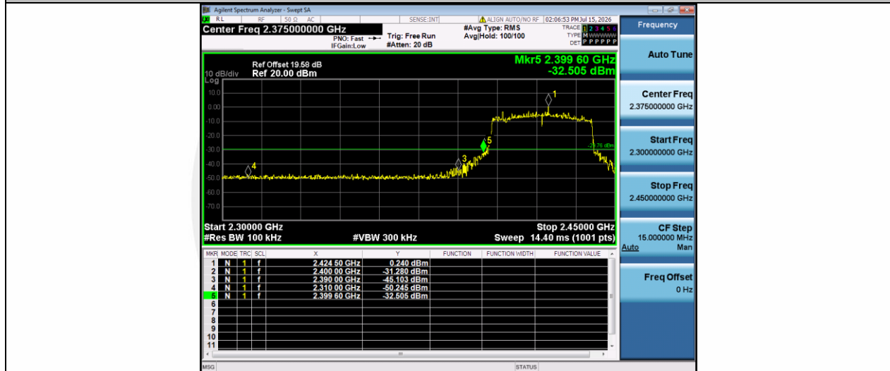
11AX40SISO-Ant1-2422-PASS
