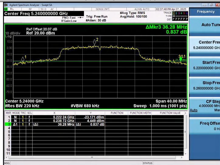
11AC20SISO-Ant1-5240
