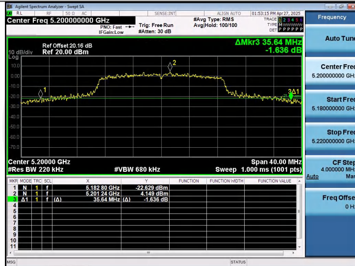
11N20SISO-Ant1-5200
