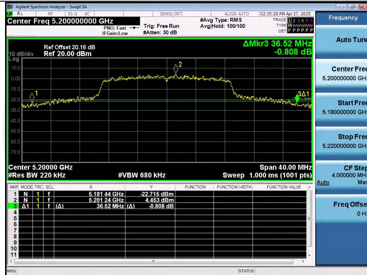
11AC20SISO-Ant1-5200
