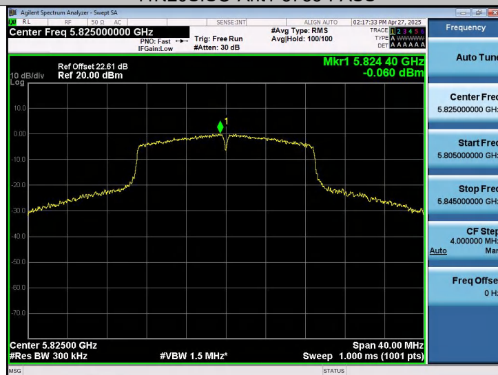
11N20SISO-Ant1-5825-PASS
