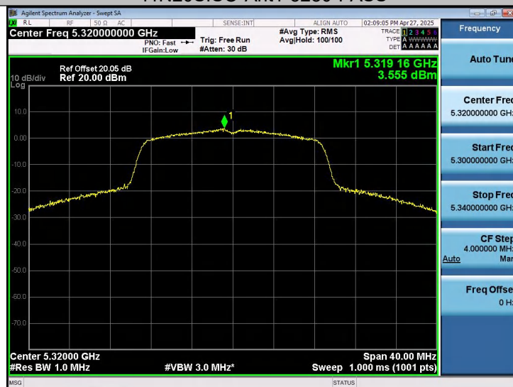
11N20SISO-Ant1-5320-PASS
