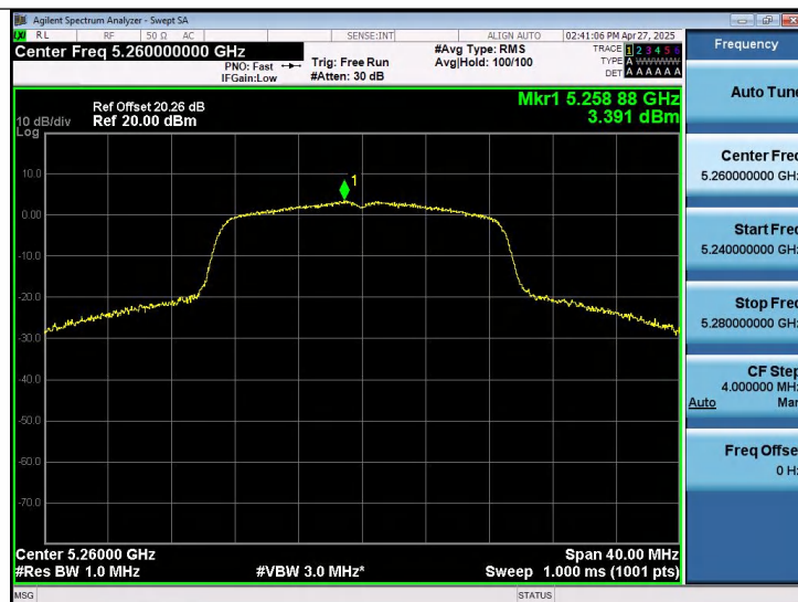
11AC20SISO-Ant1-5260-PASS
