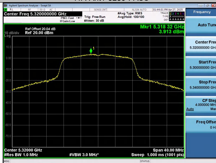
11A-Ant1-5320-PASS
