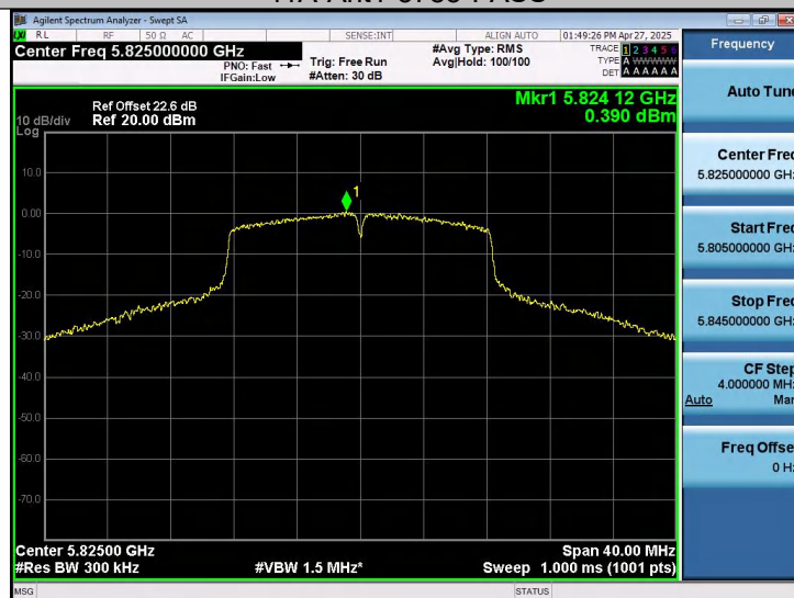
11A-Ant1-5825-PASS
