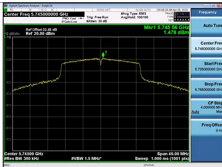
11AC20SISO-Ant1-5745-PASS
