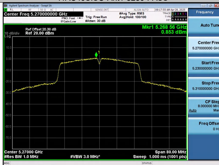
11AC40SISO-Ant1-5270-PASS
