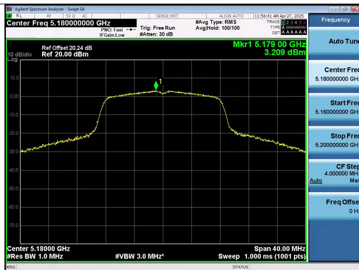
11A-Ant1-5180-PASS
