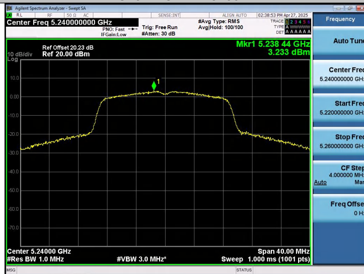
11AC20SISO-Ant1-5240-PASS
