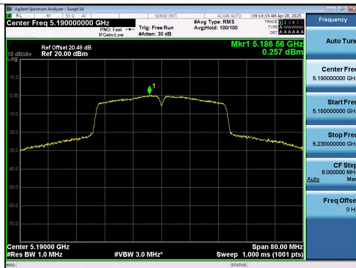
11AC40SISO-Ant1-5190-PASS
