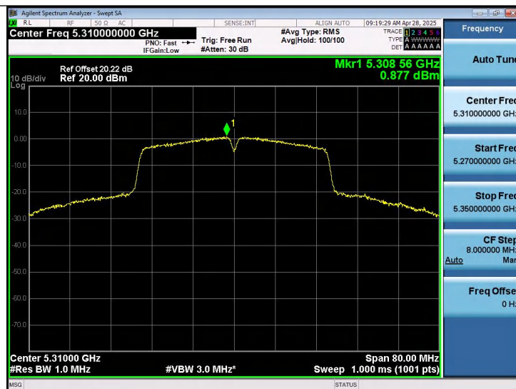
11AC40SISO-Ant1-5310-PASS
