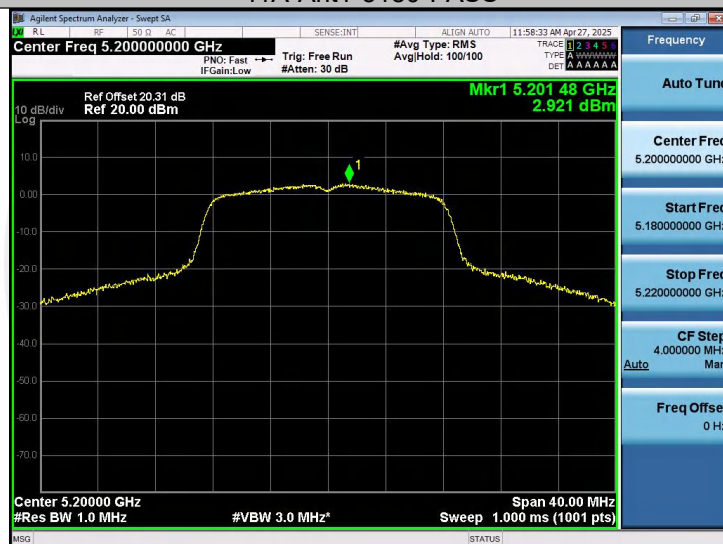
11A-Ant1-5200-PASS
