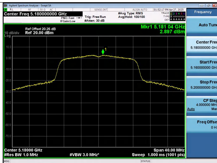
11N20SISO-Ant1-5180-PASS
