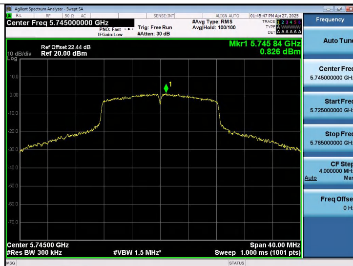
11A-Ant1-5745-PASS
