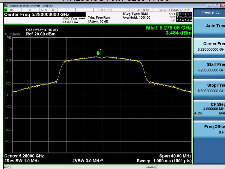
11N20SISO-Ant1-5280-PASS
