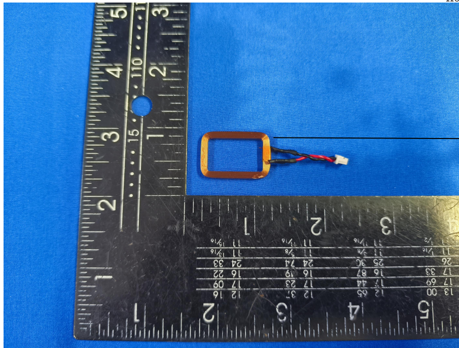
13.56MHz/125KHz Antenna
