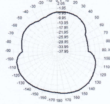
Total(H-XY), Max=-0.95dBi, CirD=10.87
