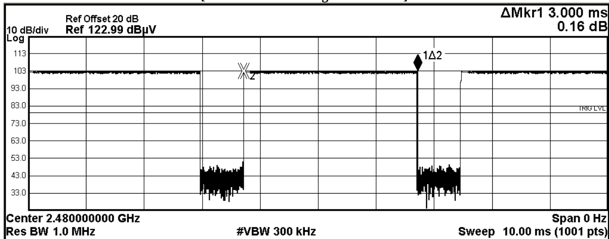
Fig. C [Pulse duration of Highest Channel]
