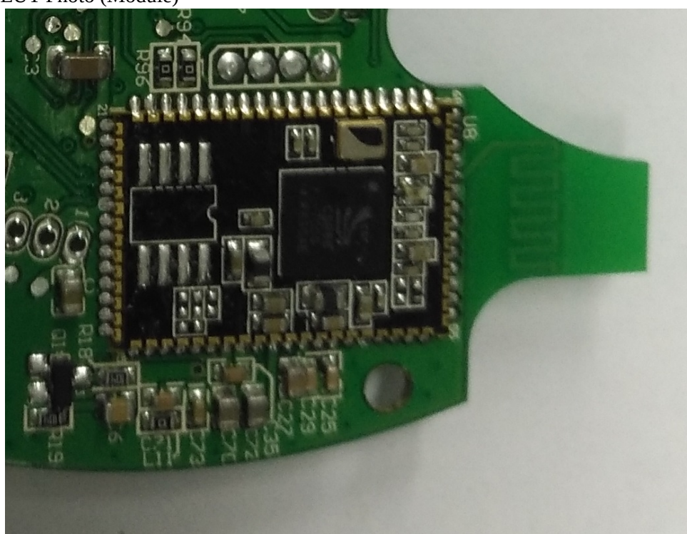
(22) EUT Photo (Module)
