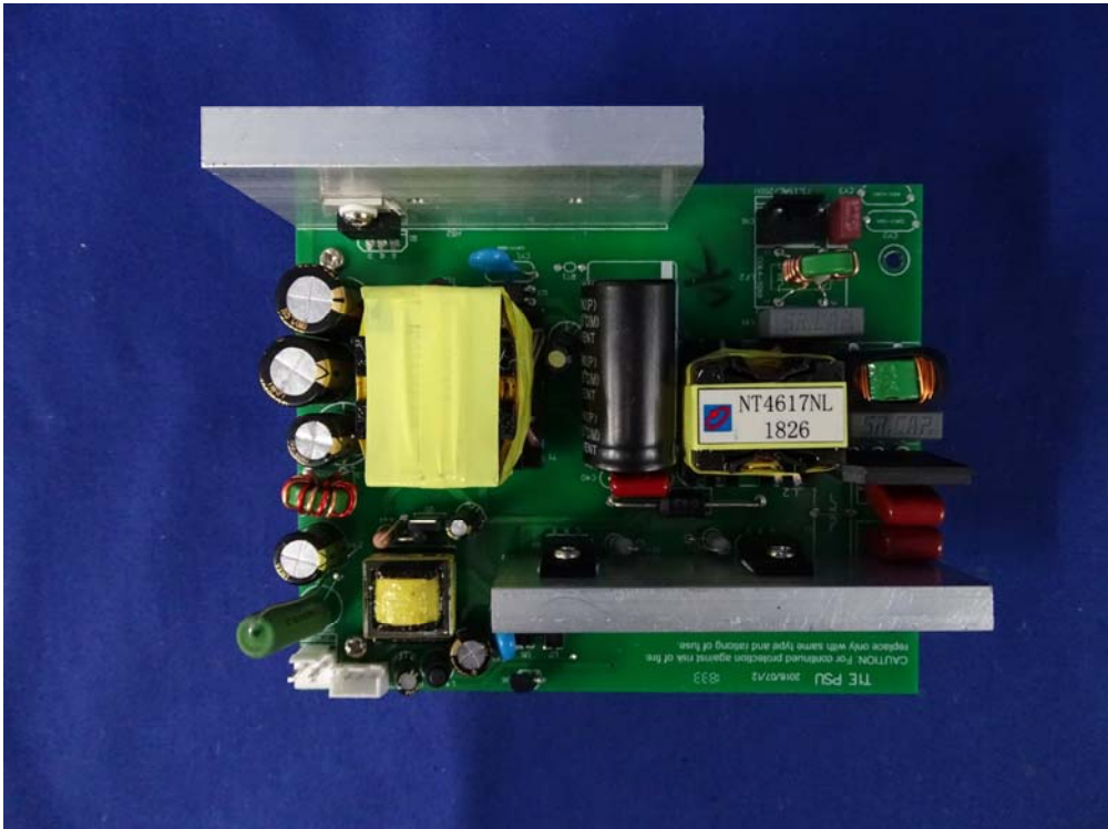
(39) EUT Photo
