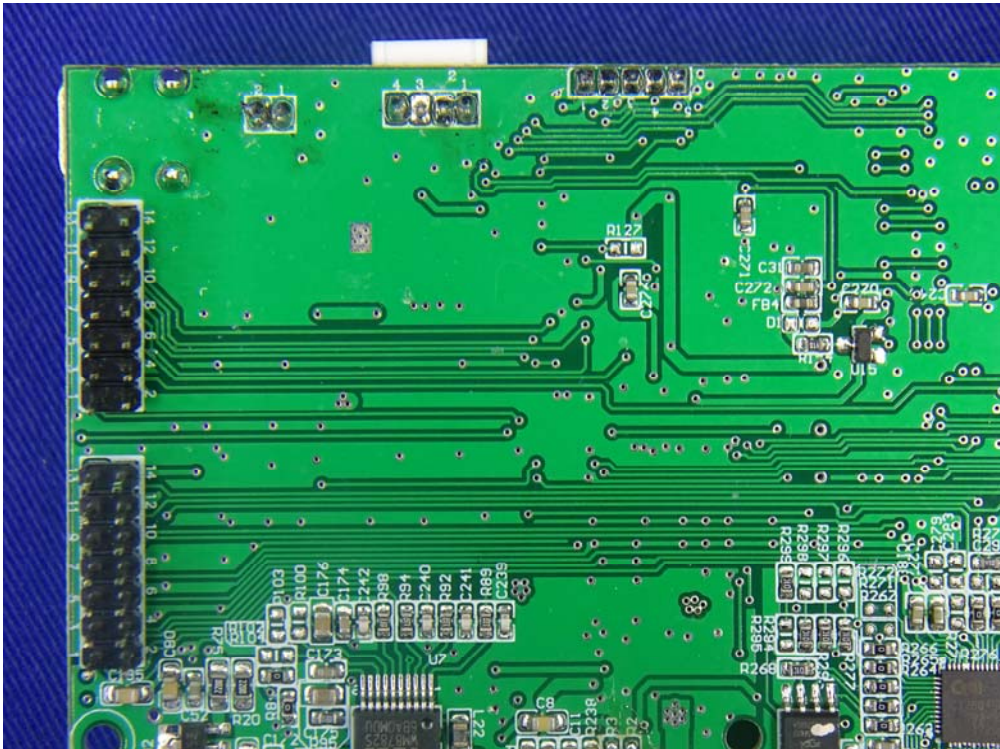
(34) EUT Photo
