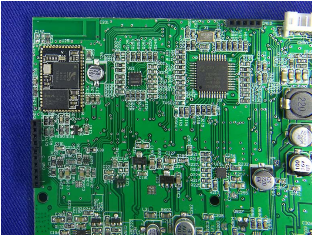
(28) EUT Photo
