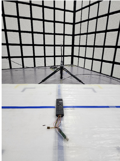
9 kHz ~ 30 MHz FACE OFF REAR TEST PHOTO
