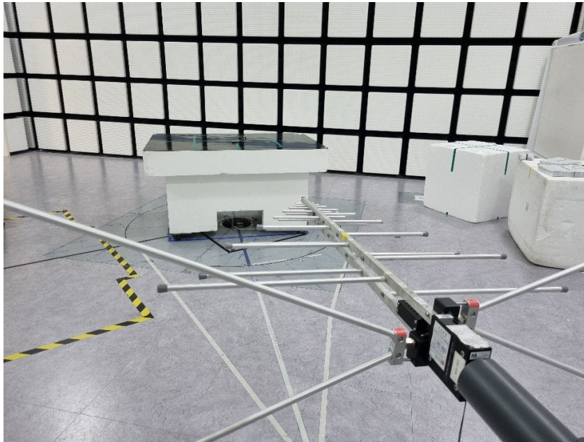
30 MHz ~ 1 GHz FRONT TEST PHOTO
