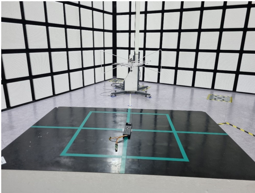
30 MHz ~ 1 GHz REAR TEST PHOTO
