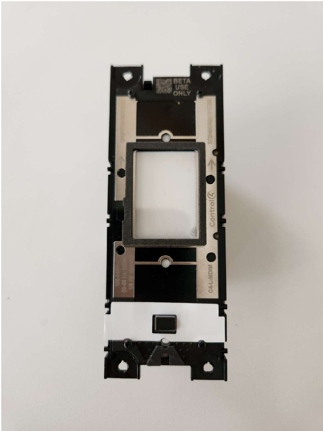
MDIM Front View (without Plastic Covers)
