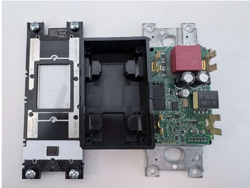
MDIM Assembly Breakdown
