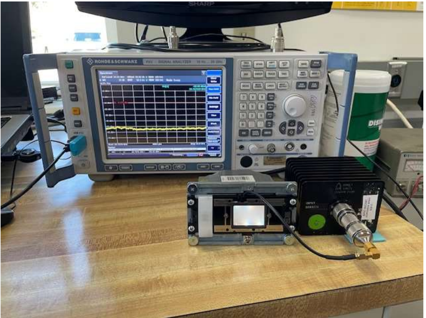
MDIM Antenna Conducted Test Setup
