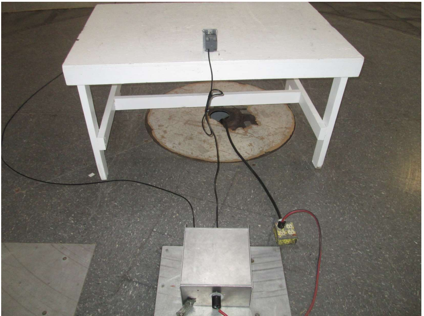
MDIM Conducted Emissions Test Setup
