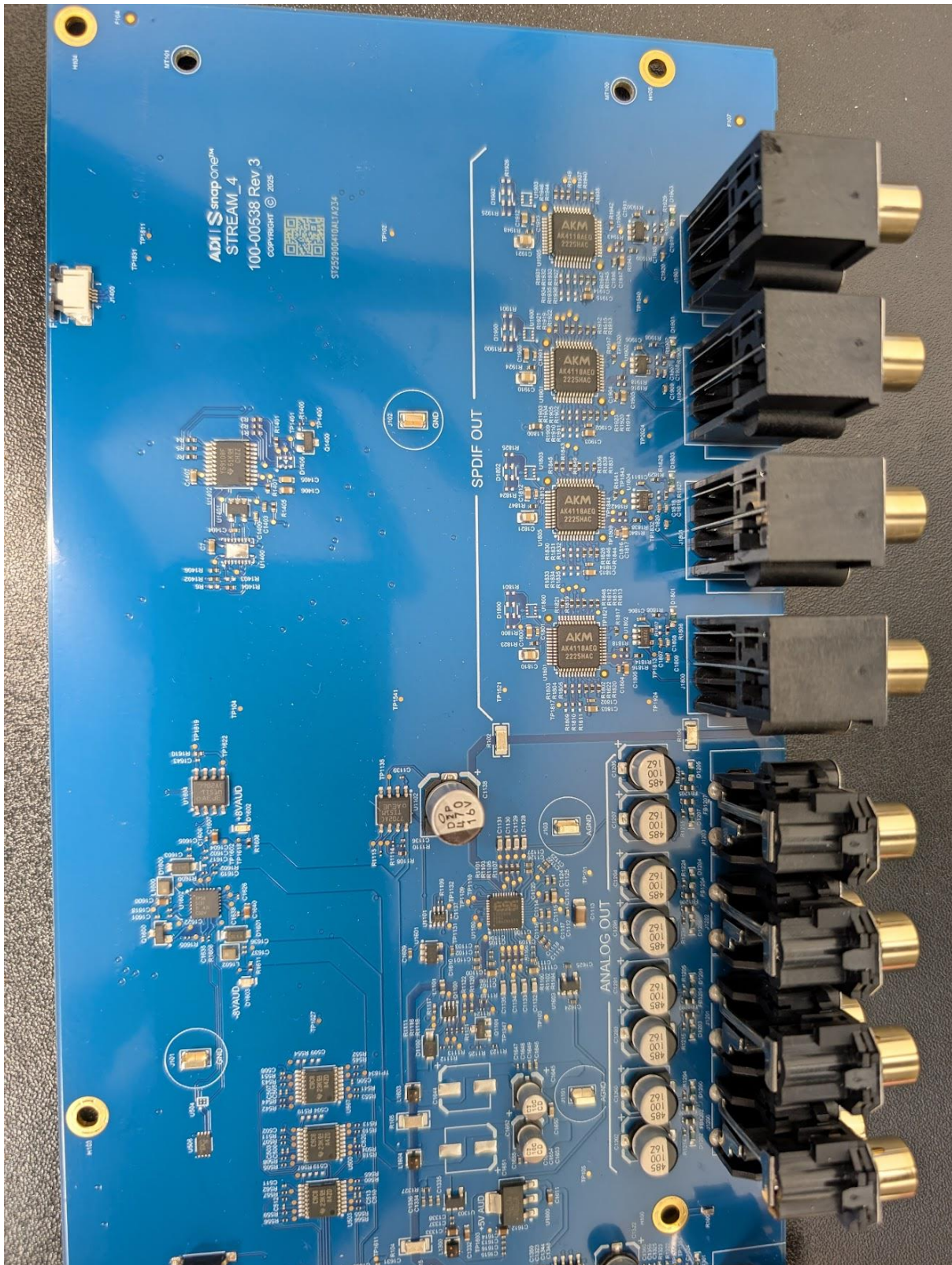
Photograph 4 – Top view of PCB, Left Side Closeup
