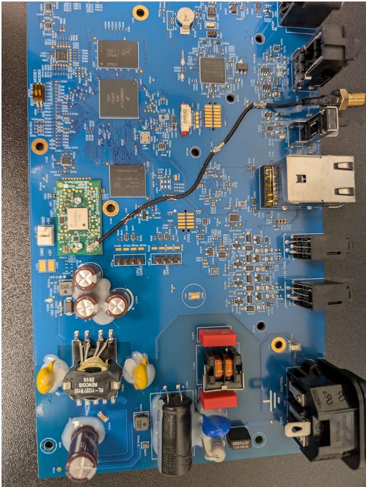
Photograph 6 – Top view of PCB, Right Side Closeup
