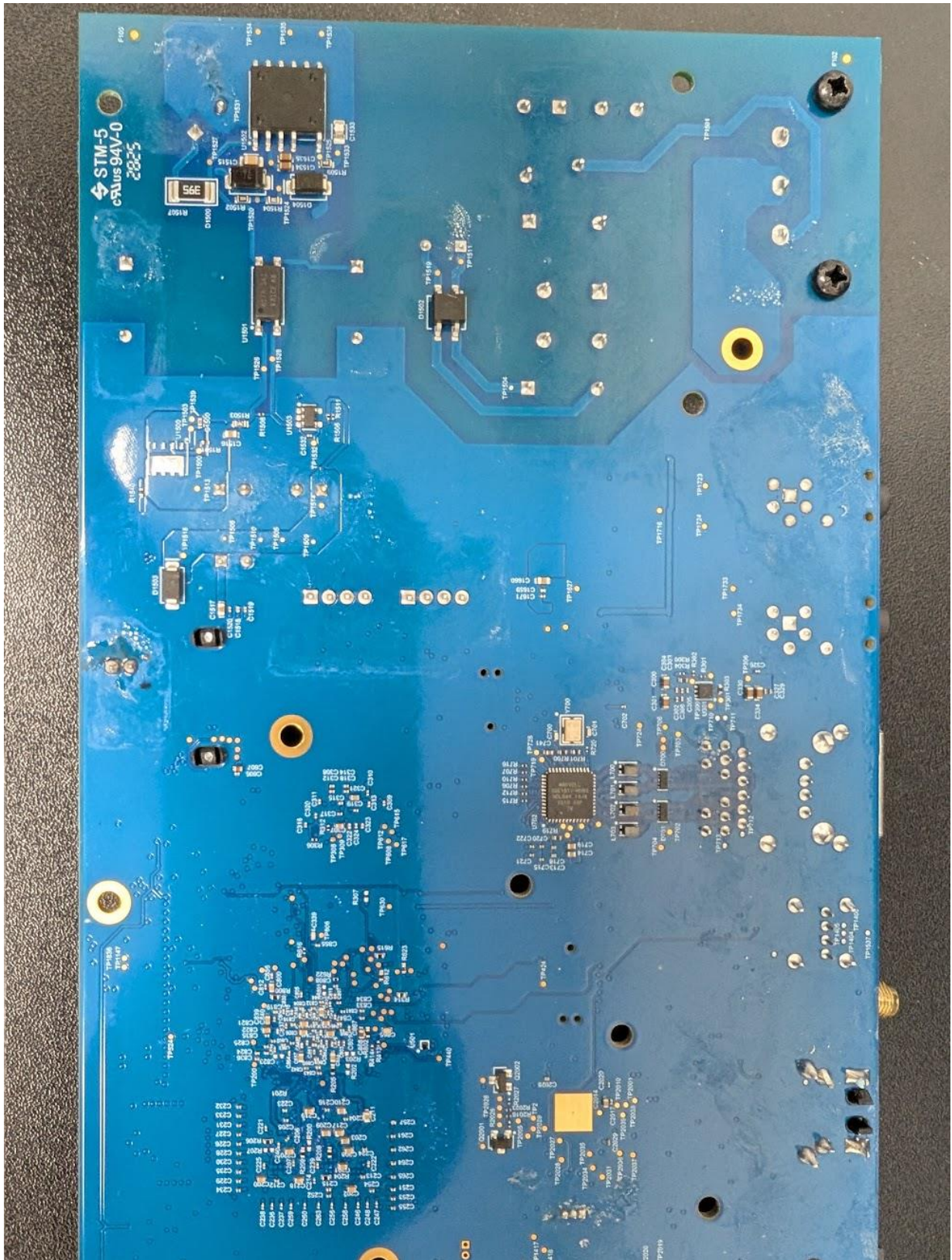
Photograph 8 – Bottom View of PCB, Left Side Closeup
