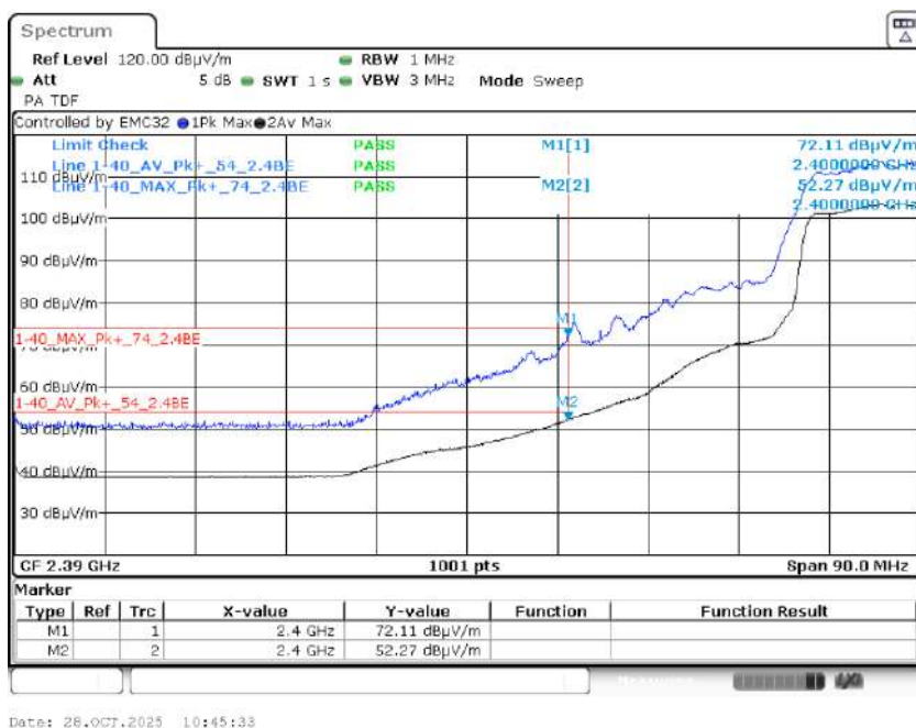
Graph 37: 2432 MHz Radiated Lower Band Edge Plot, Power Level 15
