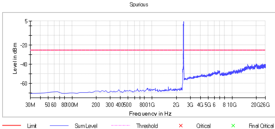
Graph 59: Transmitting on the Highest Channel, Power Level 17
