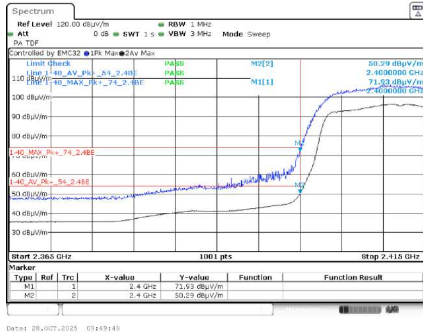
Graph 63: 2412 MHz Radiated Lower Band Edge Plot, Power Level 8
