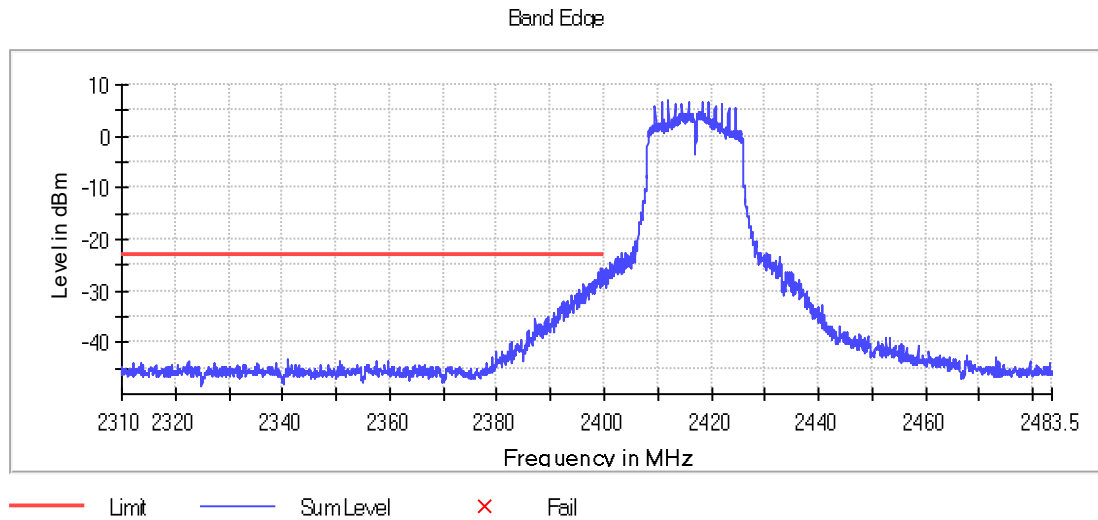
Graph 61: 2417 MHz Lower Band Edge Plot, Power Level 17
