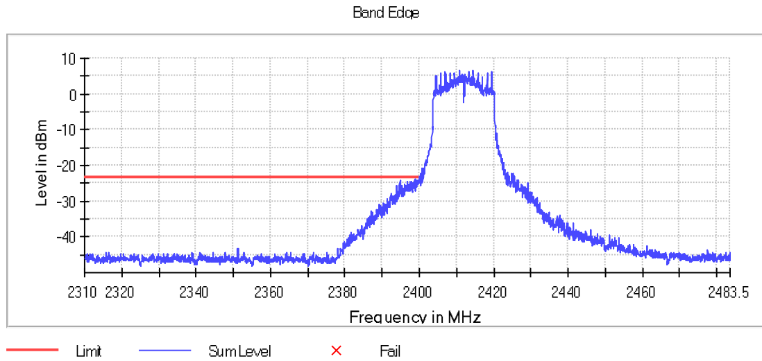
Graph 31: 2412 MHz Lower Band Edge Plot, Power Level 17
