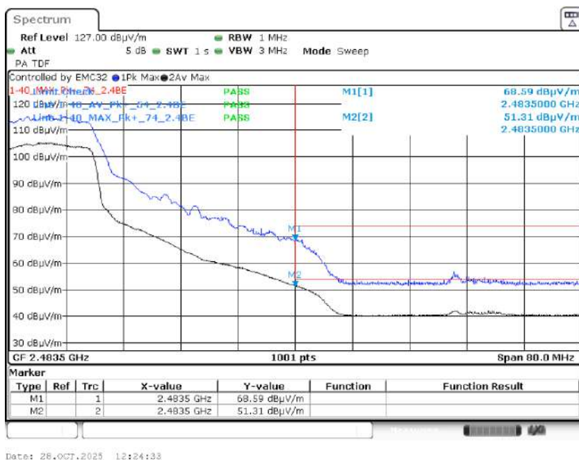
Graph 44: 2447 MHz Radiated Upper Band Edge Plot, Power Level 16
