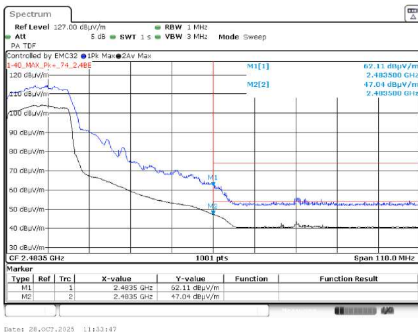
Graph 40: 2437 MHz Radiated Upper Band Edge Plot, Power Level 16
