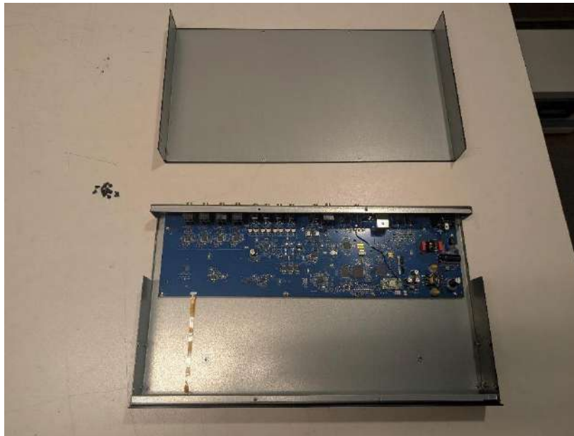
Photograph 13: View of the PCB Placement in the Enclosure
