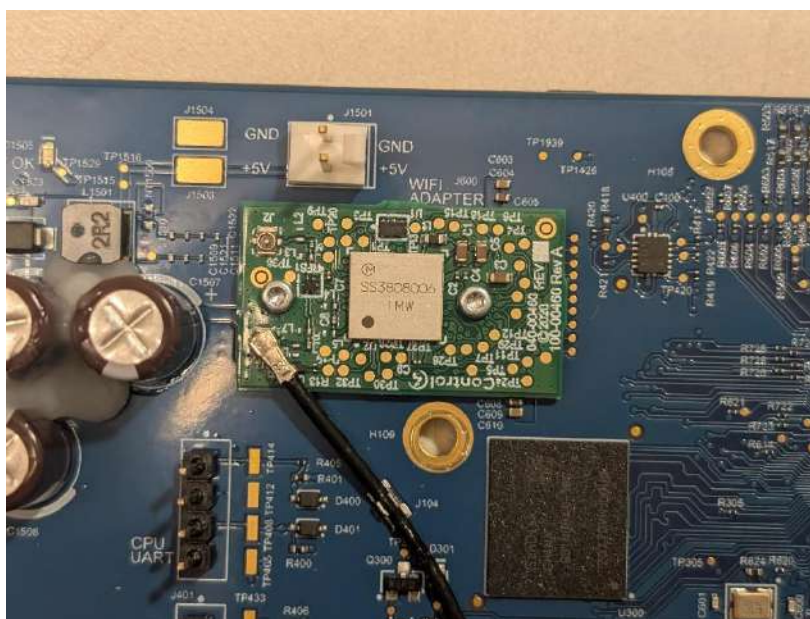
Photograph 17: Closeup View of the RF Section of the PCB Removed from Enclosure
