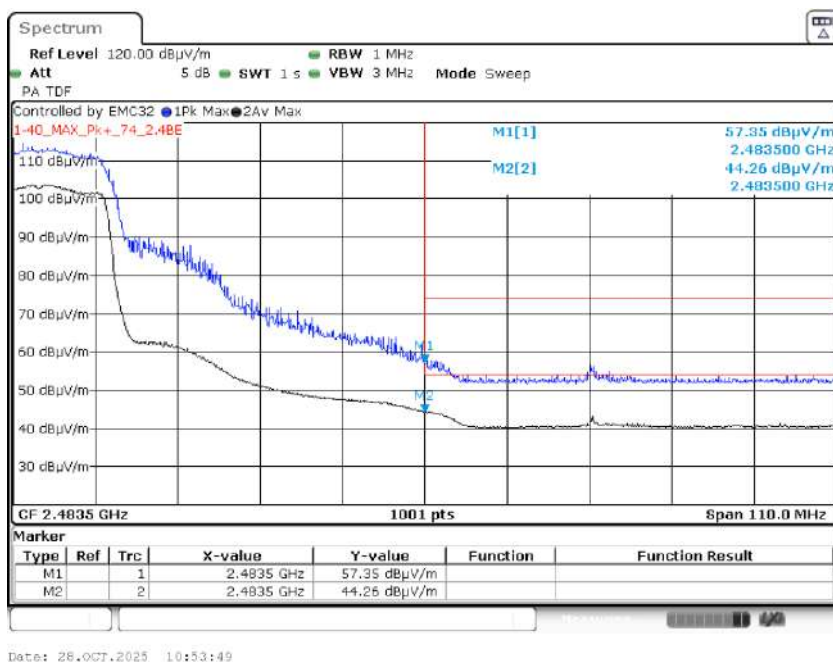
Graph 68: 2432 MHz Radiated Upper Band Edge Plot, Power Level 15
