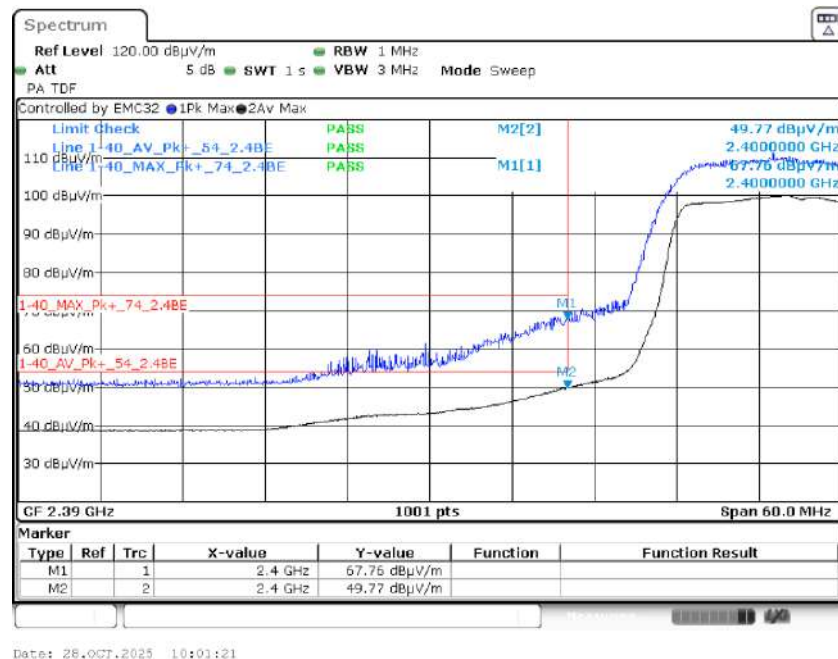
Graph 64: 2417 MHz Radiated Lower Band Edge Plot, Power Level 11
