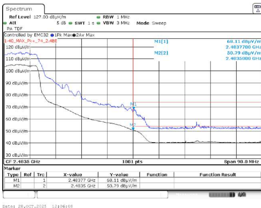
Graph 42: 2442 MHz Radiated Upper Band Edge Plot, Power Level 17
