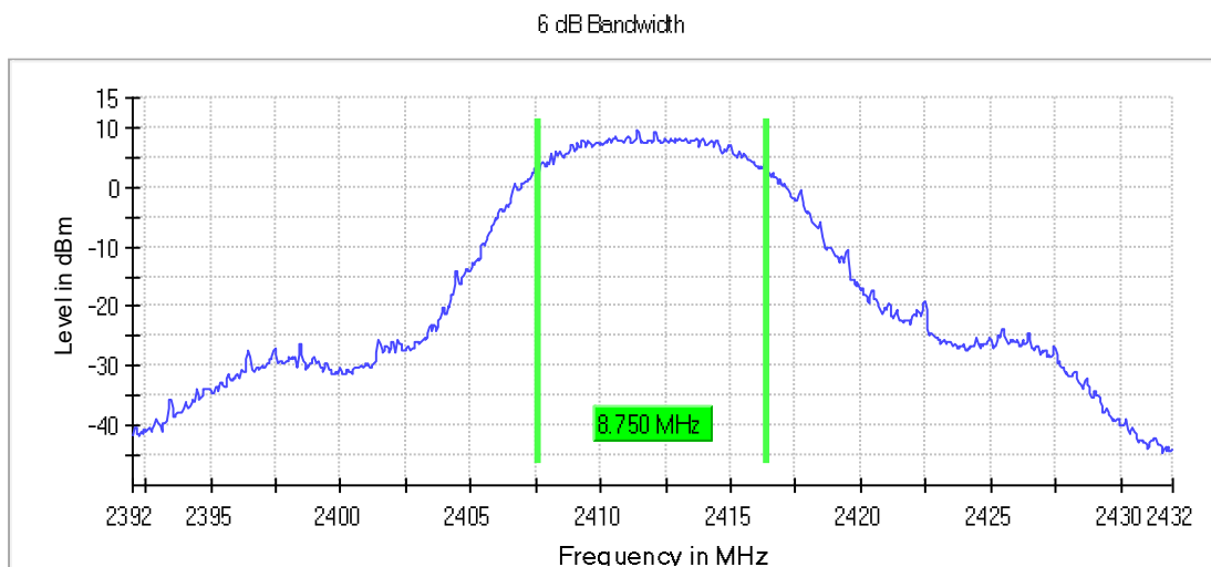
Graph 1: Lowest Channel Bandwidth
