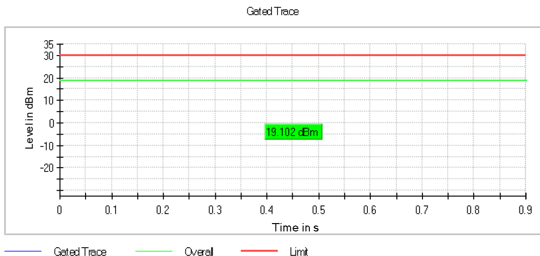
Graph 6: 2462 MHz Output Power
