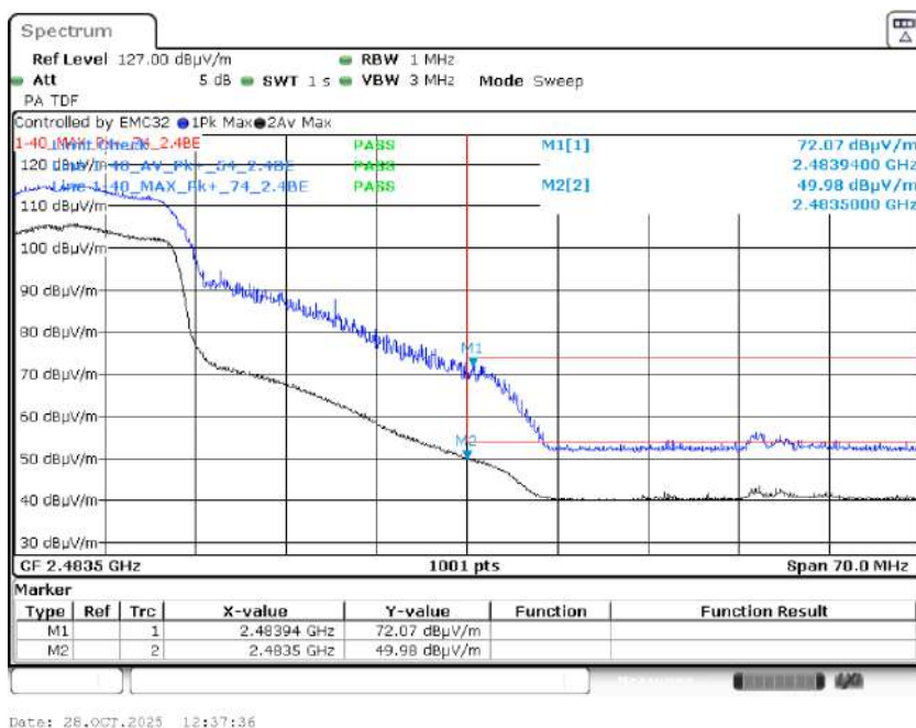
Graph 75: 2452 MHz Radiated Upper Band Edge Plot, Power Level 16
