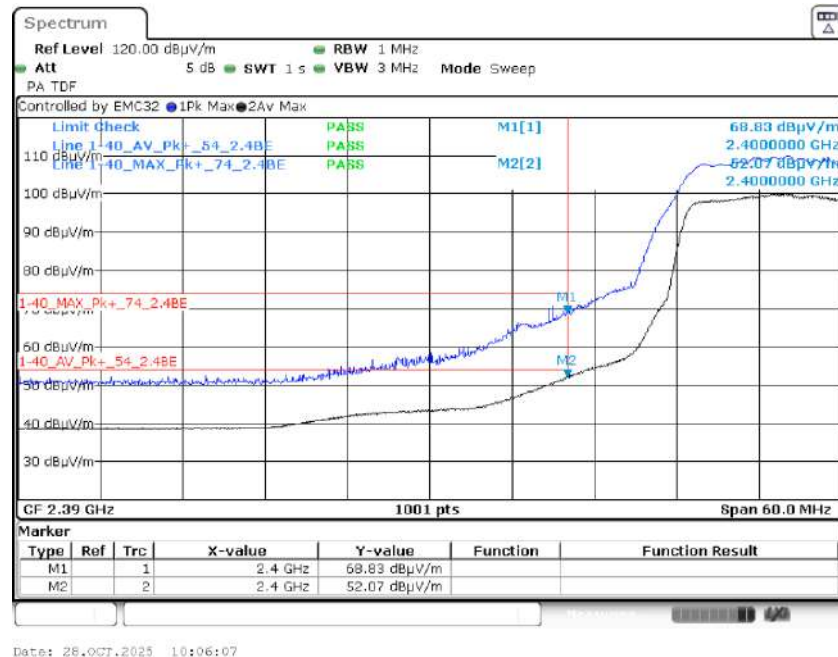
Graph 34: 2417 MHz Radiated Lower Band Edge Plot, Power Level 11
