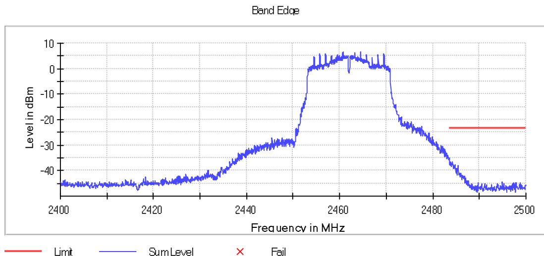
Graph 62: 2462 MHz Upper Band Edge Plot, Power Level 17
