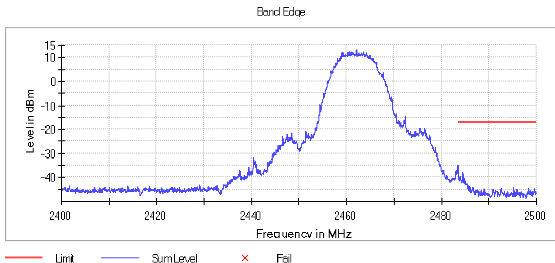
Graph 11: 2462 MHz Upper Band Edge Plot, Power Level 20
