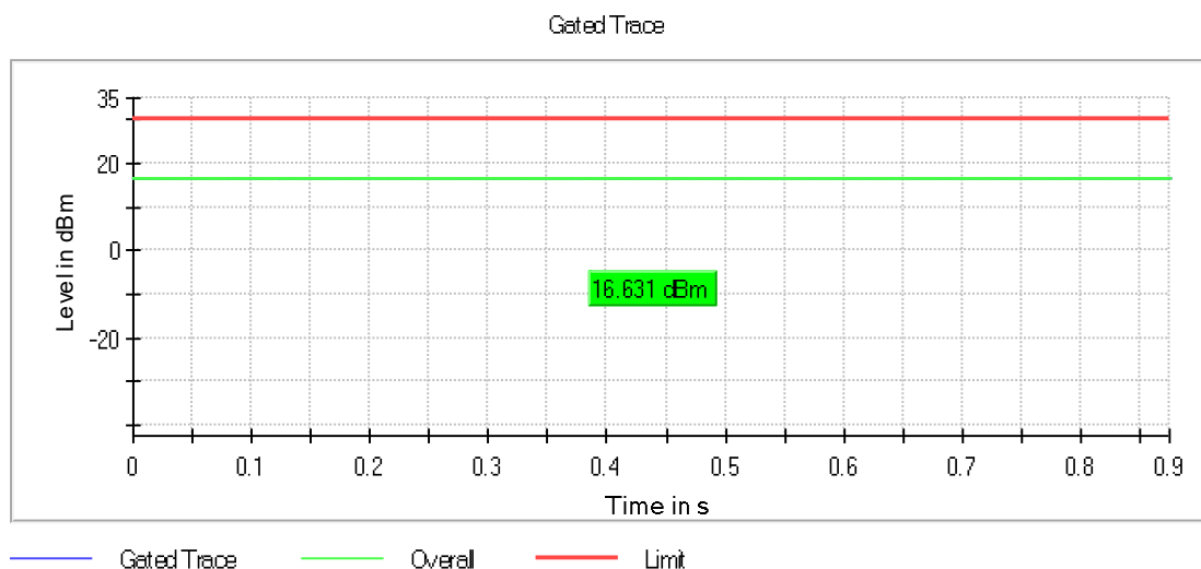
Graph 27: 2462 MHz Output Power
