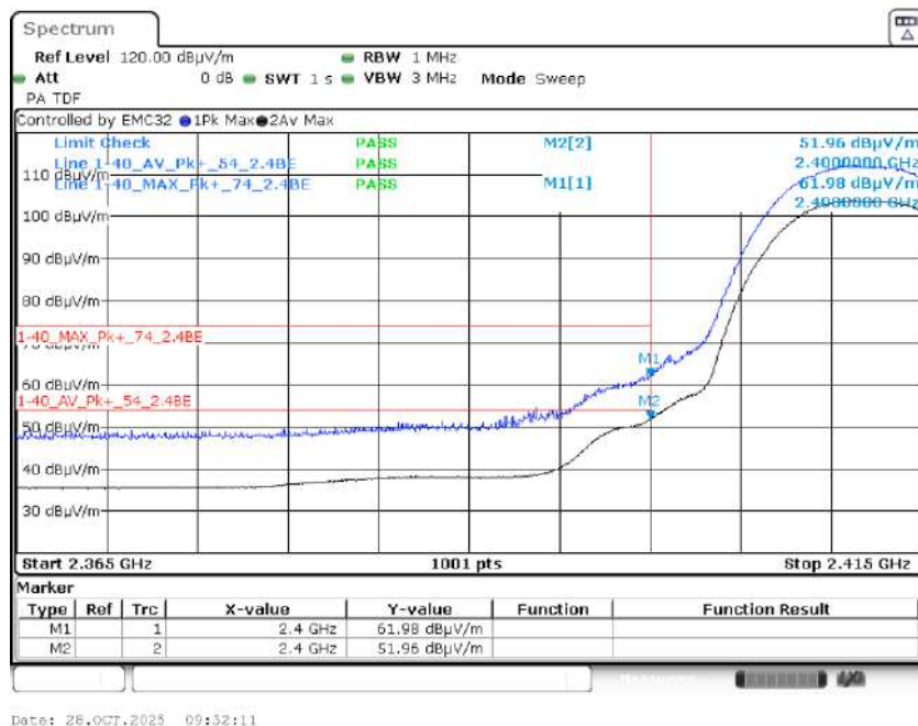
Graph 12: 2412 MHz Radiated Lower Band Edge Plot, Power Level 13
