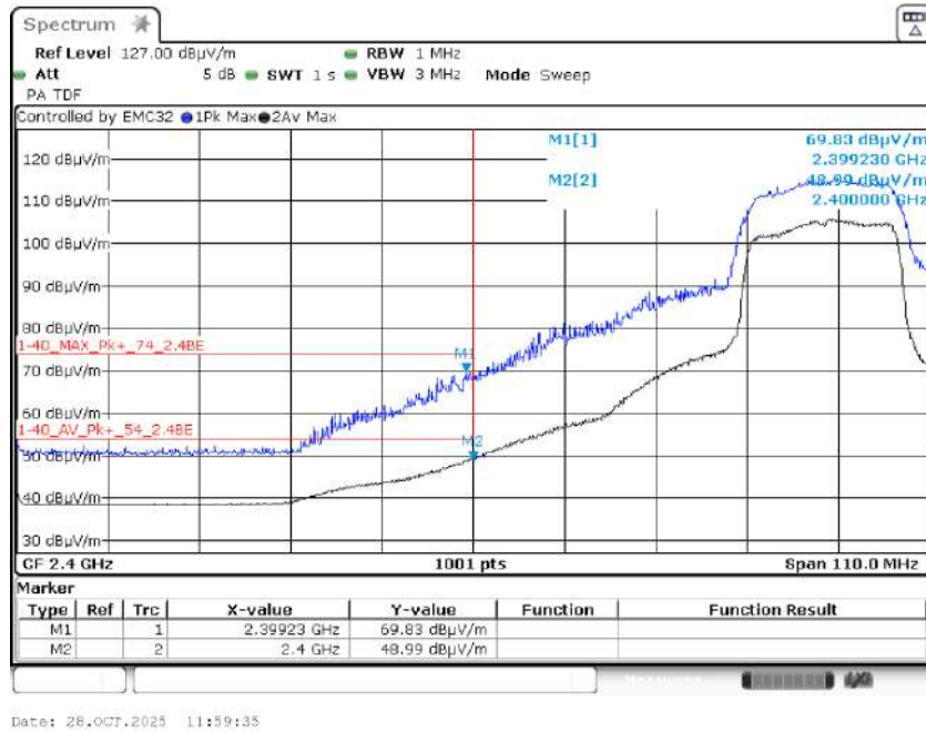
Graph 71: 2442 MHz Radiated Lower Band Edge Plot, Power Level 17
