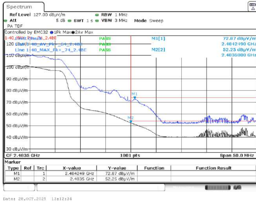
Graph 47: 2462 MHz Radiated Upper Band Edge Plot, Power Level 12
