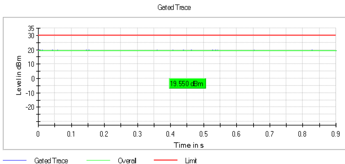
Graph 4: 2412 MHz Output Power
