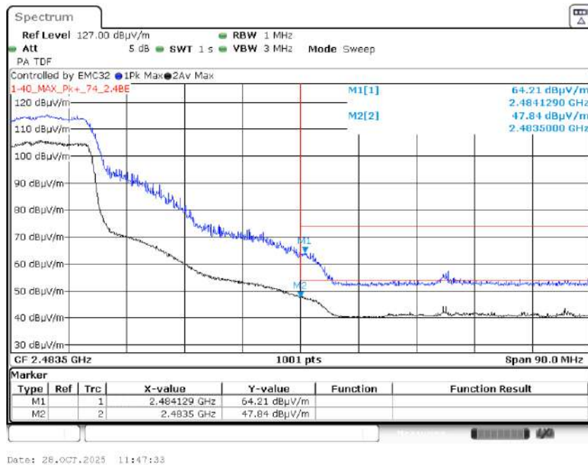
Graph 72: 2442 MHz Radiated Upper Band Edge Plot, Power Level 17
