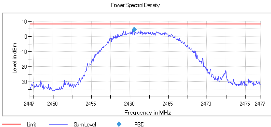
Graph 21: 2462 MHz Output 100 kHz PSD Plot
