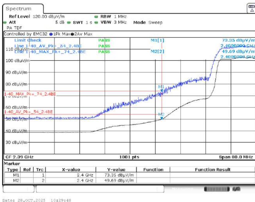
Graph 66: 2427 MHz Radiated Lower Band Edge Plot, Power Level 14
