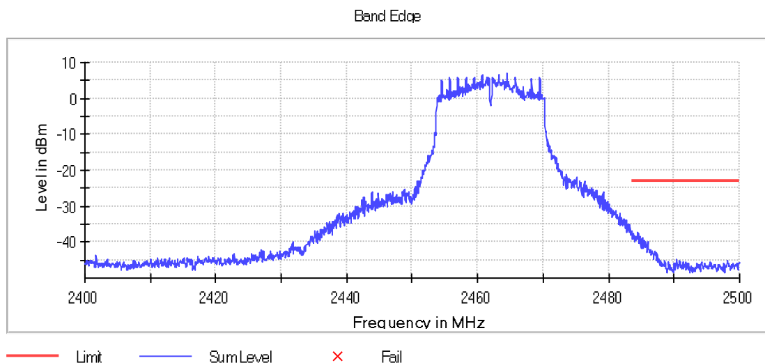
Graph 32: 2462 MHz Upper Band Edge Plot, Power Level 17
