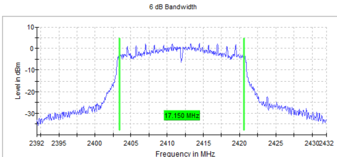
Graph 51: Lowest Channel Bandwidth
