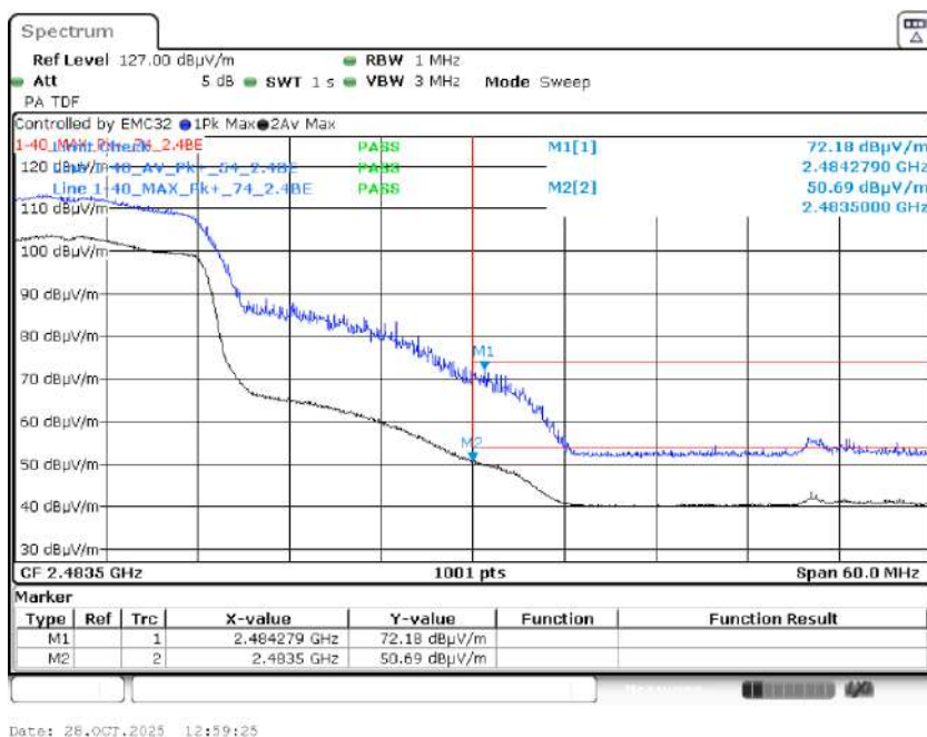
Graph 76: 2457 MHz Radiated Upper Band Edge Plot, Power Level 14
