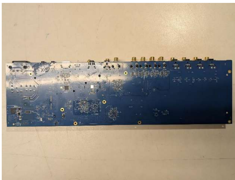
Photograph 18: Back View of the PCB Removed from Enclosure
