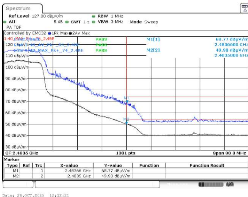
Graph 74: 2447 MHz Radiated Upper Band Edge Plot, Power Level 17
