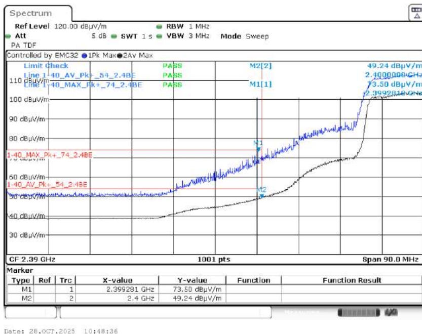
Graph 67: 2432 MHz Radiated Lower Band Edge Plot, Power Level 15
