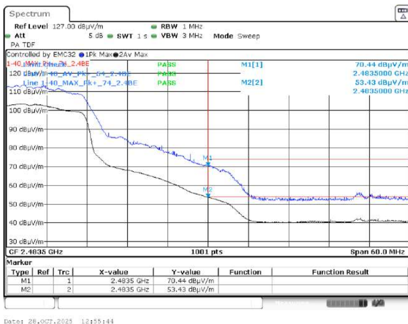
Graph 46: 2457 MHz Radiated Upper Band Edge Plot, Power Level 14
