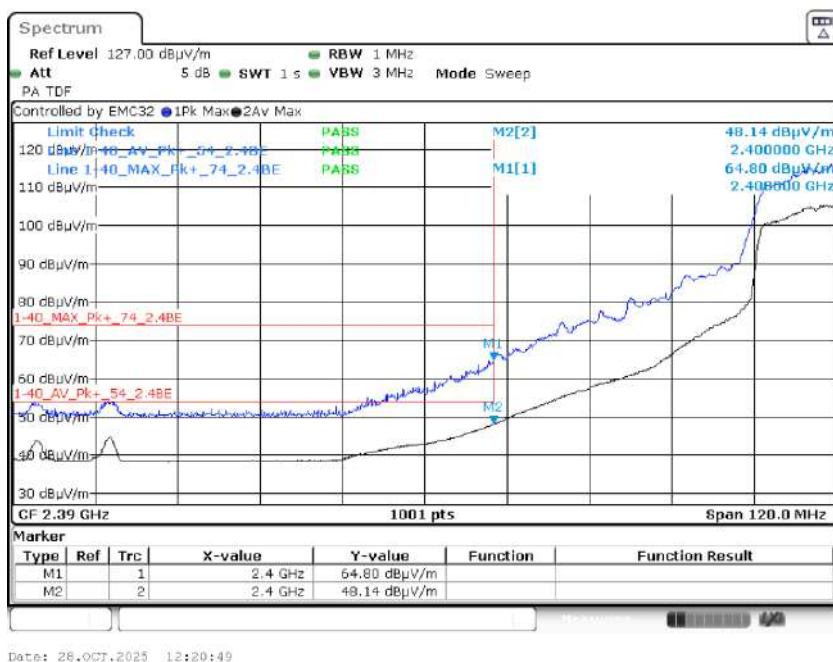
Graph 43: 2447 MHz Radiated Lower Band Edge Plot, Power Level 16
