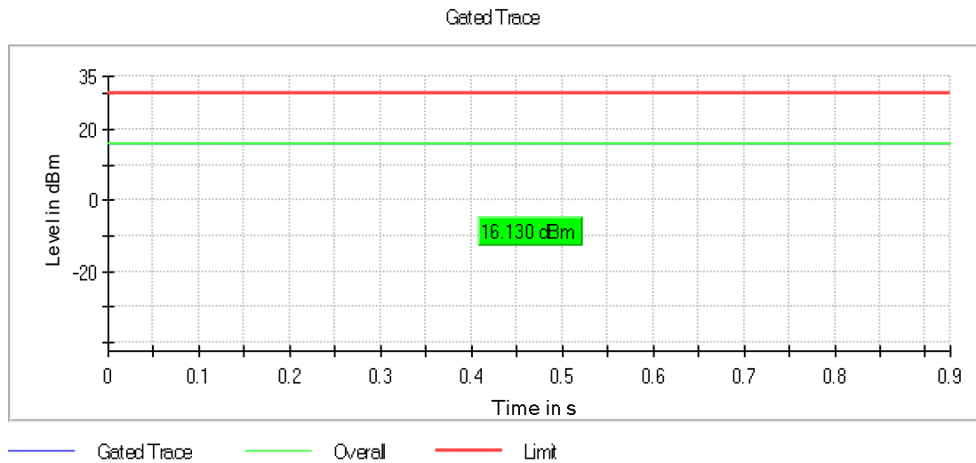
Graph 54: 2412 MHz Output Power
