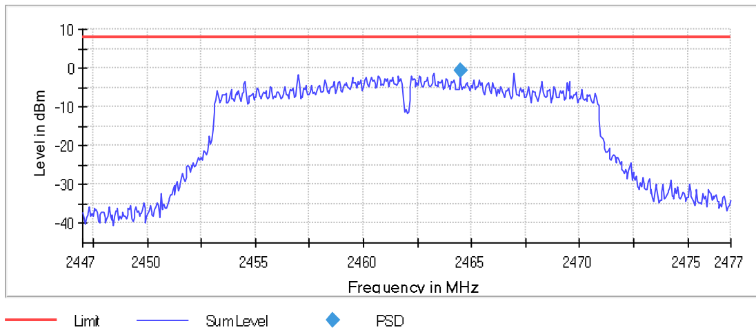
Graph 80: 2462 MHz 100 kHz PSD Plot
