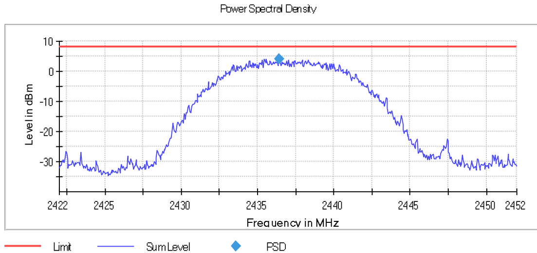
Graph 20: 2437 MHz Output 100 kHz PSD Plot
