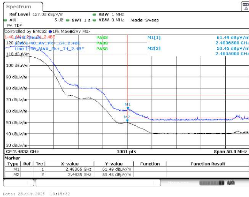
Graph 18: 2462 MHz Radiated Upper Band Edge Plot, Power Level 18
