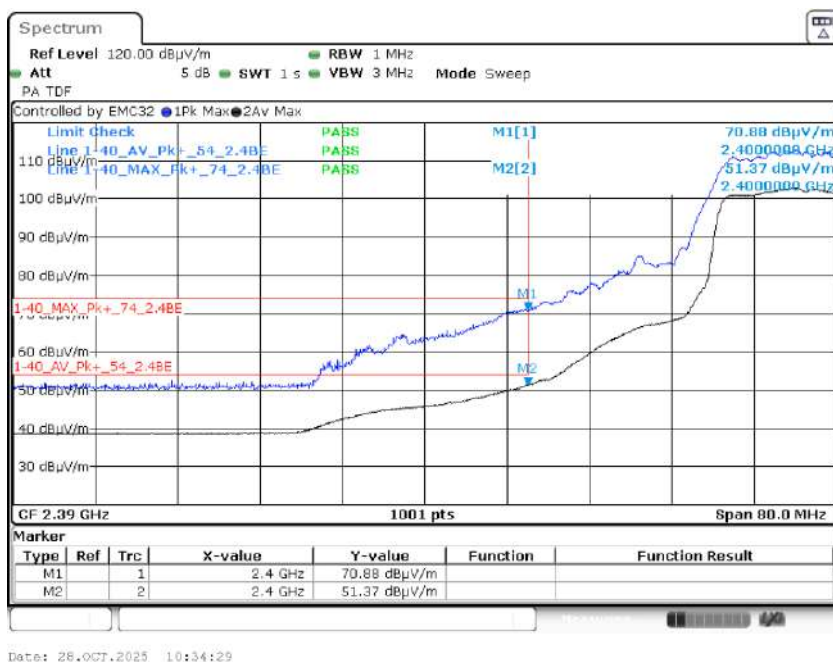
Graph 36: 2427 MHz Radiated Lower Band Edge Plot, Power Level 14
