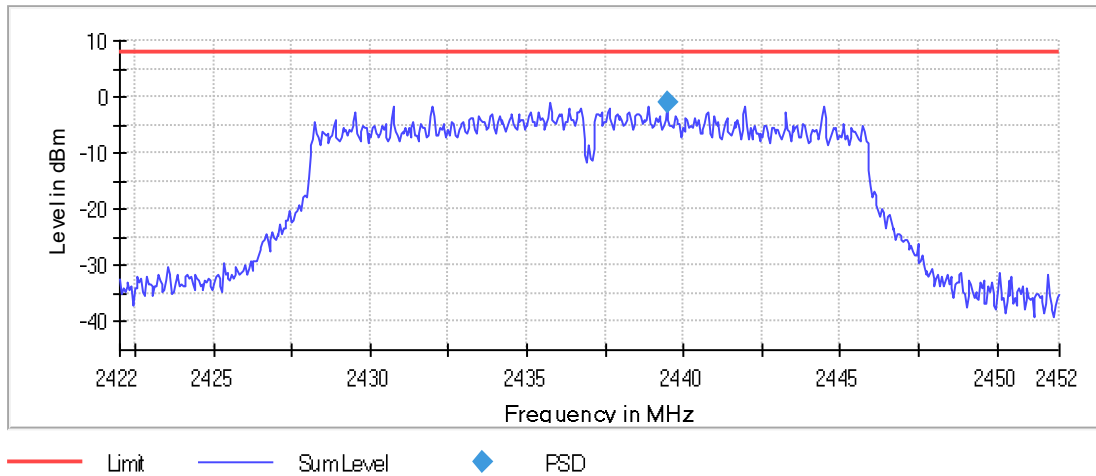
Graph 79: 2437 MHz 100 kHz PSD Plot
