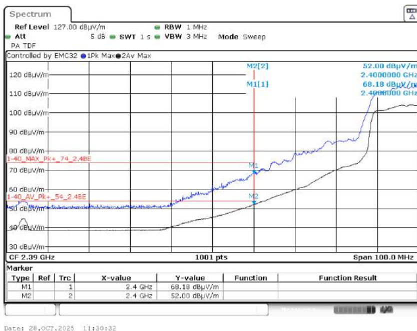
Graph 39: 2437 MHz Radiated Lower Band Edge Plot, Power Level 16
