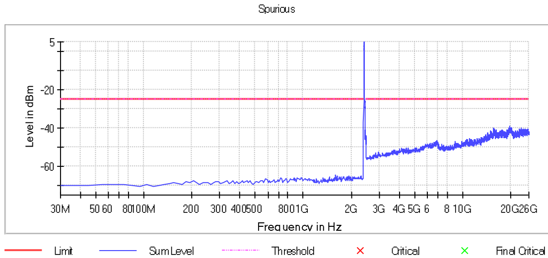
Graph 57: Transmitting on the Lowest Channel, Power Level 17
