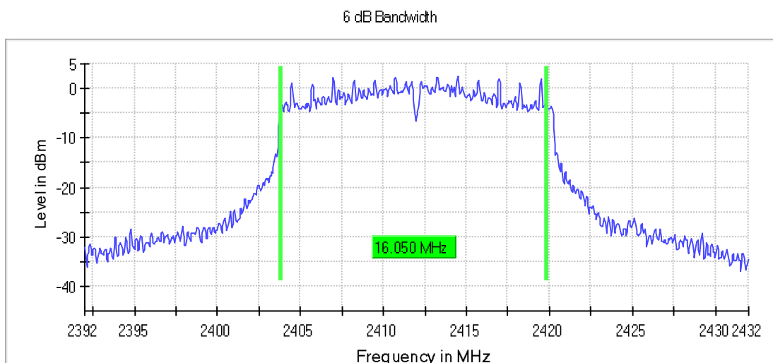
Graph 22: Lowest Channel Bandwidth
