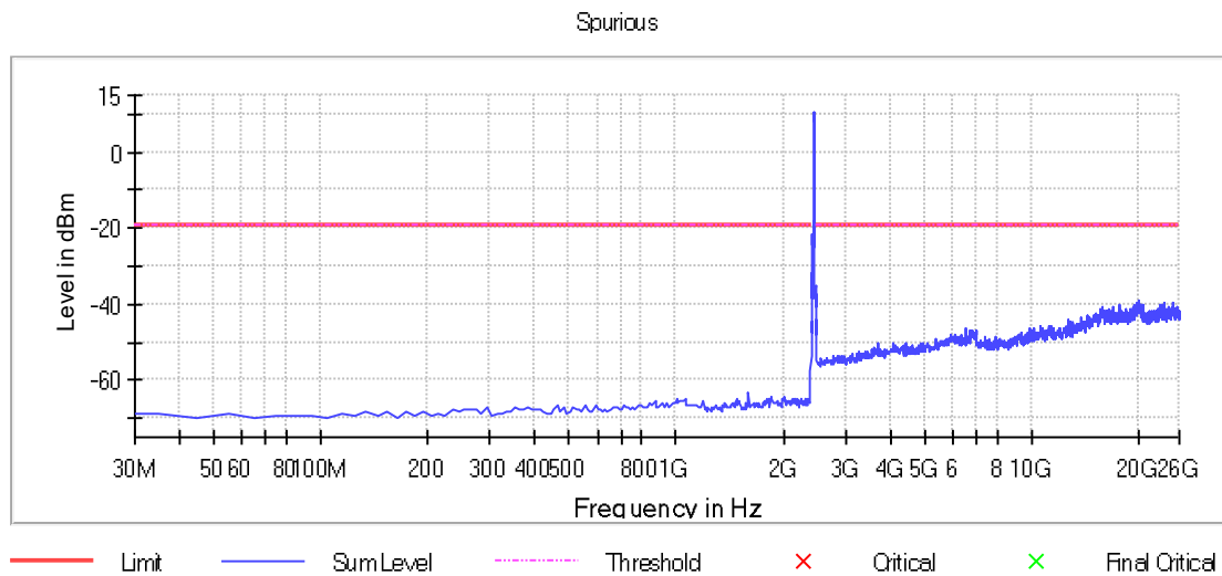
Graph 8: Transmitting on the Middle Channel, Power Level 20
