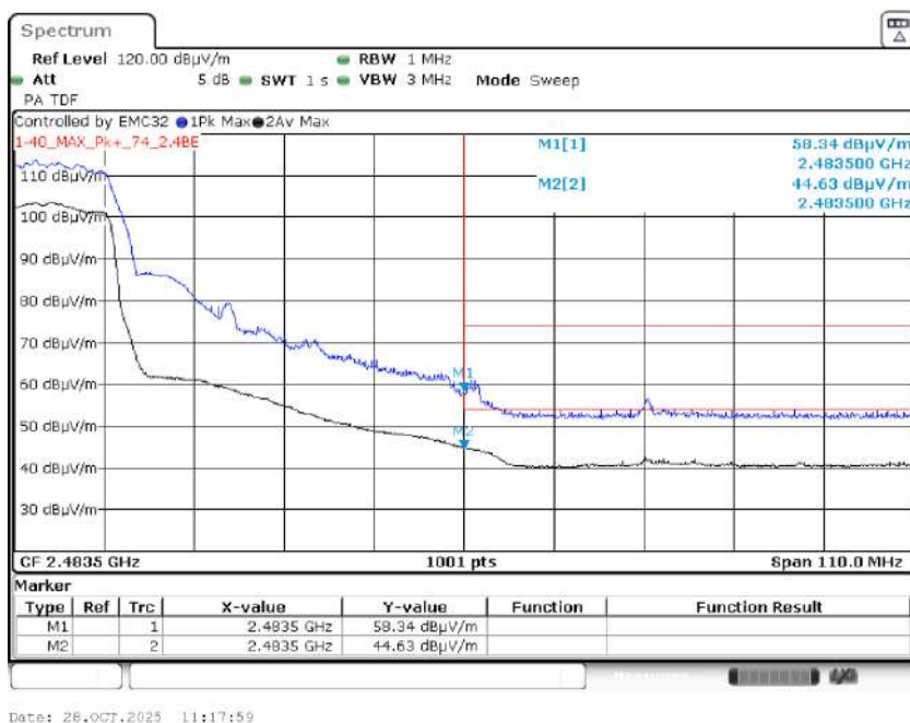
Graph 38: 2432 MHz Radiated Upper Band Edge Plot, Power Level 15
