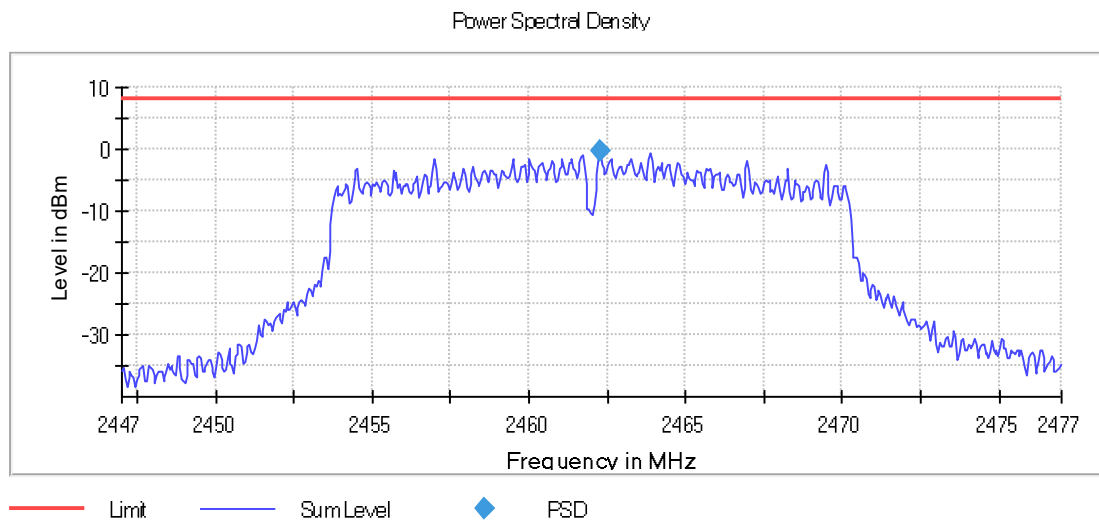
Graph 50: 2462 MHz Output 100 kHz PSD Plot
