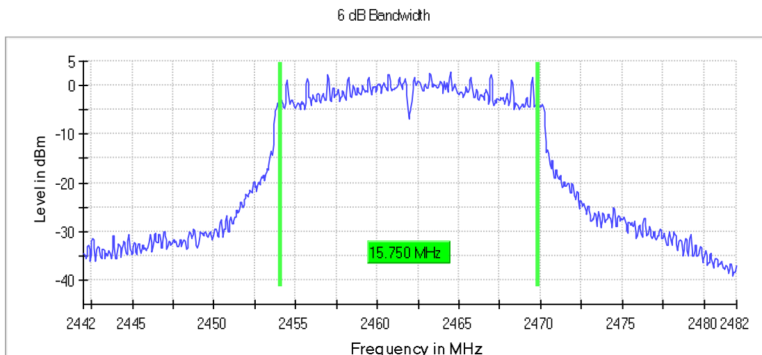
Graph 24: Highest Channel Bandwidth
