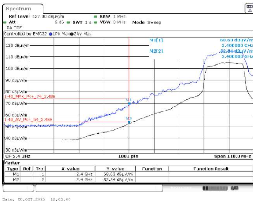
Graph 41: 2442 MHz Radiated Lower Band Edge Plot, Power Level 17
