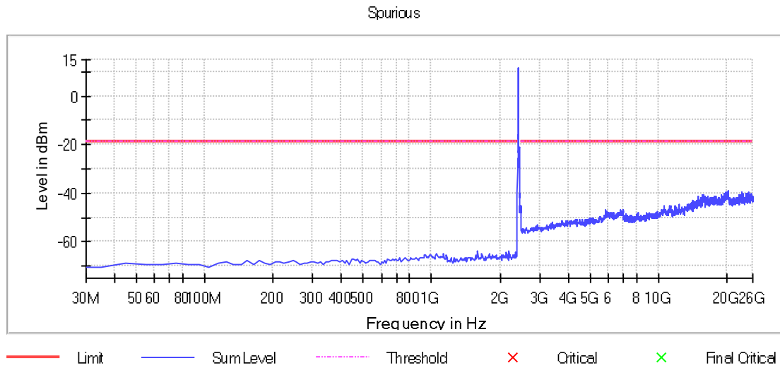
Graph 7: Transmitting on the Lowest Channel, Power Level 20
