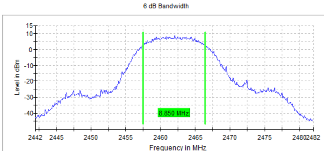
Graph 3: Highest Channel Bandwidth
