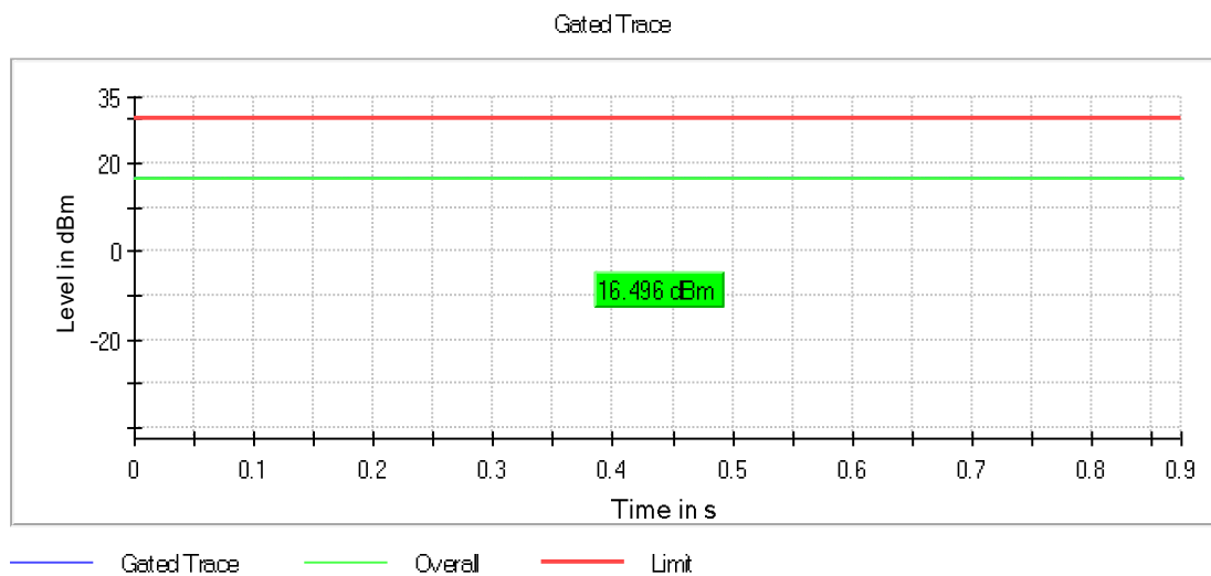
Graph 26: 2437 MHz Output Power
