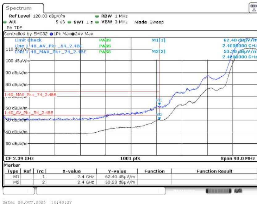
Graph 16: 2432 MHz Radiated Lower Band Edge Plot, Power Level 20
