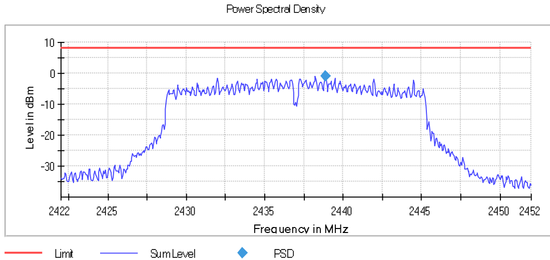
Graph 49: 2437 MHz Output 100 kHz PSD Plot
