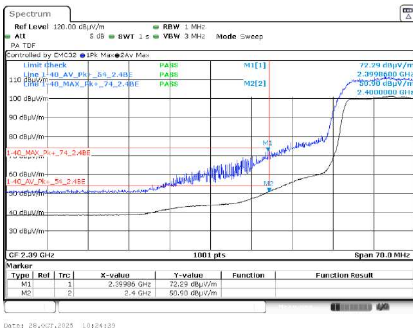
Graph 65: 2422 MHz Radiated Lower Band Edge Plot, Power Level 12
