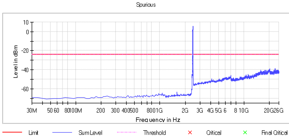
Graph 30: Transmitting on the Highest Channel, Power Level 17
