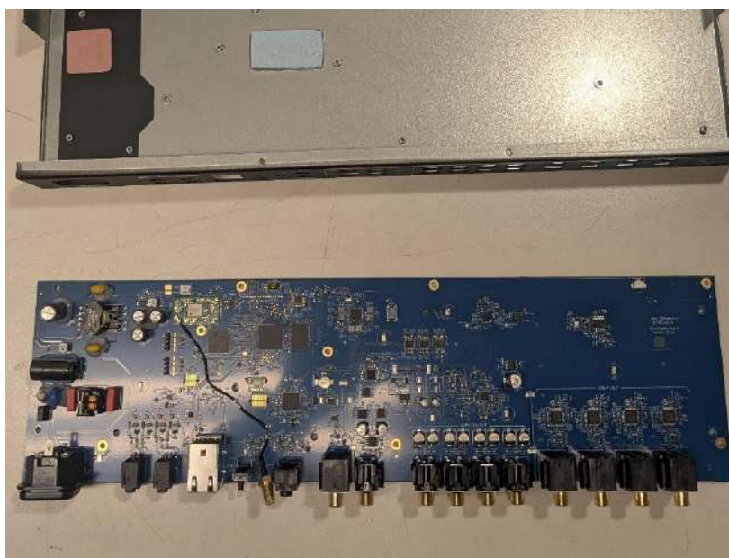
Photograph 16: Front View of the PCB Removed from Enclosure
