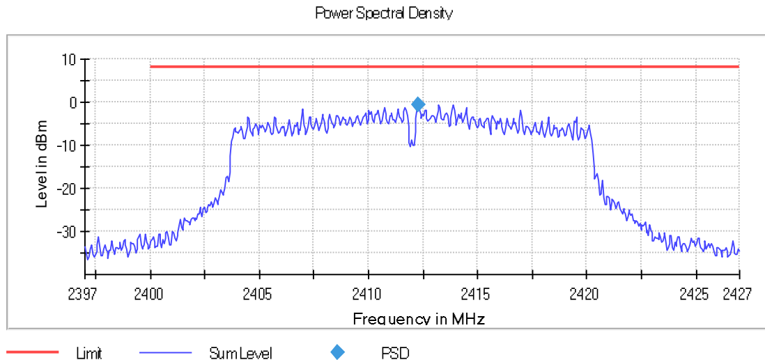
Graph 48: 2412 MHz 100 kHz PSD Plot
