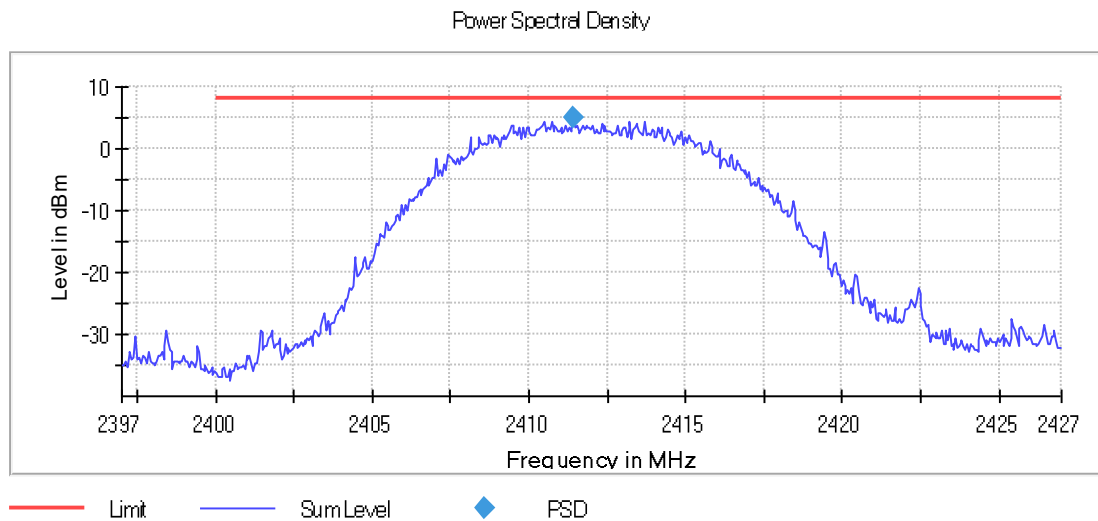
Graph 19: 2412 MHz 100 kHz PSD Plot
