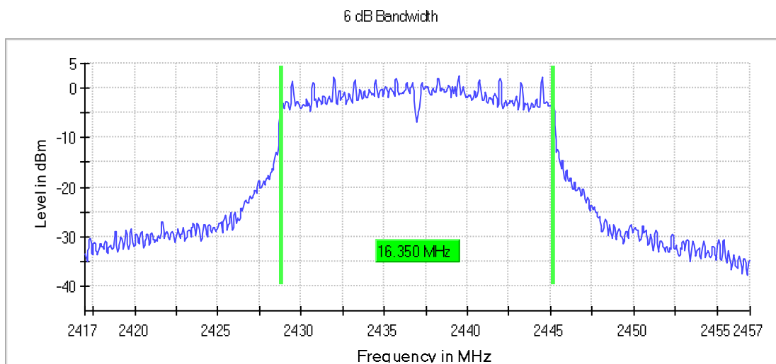
Graph 23: Middle Channel Bandwidth
