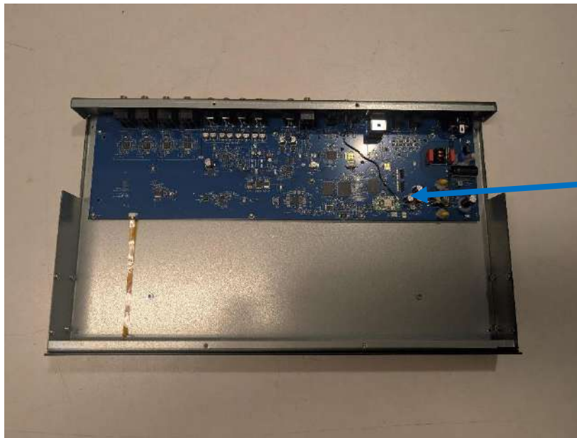
Photograph 14: Closeup View of the PCB Placement in the Enclosure
