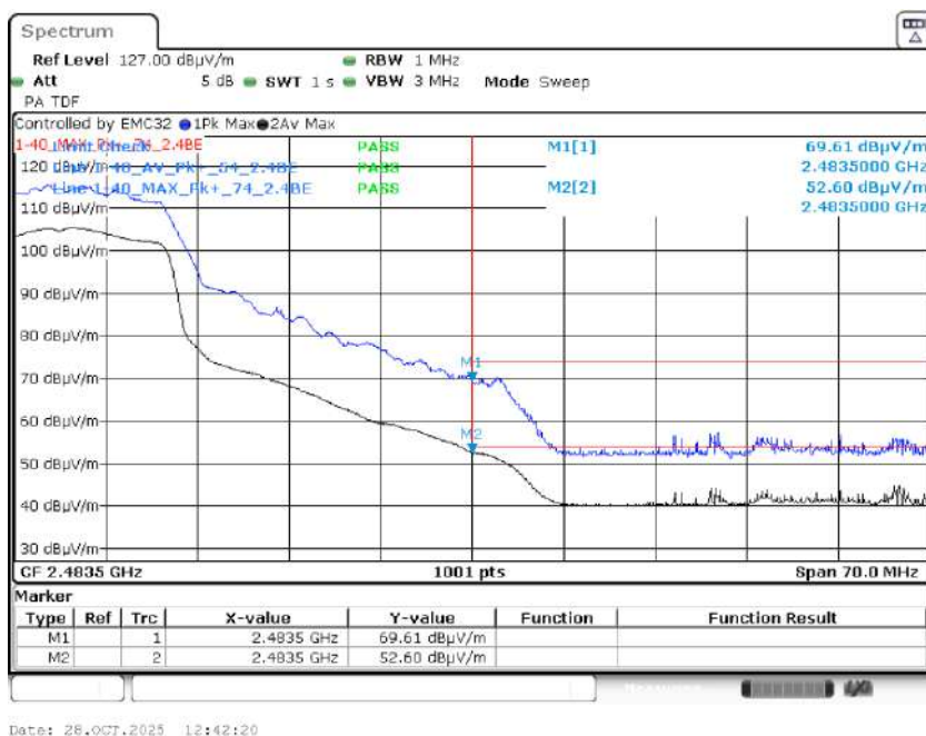
Graph 45: 2452 MHz Radiated Upper Band Edge Plot, Power Level 16
