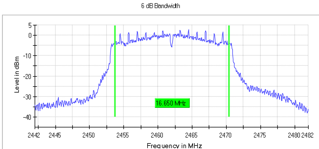
Graph 53: Highest Channel Bandwidth
