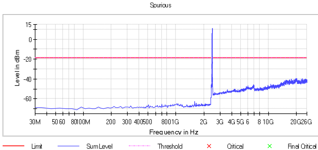
Graph 9: Transmitting on the Highest Channel, Power Level 20
