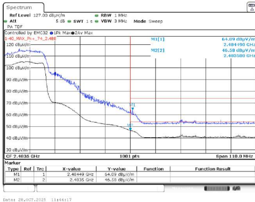
Graph 70: 2437 MHz Radiated Upper Band Edge Plot, Power Level 17
