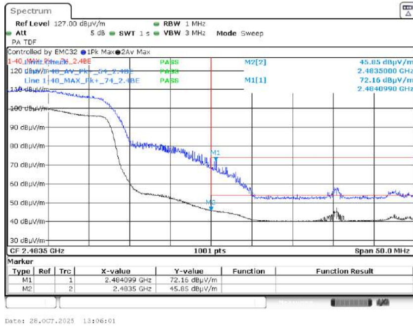
Graph 77: 2462 MHz Radiated Upper Band Edge Plot, Power Level 11
