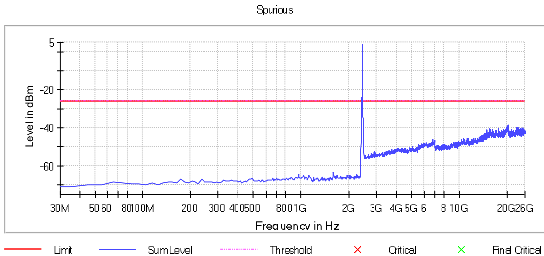
Graph 58: Transmitting on the Middle Channel, Power Level 17
