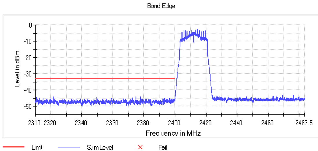
Graph 60: 2412 MHz Lower Band Edge Plot, Power Level 8
