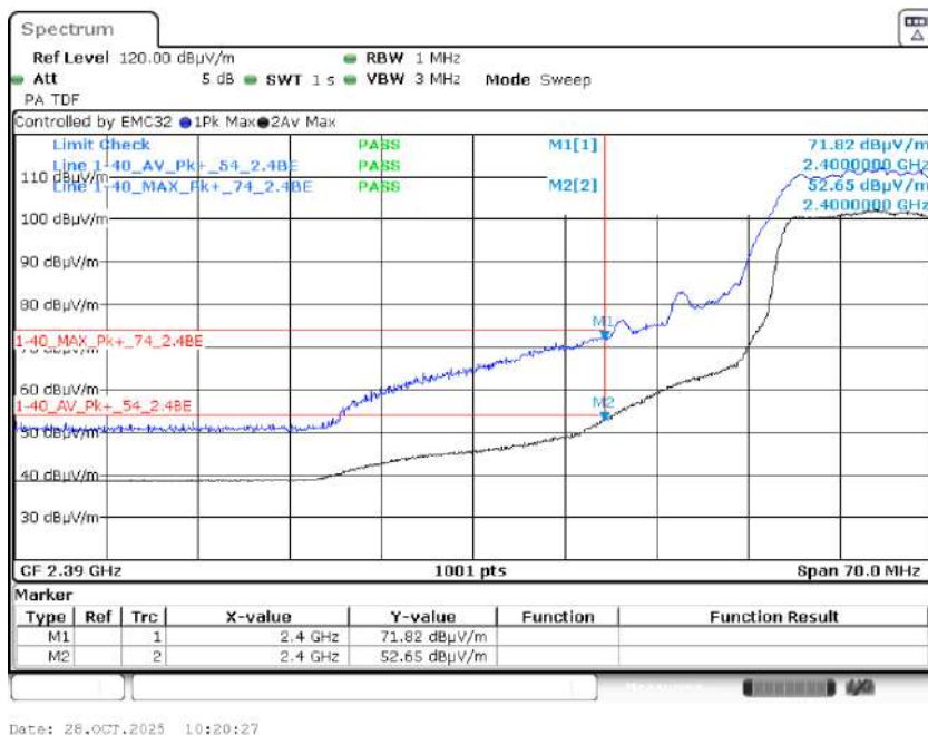
Graph 35: 2422 MHz Radiated Lower Band Edge Plot, Power Level 13
