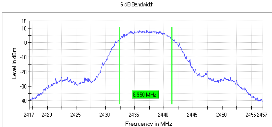
Graph 2: Middle Channel Bandwidth
