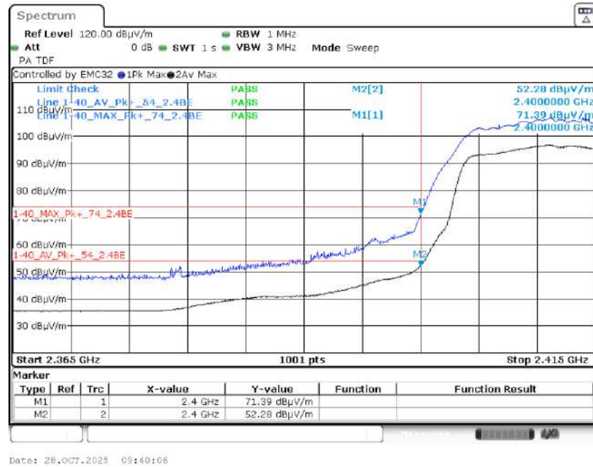
Graph 33: 2412 MHz Radiated Lower Band Edge Plot, Power Level 9
