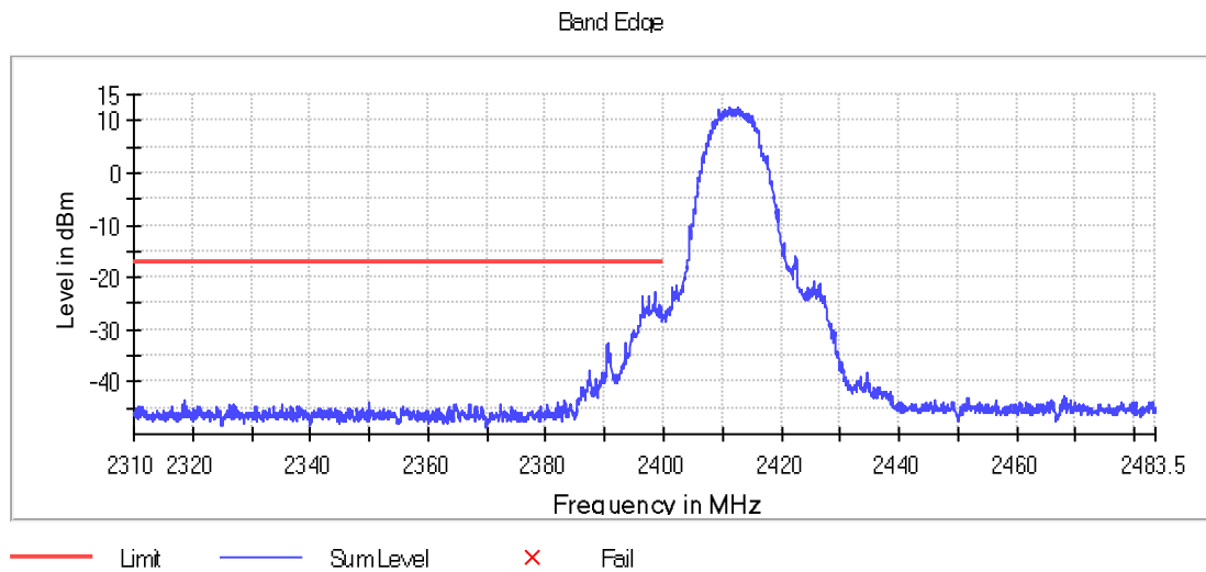
Graph 10: 2412 MHz Lower Band Edge Plot, Power Level 20
