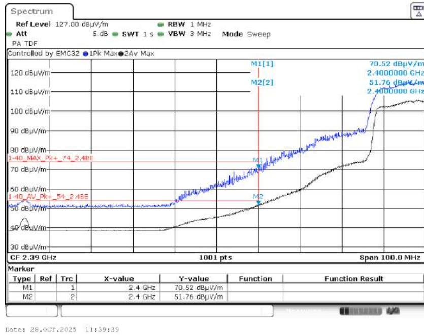
Graph 69: 2437 MHz Radiated Lower Band Edge Plot, Power Level 17
