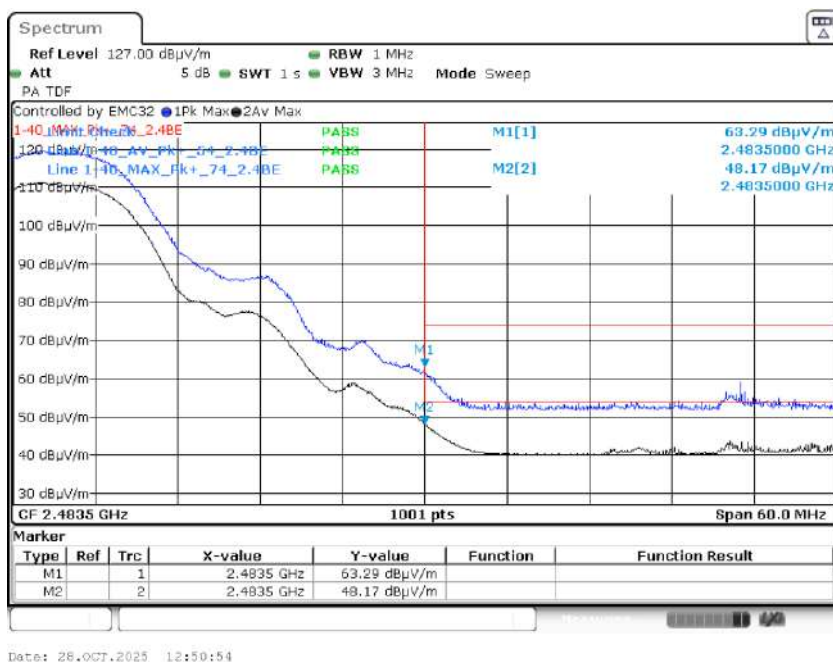
Graph 17: 2457 MHz Radiated Upper Band Edge Plot, Power Level 20
