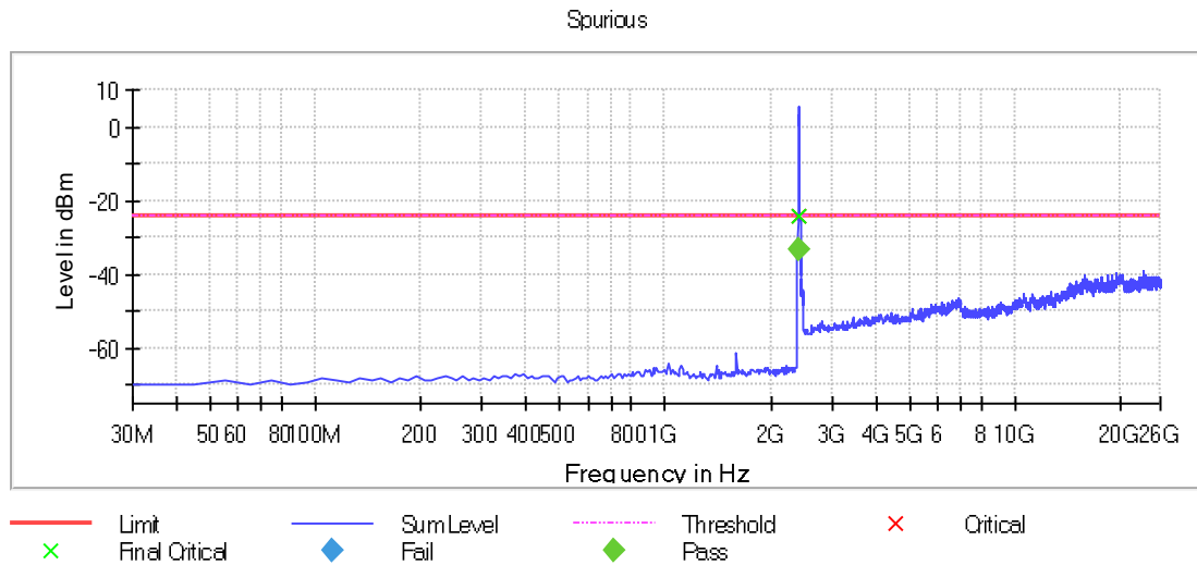
Graph 28: Transmitting on the Lowest Channel, Power Level 17
