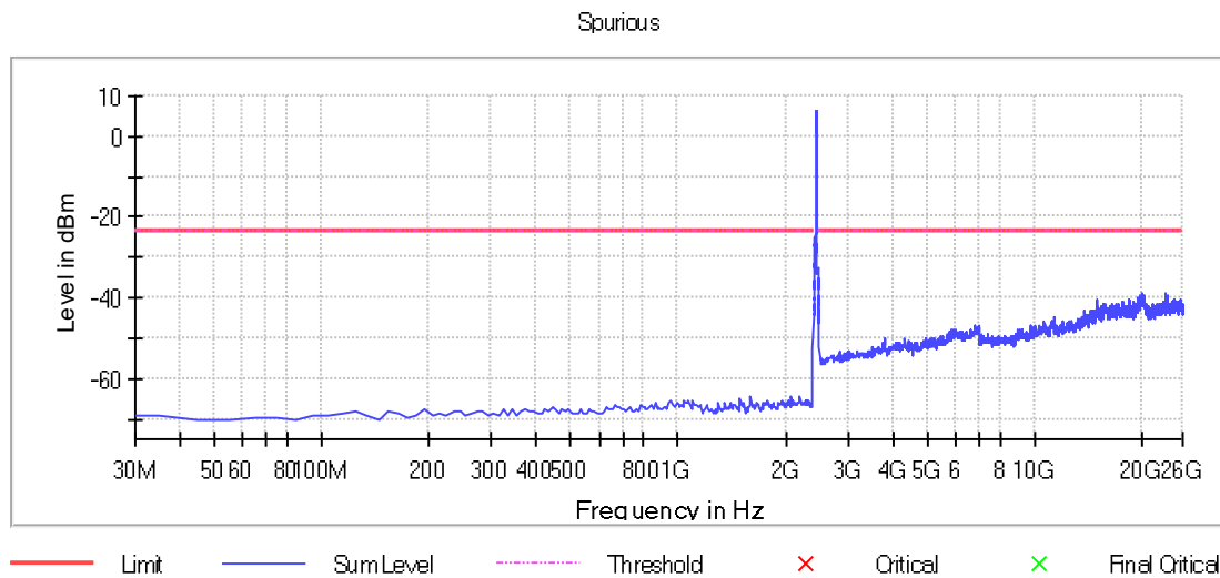
Graph 29: Transmitting on the Middle Channel, Power Level 17
