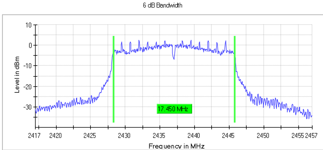
Graph 52: Middle Channel Bandwidth
