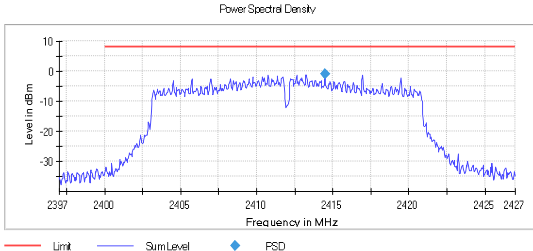
Graph 78: 2412 MHz 100 kHz PSD Plot
