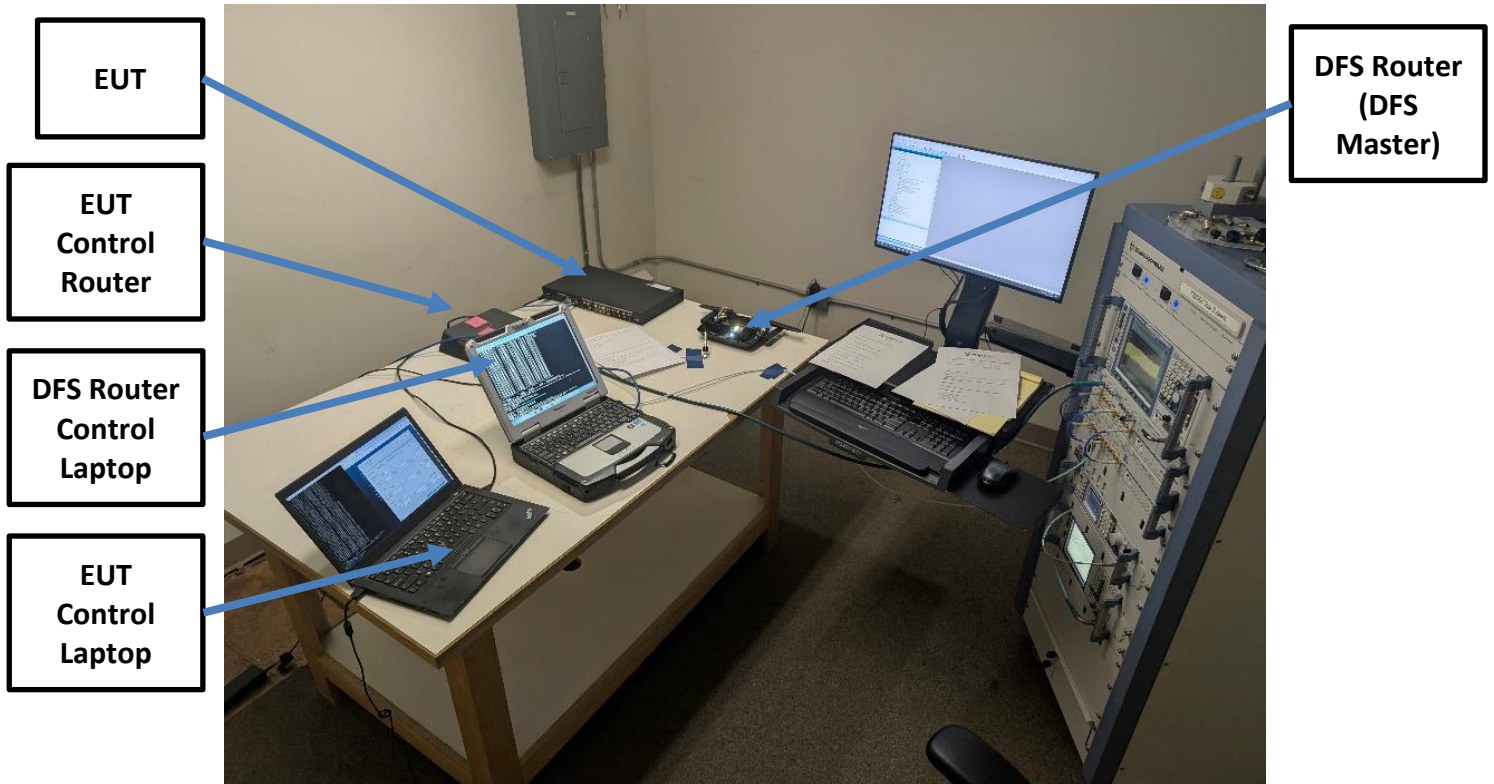
Photograph 8: DFS Test Setup
