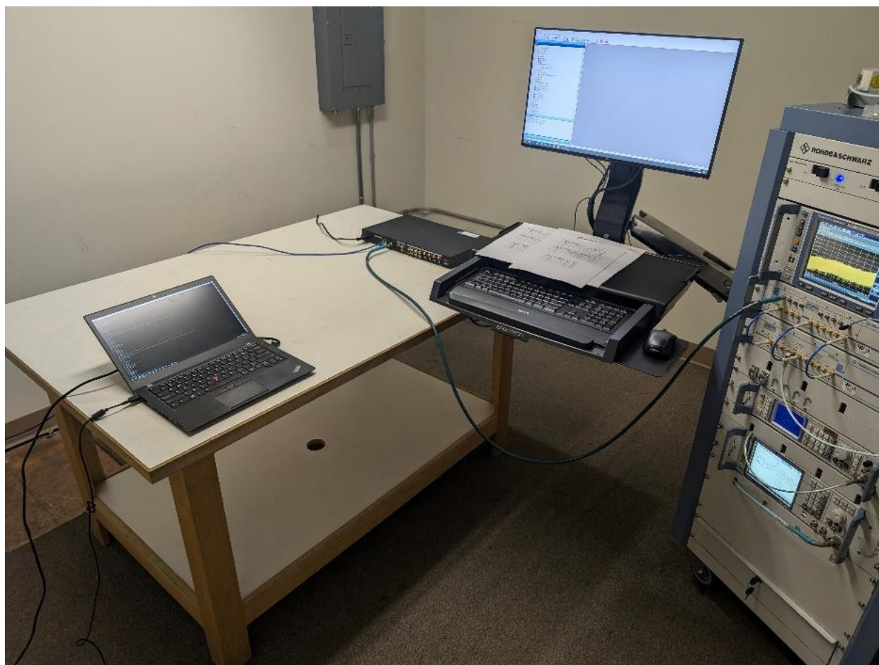
Photograph 7: Antenna Port Conducted Emissions Setup
