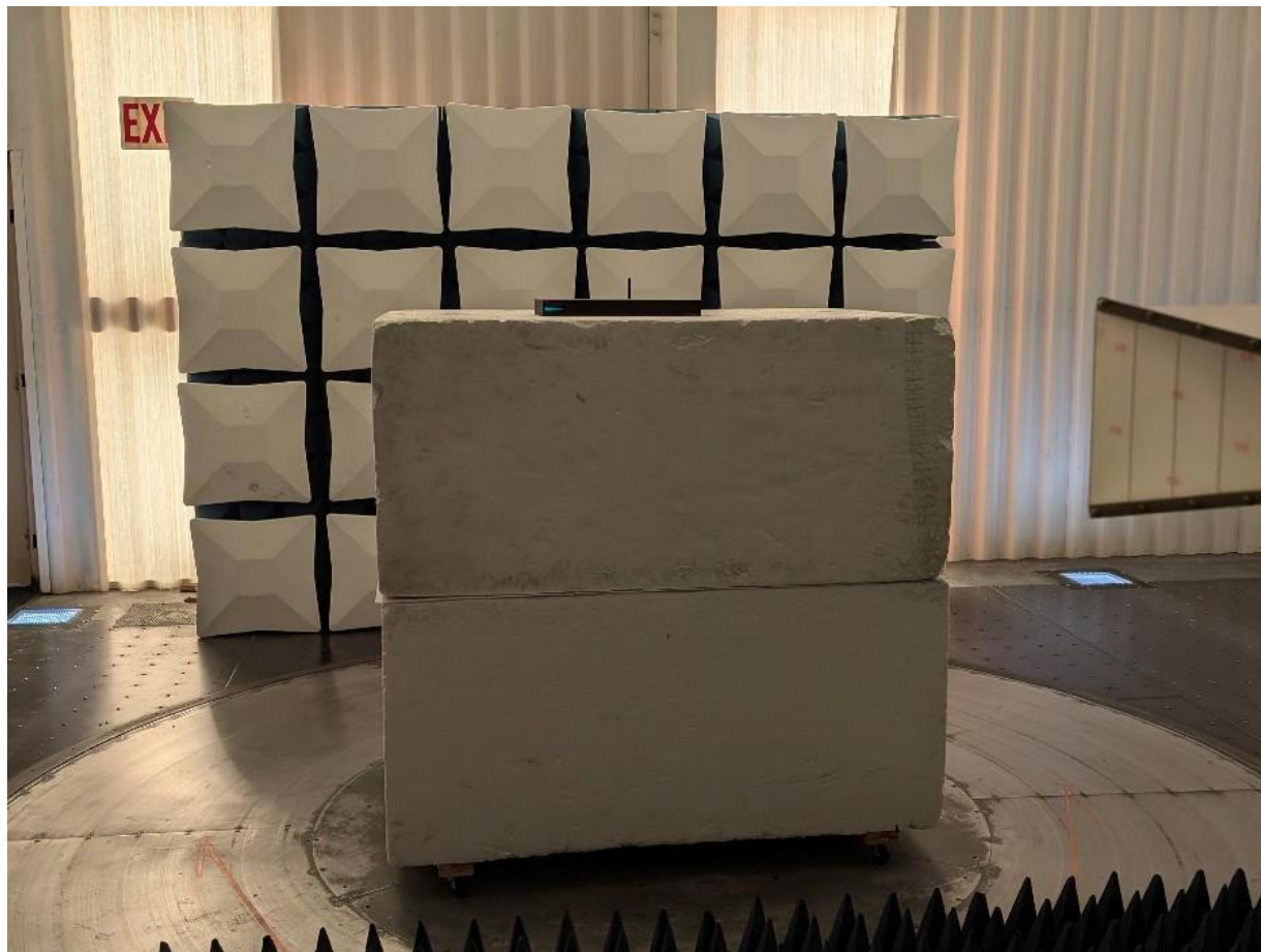
Photograph 1: Front View Radiated Emissions Worst Case Configuration
