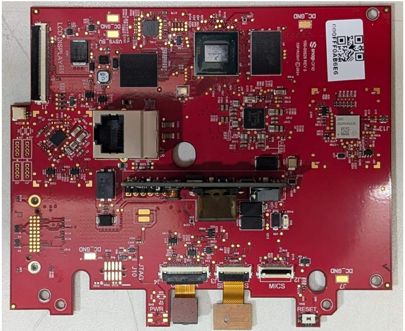
Photograph 3 – Top view of PCB
