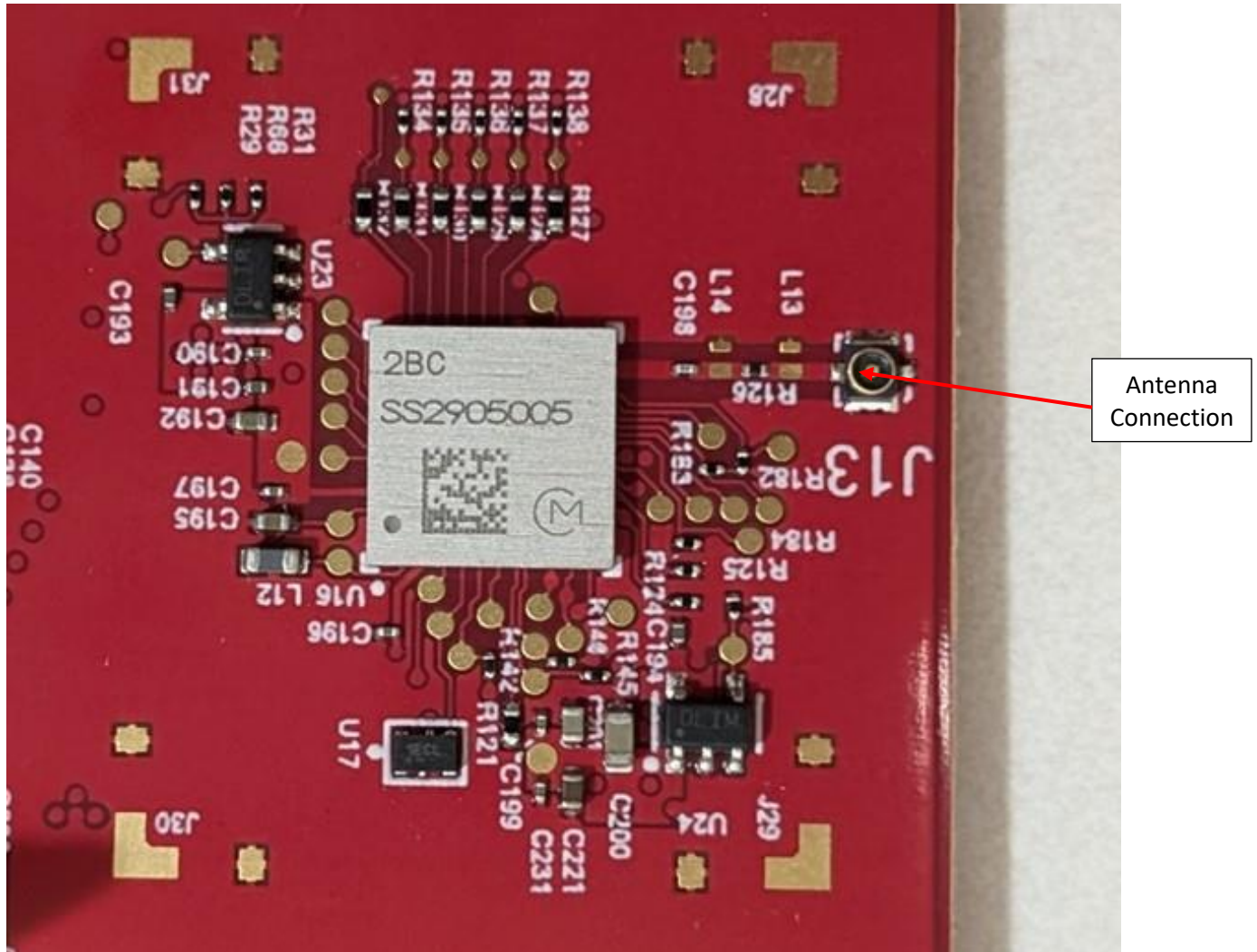
Photograph 1 –View of the RF Circuitry
