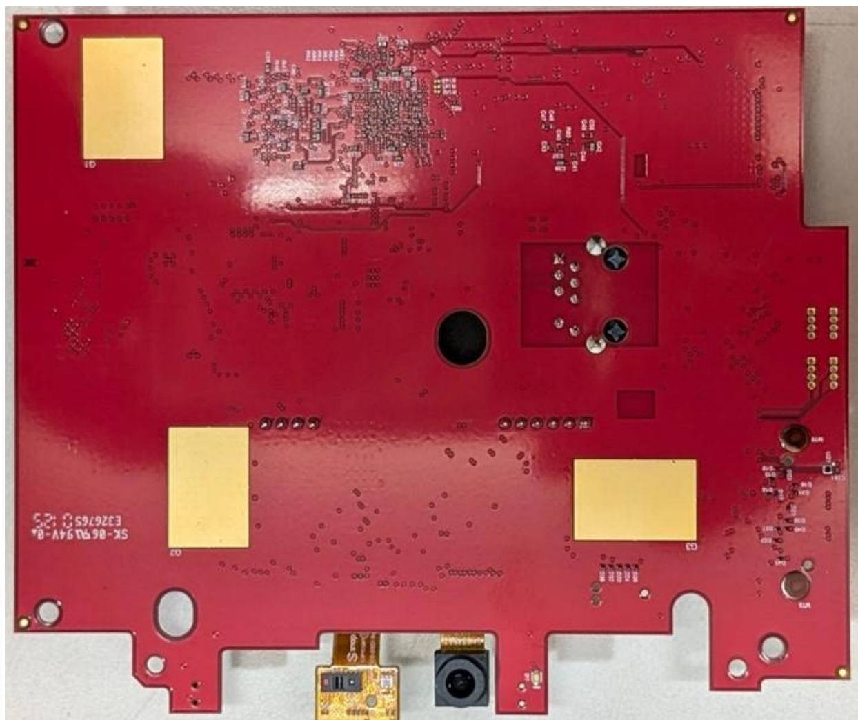
Photograph 4 – Bottom View of PCB
