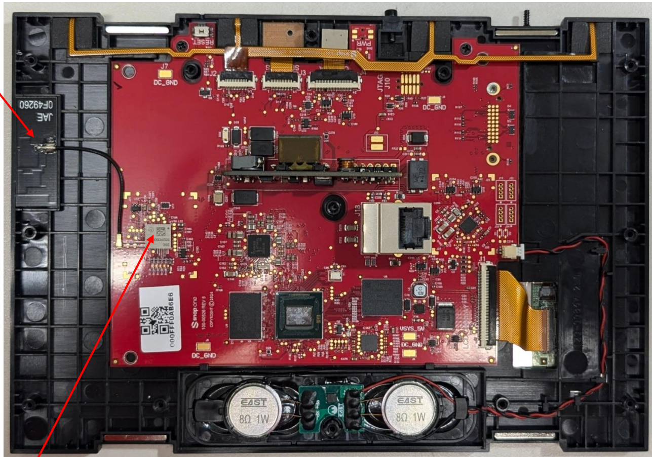
Photograph 2 – Top view of PCB in Housing, T5IW8
