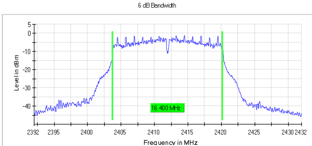
Graph 34: Lowest Channel Bandwidth
