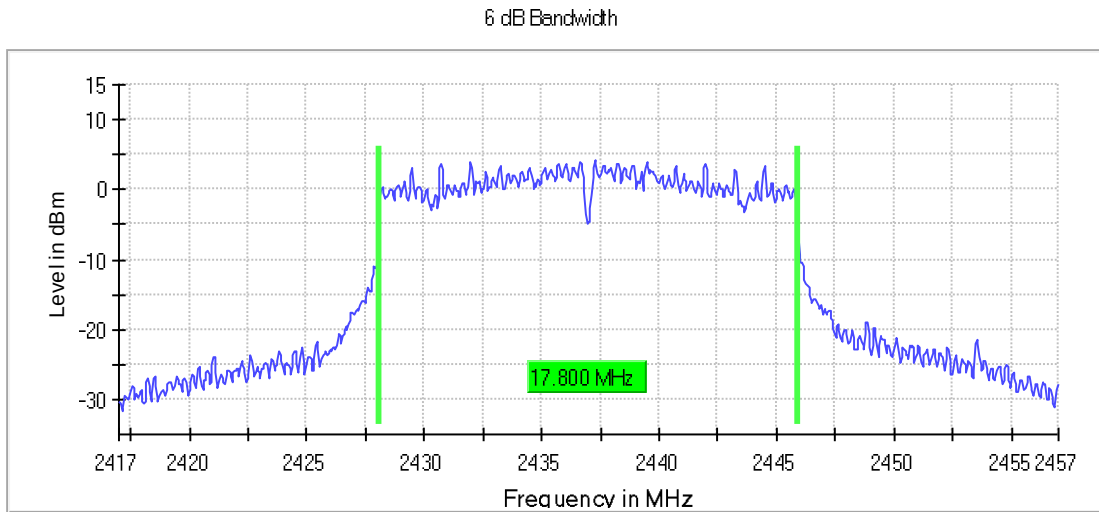
Graph 96: Middle Channel Bandwidth
