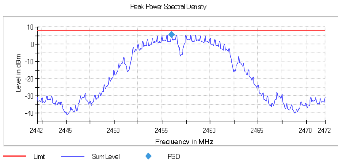
Graph 32: 2457 MHz Output 100 kHz PSD Plot
