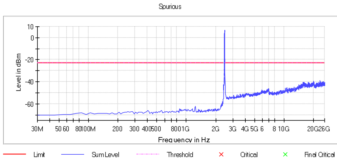
Graph 51: Transmitting on the Highest Channel, Power Level 20
