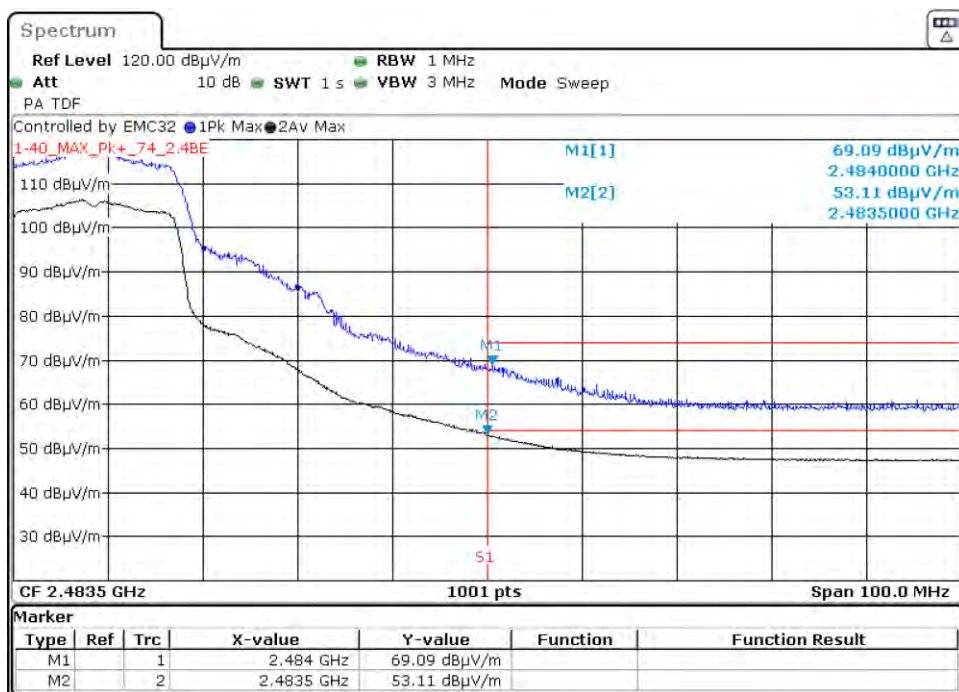
Graph 140: 2442 MHz Radiated Upper Band Edge Plot, Power Level 18 (C4-T5IW11)
