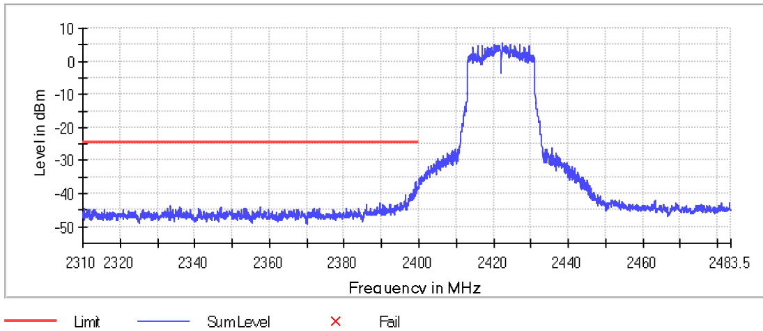
Graph 115: 2422 MHz Lower Band Edge Plot, Power Level 16
