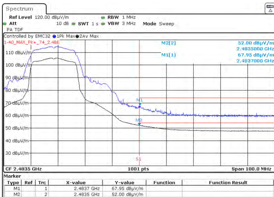
Graph 70: 2452 MHz Radiated Upper Band Edge Plot, Power Level 17 (C4-T5IW8)
