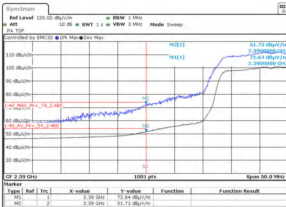
Graph 134: 2412 MHz Radiated Lower Band Edge Plot, Power Level 13 (C4-T5IW11)
