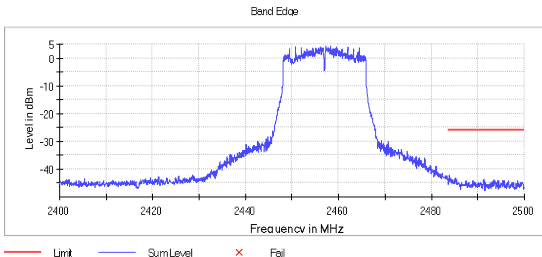
Graph 122: 2457 MHz Upper Band Edge Plot, Power Level 15
