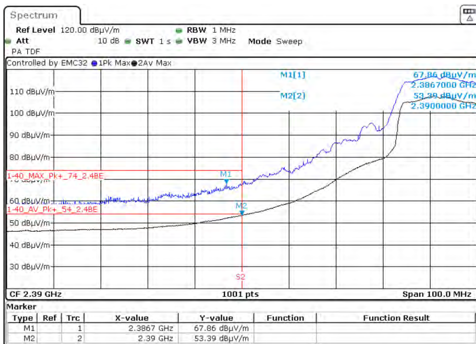
Graph 67: 2432 MHz Radiated Lower Band Edge Plot, Power Level 20 (C4-T5IW8)
