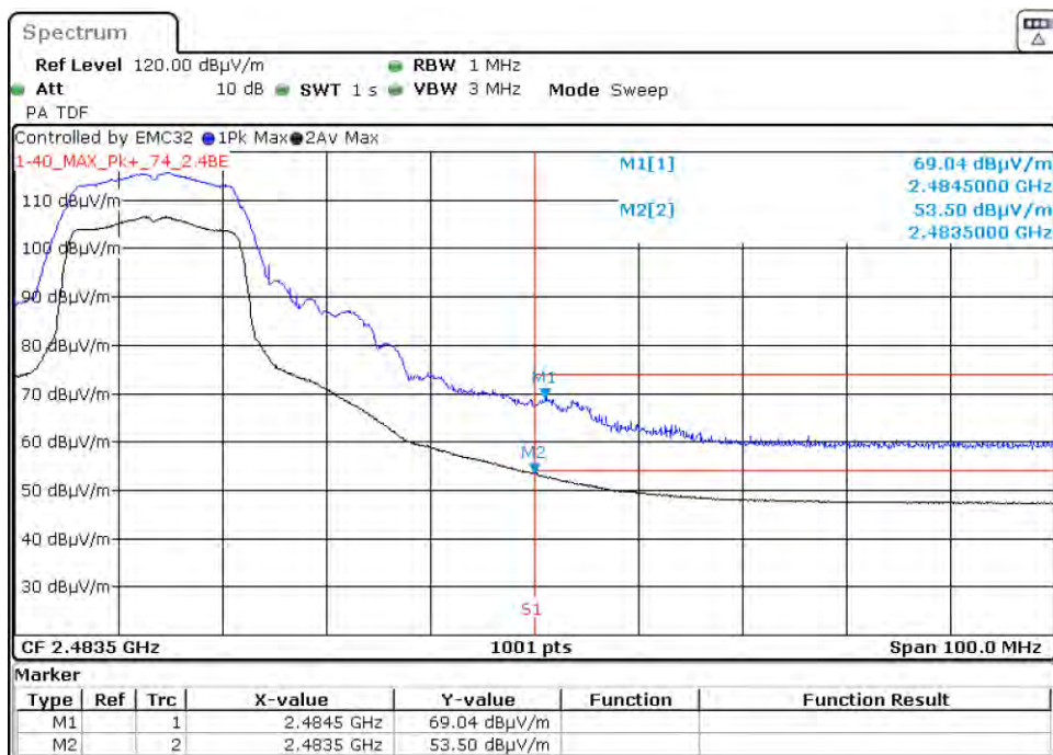
Graph 80: 2447 MHz Radiated Upper Band Edge Plot, Power Level 17 (C4-T5IW11)
