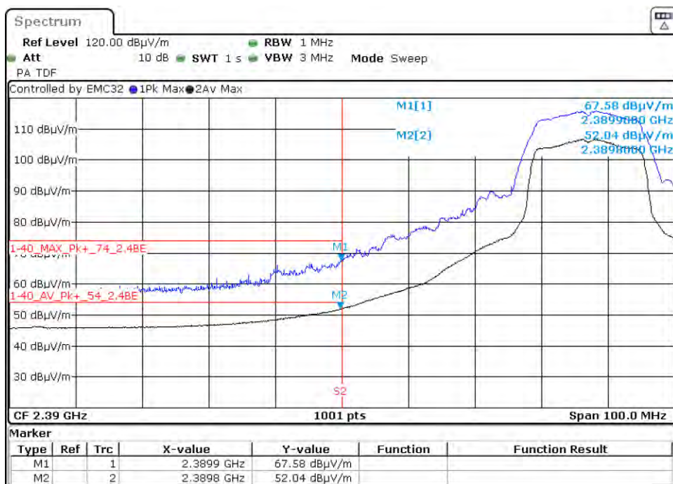
Graph 76: 2427 MHz Radiated Lower Band Edge Plot, Power Level 17 (C4-T5IW11)
