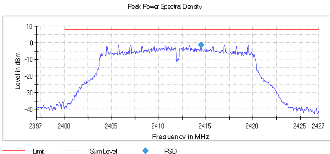
Graph 84: 2412 MHz 100 kHz PSD Plot
