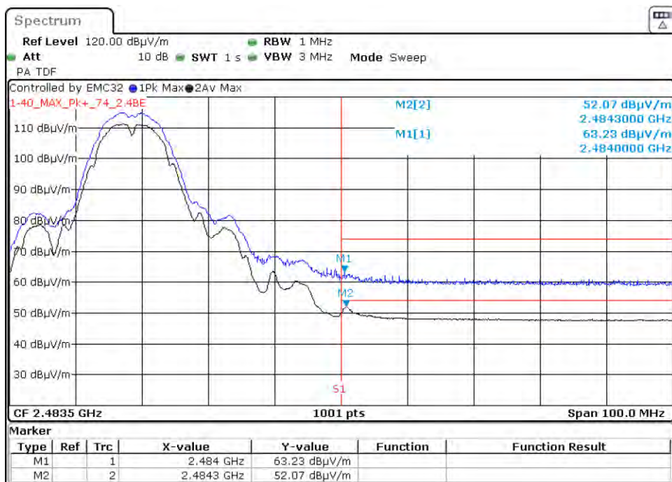
Graph 25: 2452 MHz Radiated Upper Band Edge Plot, Power Level 20 (C4-T5IW11)
