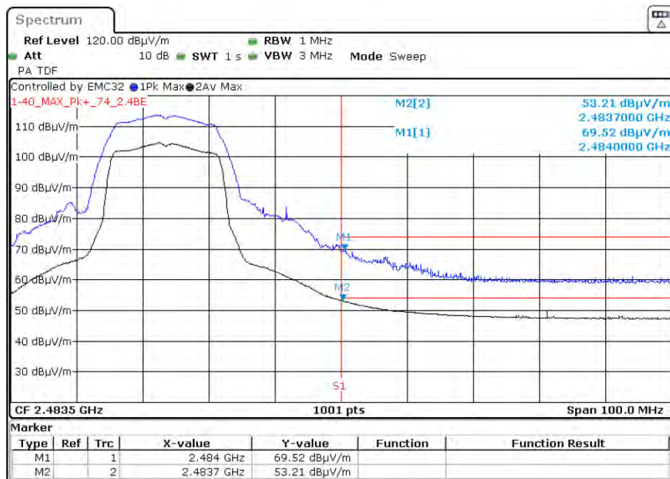
Graph 82: 2457 MHz Radiated Upper Band Edge Plot, Power Level 15 (C4-T5IW11)
