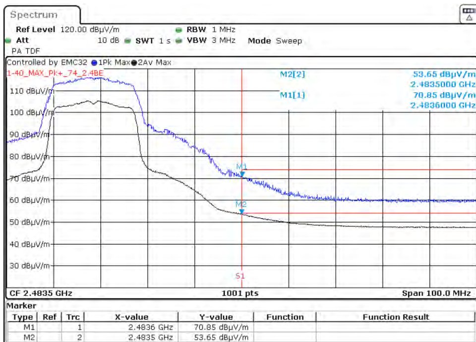
Graph 131: 2452 MHz Radiated Upper Band Edge Plot, Power Level 18 (C4-T5IW8)
