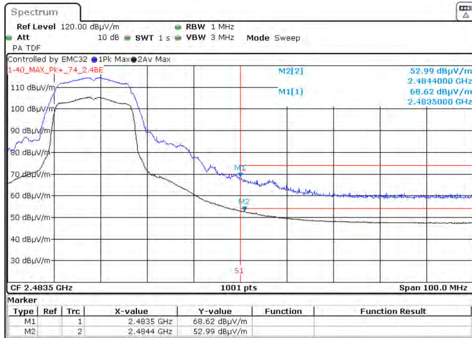
Graph 81: 2452 MHz Radiated Upper Band Edge Plot, Power Level 16 (C4-T5IW11)
