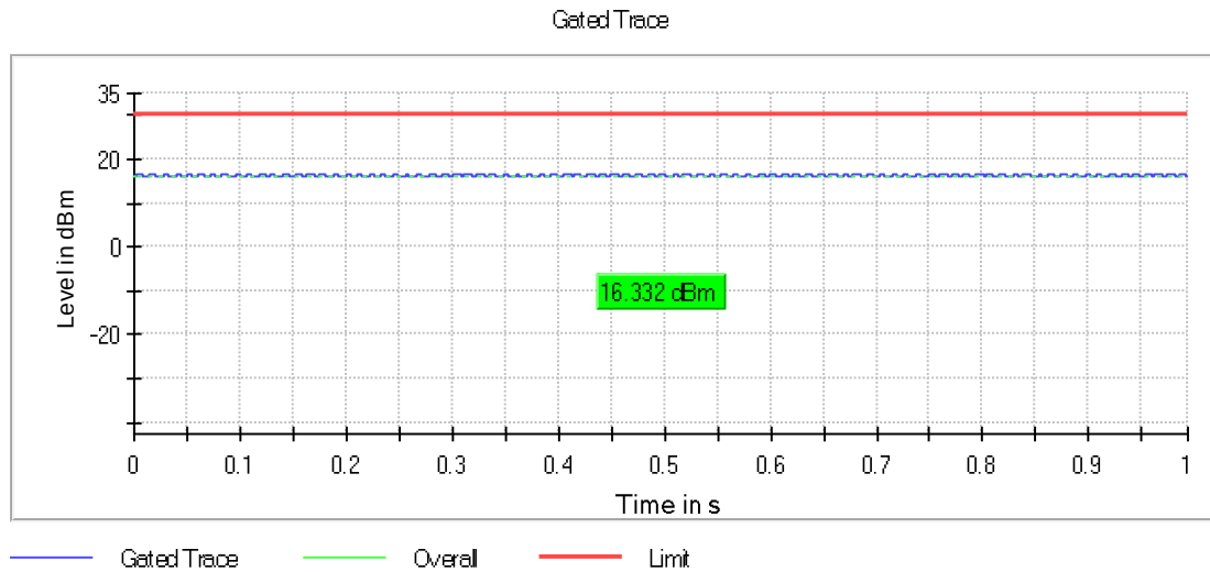
Graph 8: 2457 MHz Output Power Plot
