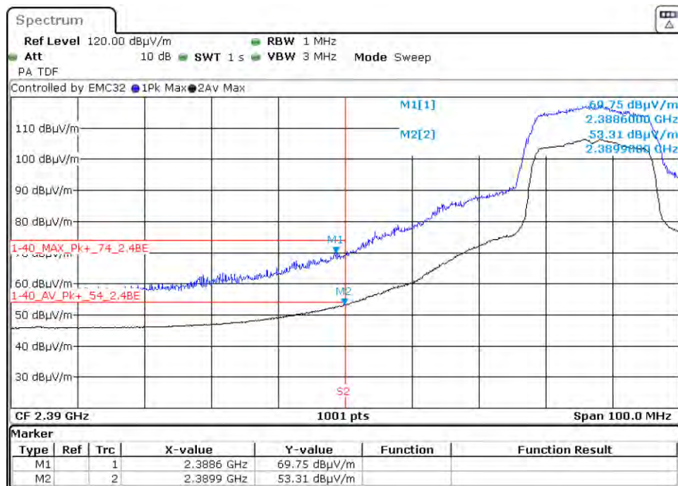
Graph 137: 2427 MHz Radiated Lower Band Edge Plot, Power Level 18 (C4-T5IW11)
