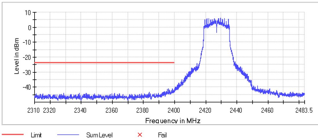
Graph 55: 2427 MHz Lower Band Edge Plot, Power Level 17
