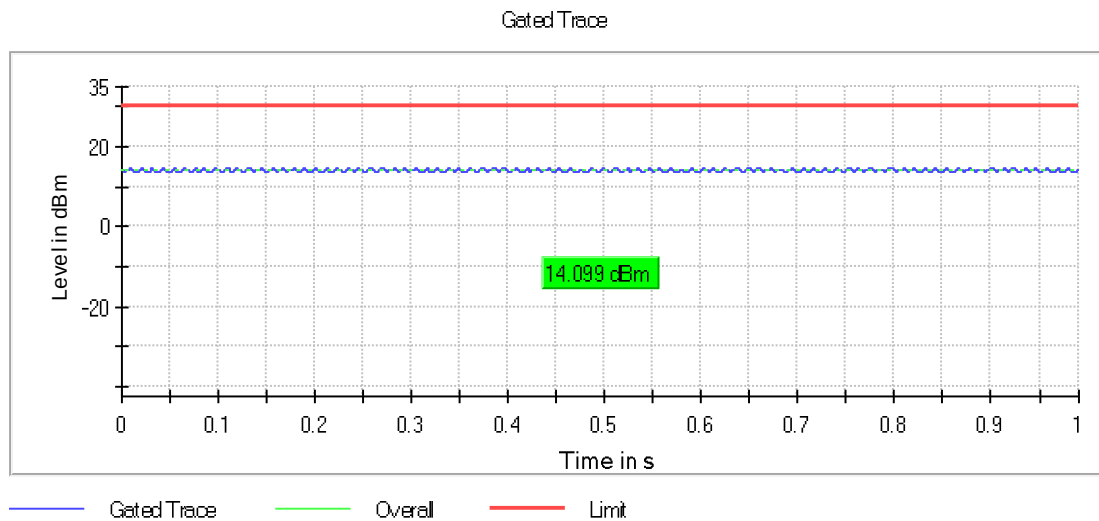
Graph 9: 2462 MHz Output Power Plot
