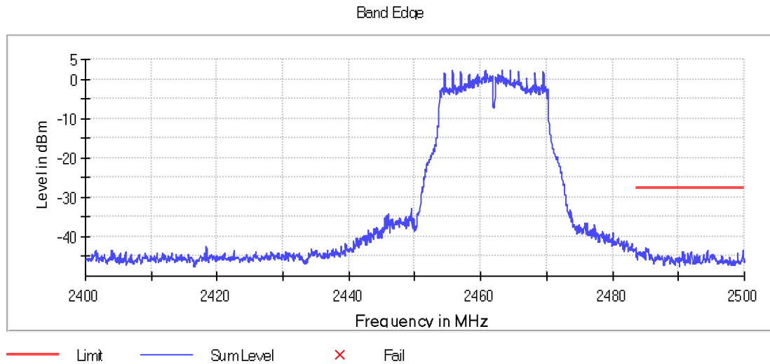
Graph 62: 2462 MHz Upper Band Edge Plot, Power Level 13
