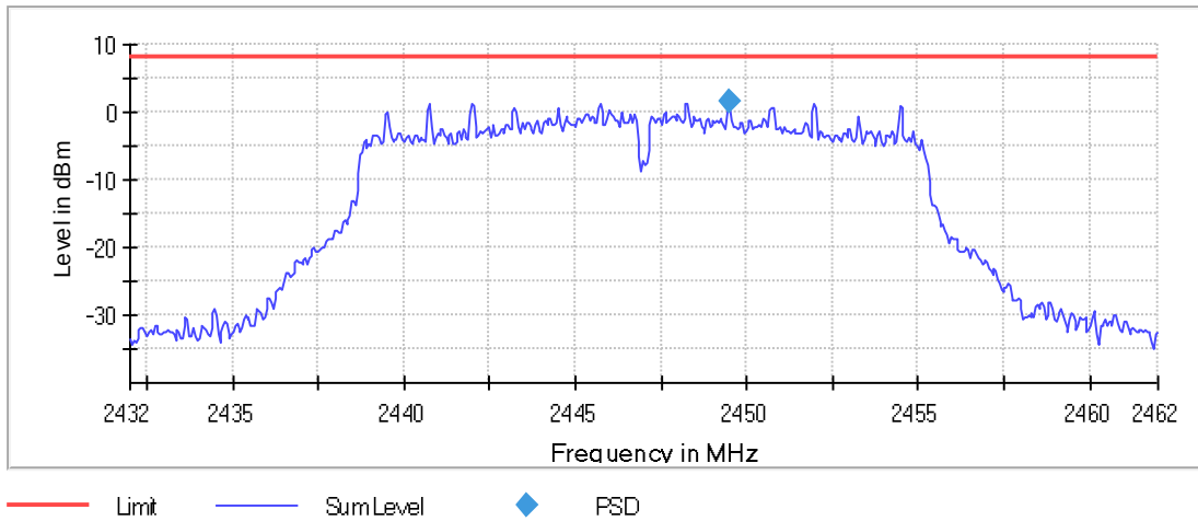
Graph 91: 2447 MHz 100 kHz PSD Plot
