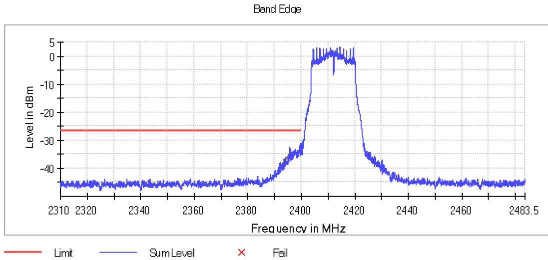
Graph 52: 2412 MHz Lower Band Edge Plot, Power Level 14
