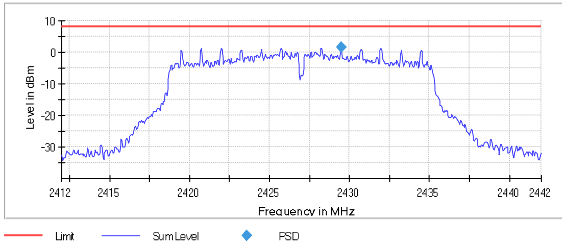
Graph 87: 2427 MHz 100 kHz PSD Plot
