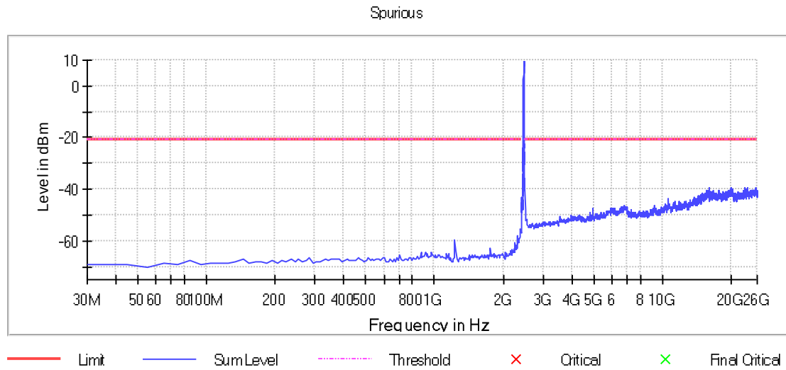
Graph 12: Transmitting on the Highest Channel, Power Level 20
