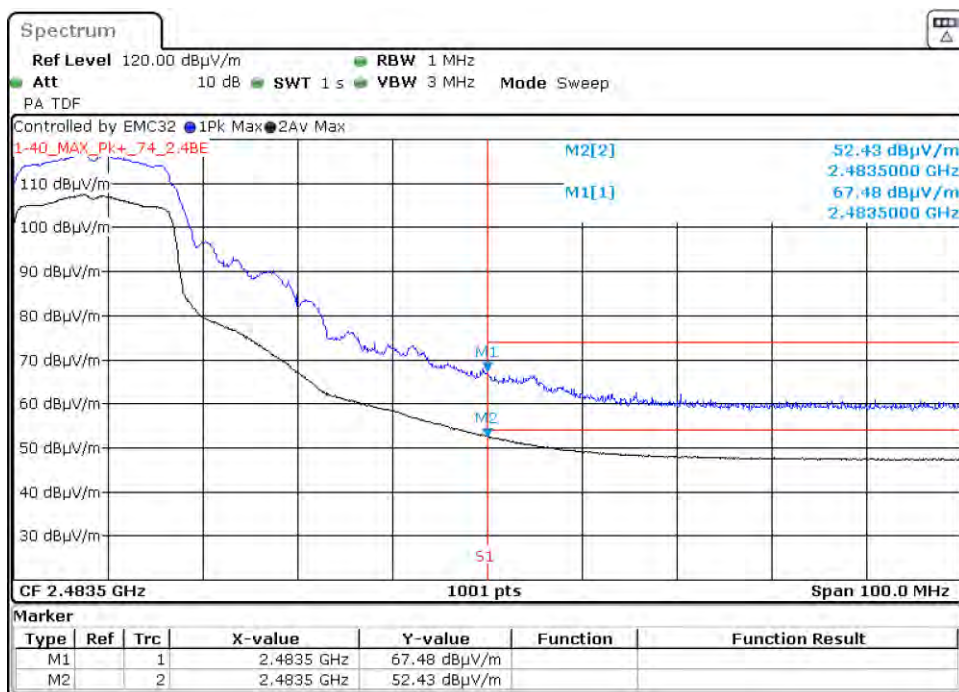
Graph 79: 2442 MHz Radiated Upper Band Edge Plot, Power Level 18 (C4-T5IW11)
