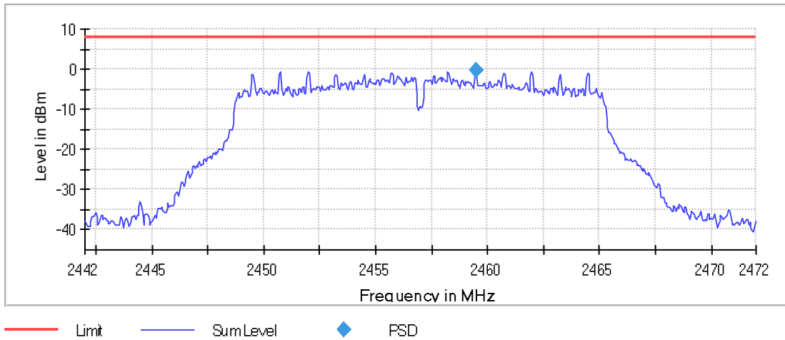
Graph 93: 2457 MHz 100 kHz PSD Plot
