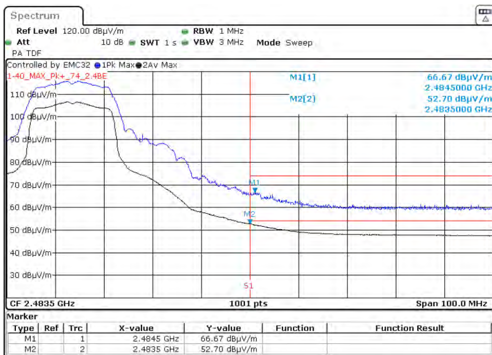
Graph 69: 2447 MHz Radiated Upper Band Edge Plot, Power Level 18 (C4-T5IW8)
