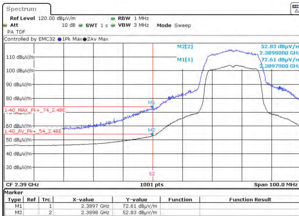
Graph 135: 2417 MHz Radiated Lower Band Edge Plot, Power Level 16 (C4-T5IW11)
