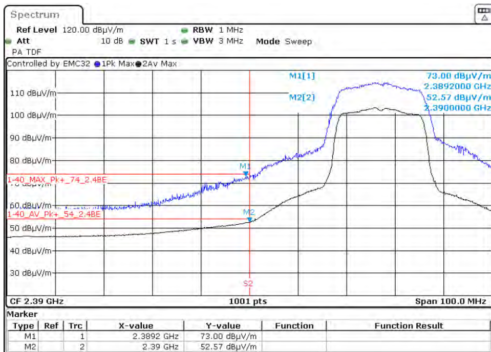
Graph 125: 2417 MHz Radiated Lower Band Edge Plot, Power Level 16 (C4-T5IW8)
