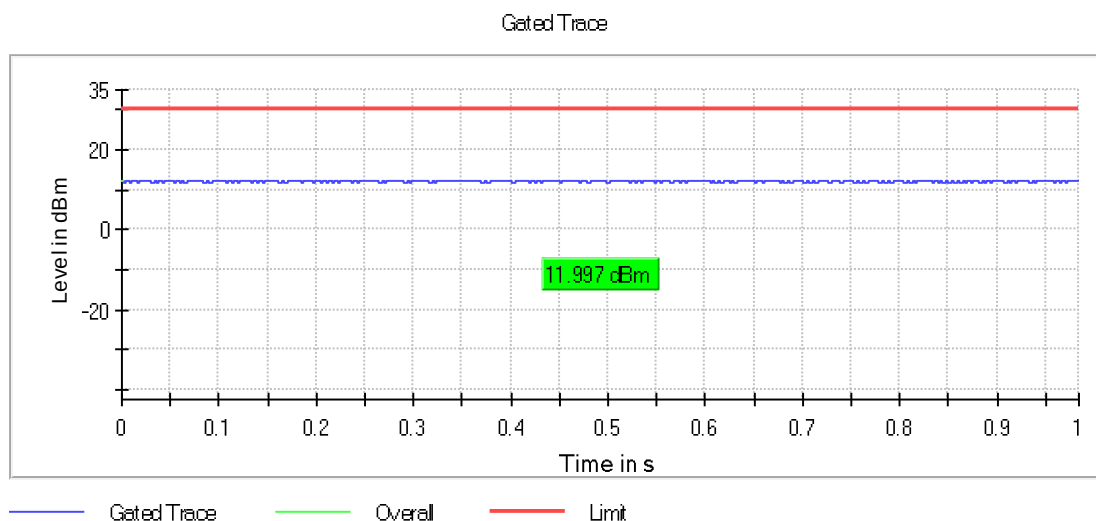
Graph 47: 2462 MHz Output Power Plot
