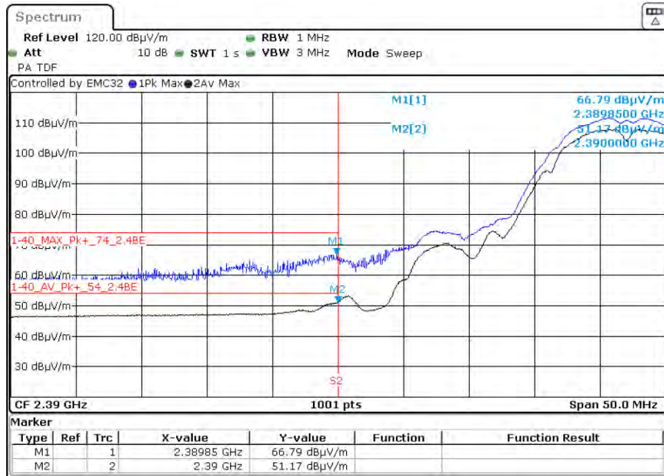
Graph 18: 2412 MHz Radiated Lower Band Edge Plot, Power Level 17 (C4-T5IW8)
