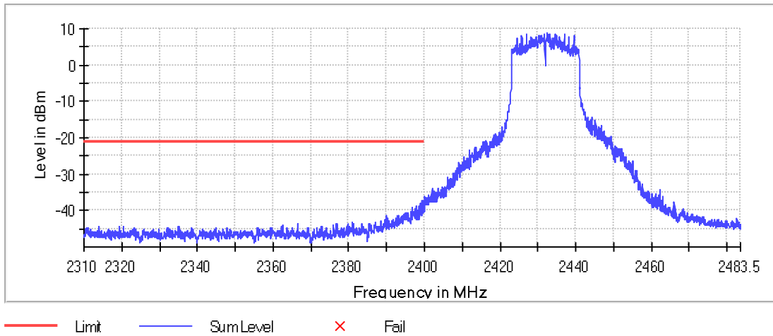
Graph 117: 2432 MHz Lower Band Edge Plot, Power Level 20
