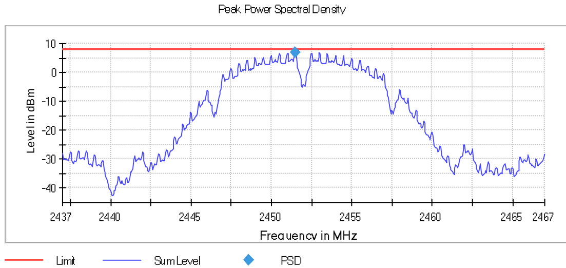
Graph 31: 2452 MHz Output 100 kHz PSD Plot
