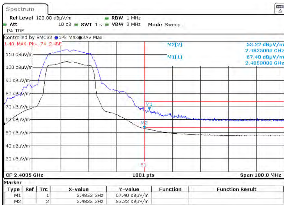
Graph 71: 2457 MHz Radiated Upper Band Edge Plot, Power Level 16 (C4-T5IW8)
