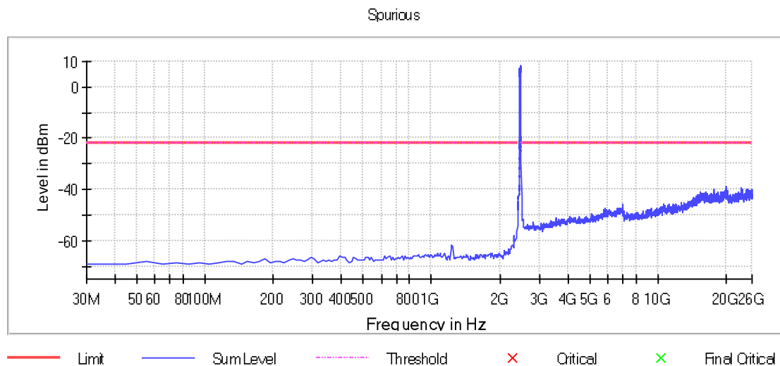
Graph 112: Transmitting on the Highest Channel, Power Level 20
