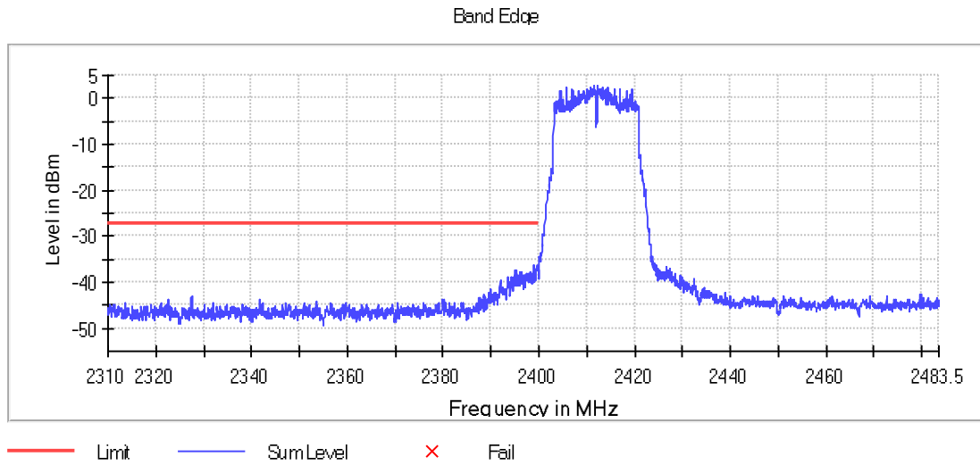
Graph 113: 2412 MHz Lower Band Edge Plot, Power Level 13
