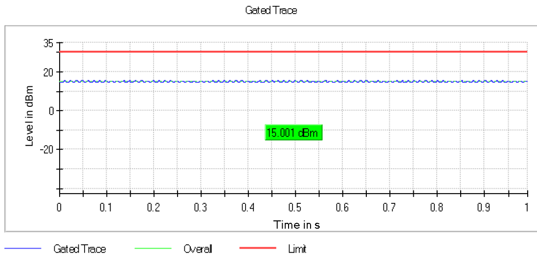
Graph 4: 2412 MHz Output Power Plot
