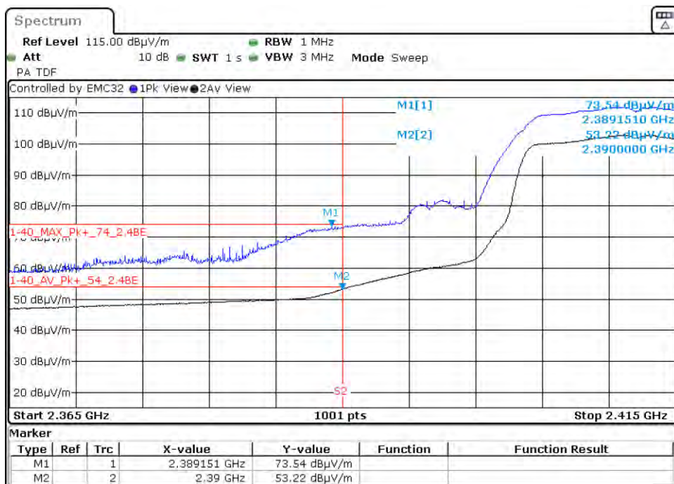
Graph 63: 2412 MHz Radiated Lower Band Edge Plot, Power Level 14 (C4-T5IW8)
