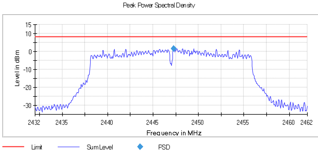
Graph 152: 2447 MHz 100 kHz PSD Plot
