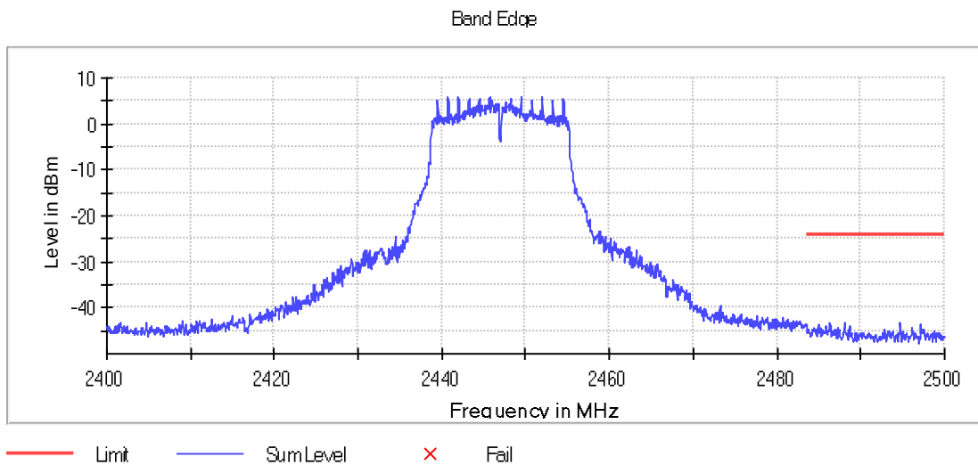
Graph 59: 2447 MHz Upper Band Edge Plot, Power Level 17
