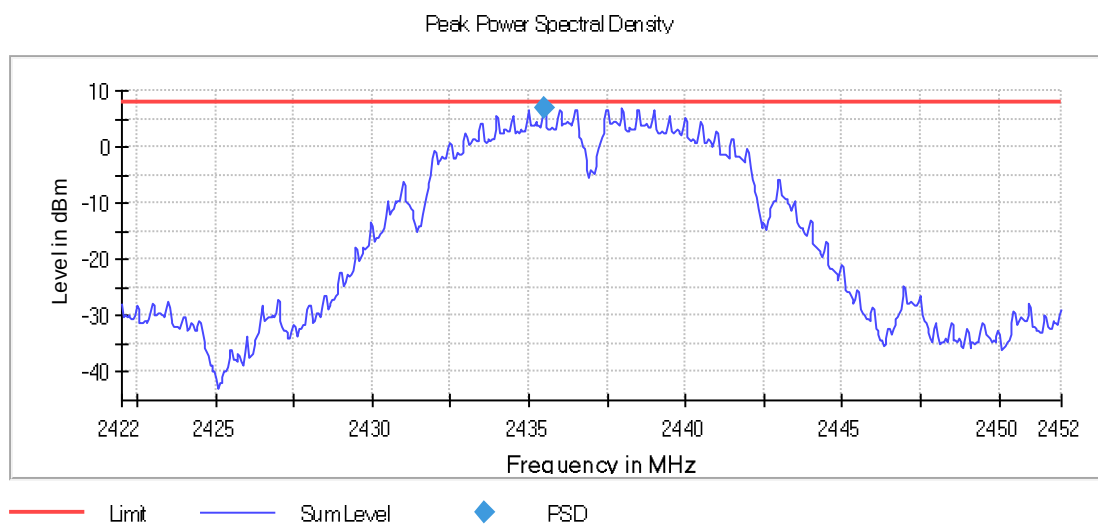
Graph 30: 2437 MHz Output 100 kHz PSD Plot
