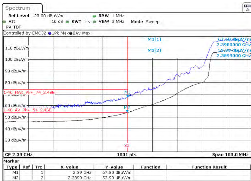
Graph 77: 2432 MHz Radiated Lower Band Edge Plot, Power Level 20 (C4-T5IW11)
