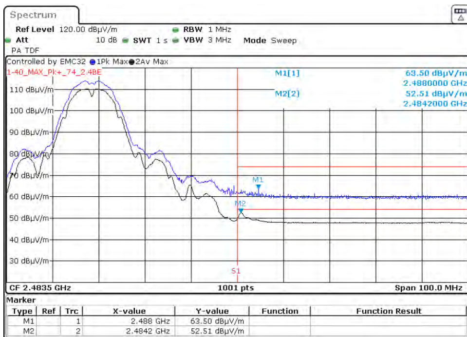
Graph 20: 2452 MHz Radiated Upper Band Edge Plot, Power Level 20 (C4-T5IW8)
