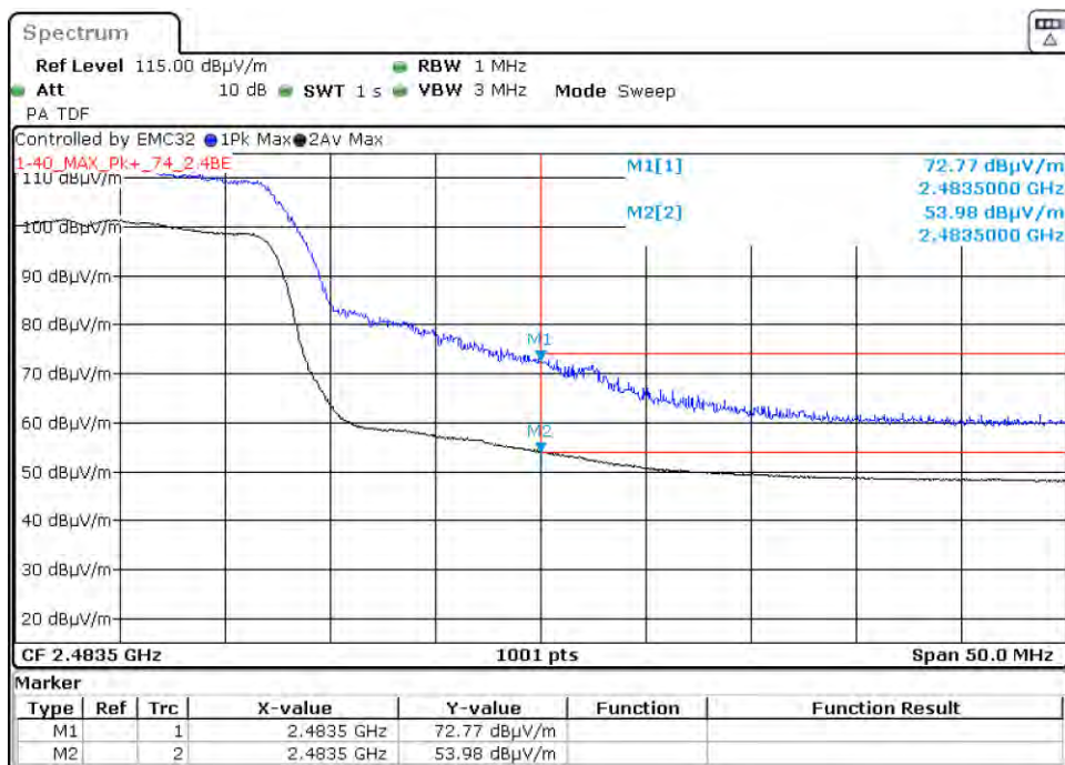
Graph 133: 2462 MHz Radiated Upper Band Edge Plot, Power Level 14 (C4-T5IW8)
