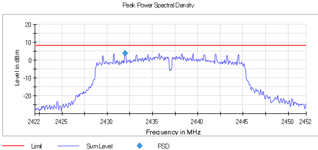
Graph 89: 2437 MHz 100 kHz PSD Plot
