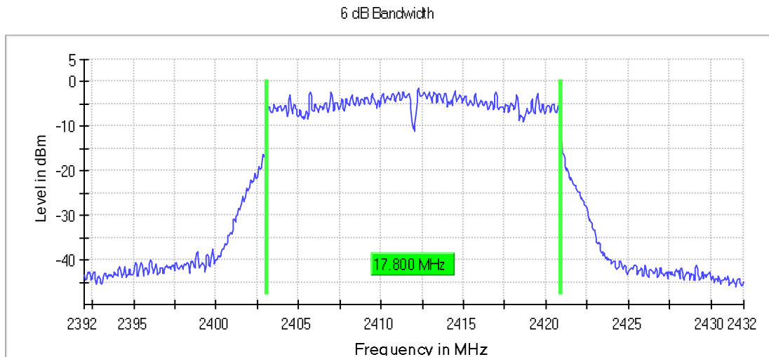
Graph 95: Lowest Channel Bandwidth
