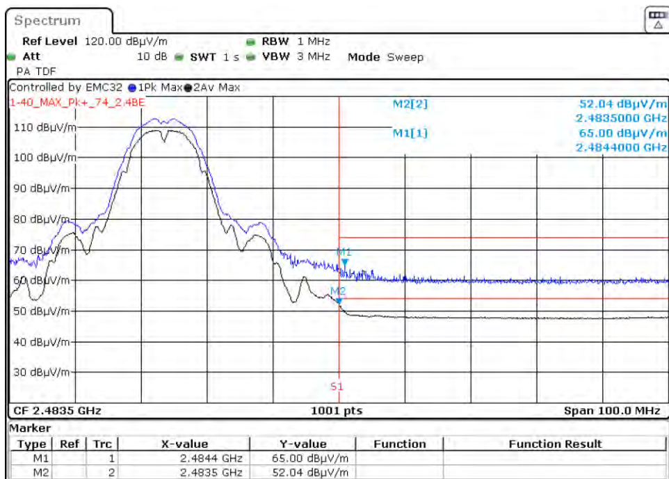
Graph 21: 2457 MHz Radiated Upper Band Edge Plot, Power Level 18 (C4-T5IW8)
