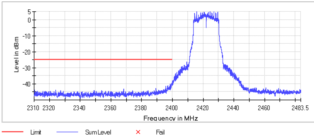
Graph 54: 2422 MHz Lower Band Edge Plot, Power Level 16
