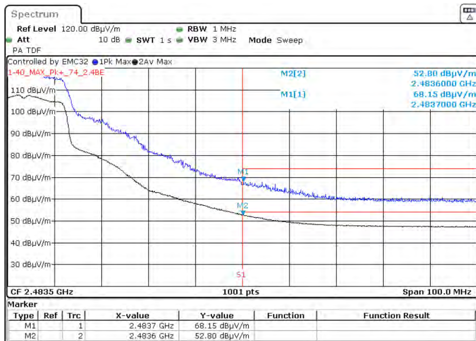
Graph 139: 2437 MHz Radiated Upper Band Edge Plot, Power Level 20 (C4-T5IW11)
