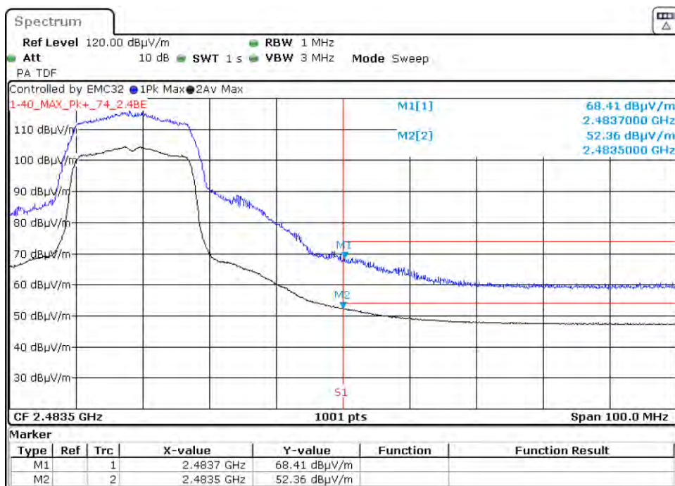
Graph 142: 2452 MHz Radiated Upper Band Edge Plot, Power Level 16 (C4-T5IW11)
