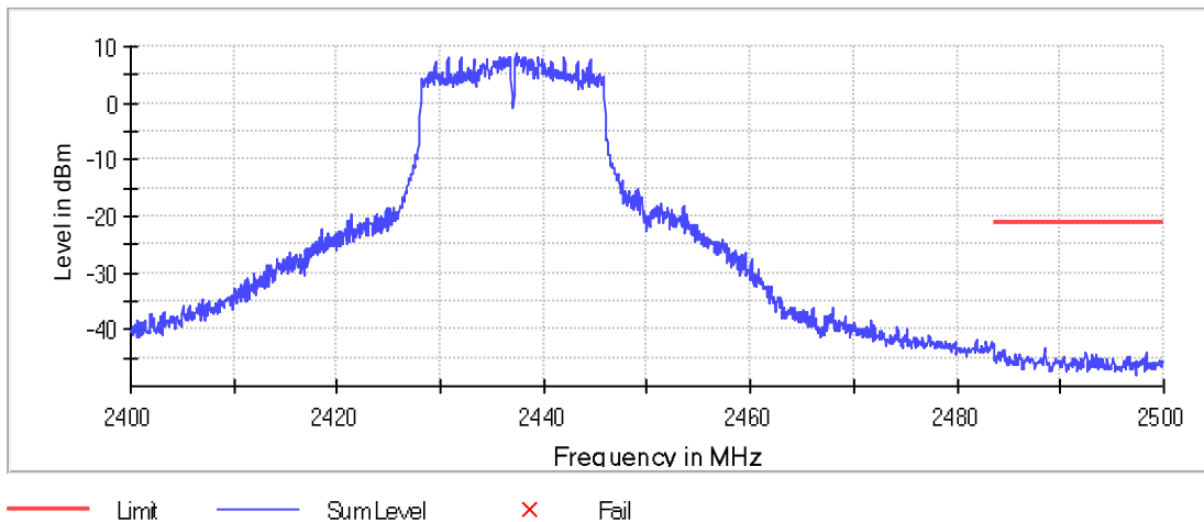
Graph 118: 2437 MHz Upper Band Edge Plot, Power Level 20
