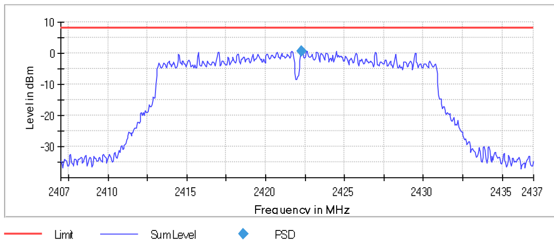
Graph 147: 2422 MHz 100 kHz PSD Plot
