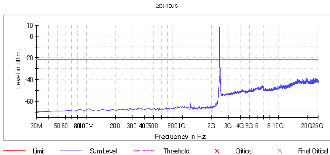
Graph 111: Transmitting on the Middle Channel, Power Level 20
