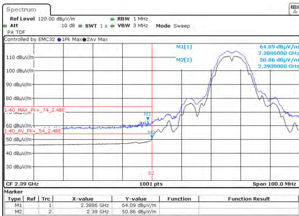
Graph 24: 2417 MHz Radiated Lower Band Edge Plot, Power Level 20 (C4-T5IW11)
