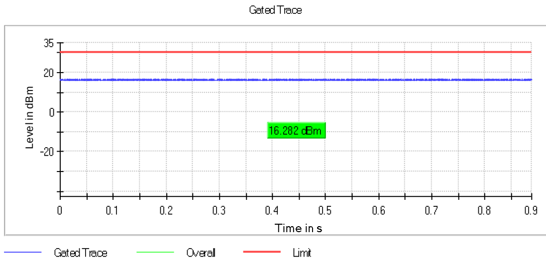
Graph 104: 2442 MHz Output Power Plot
