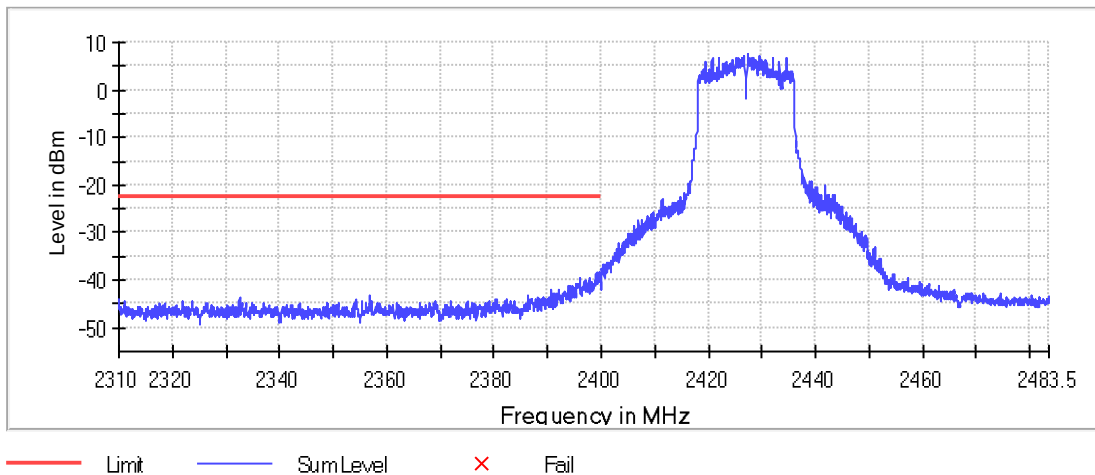
Graph 116: 2427 MHz Lower Band Edge Plot, Power Level 18
