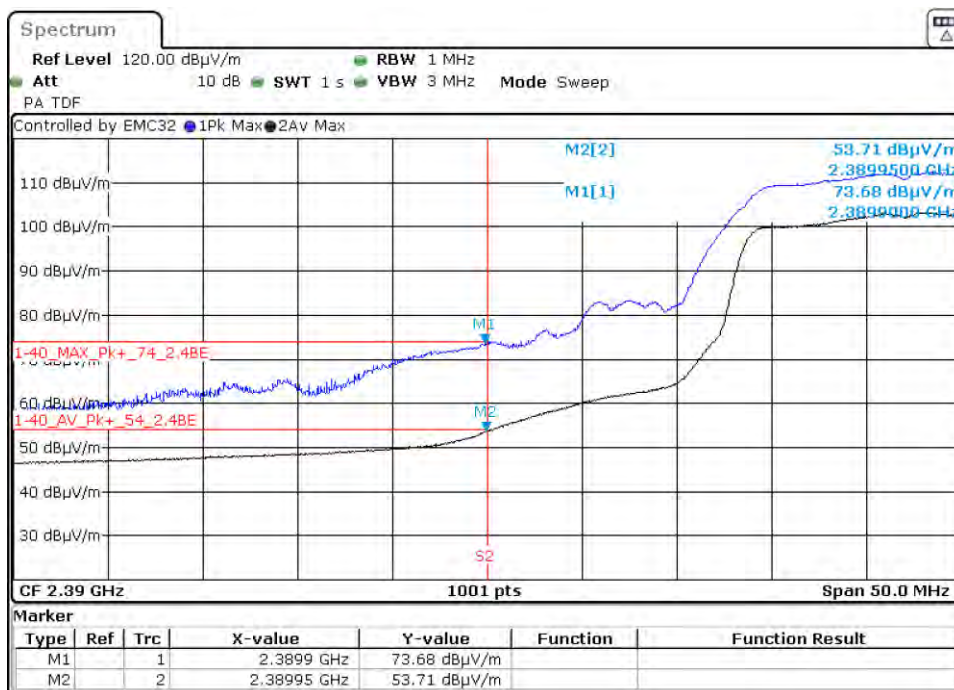
Graph 73: 2412 MHz Radiated Lower Band Edge Plot, Power Level 14 (C4-T5IW11)
