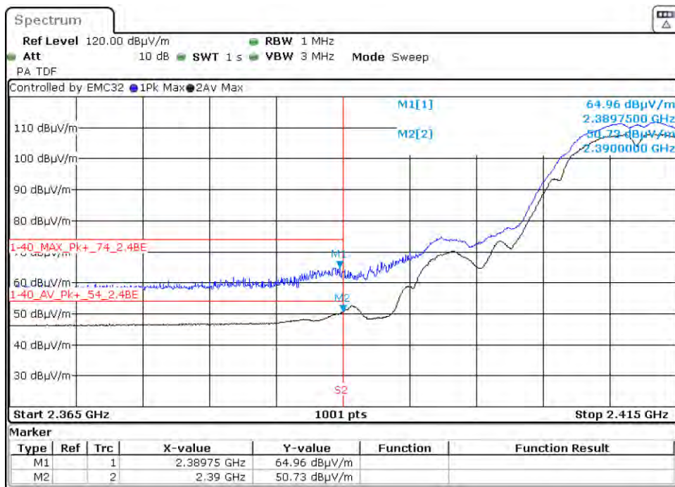
Graph 23: 2412 MHz Radiated Lower Band Edge Plot, Power Level 17 (C4-T5IW11)
