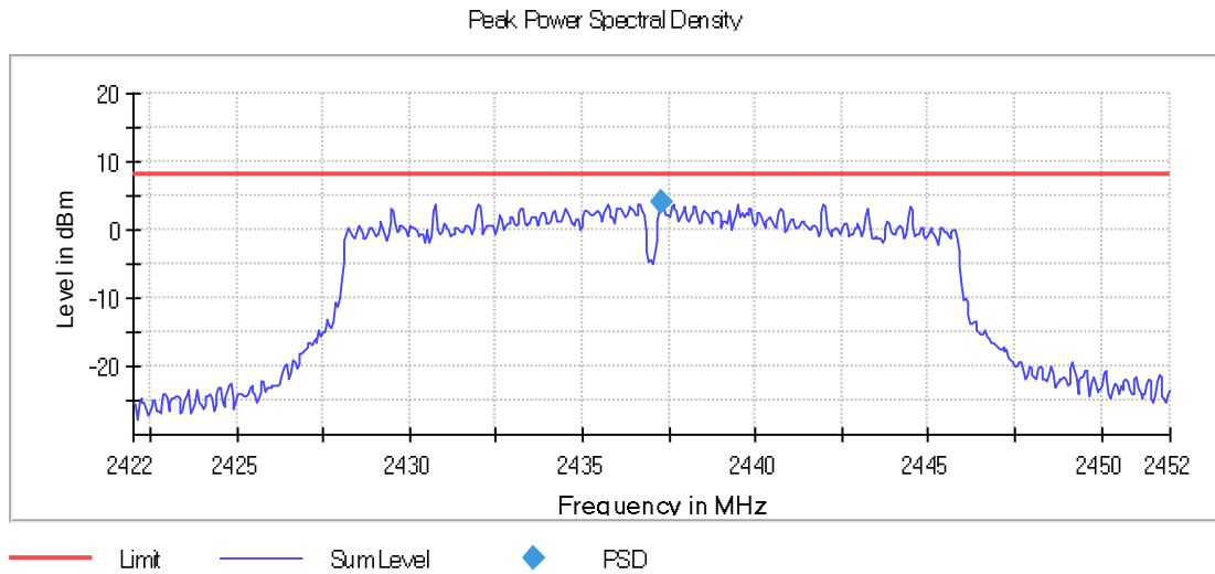
Graph 150: 2437 MHz 100 kHz PSD Plot
