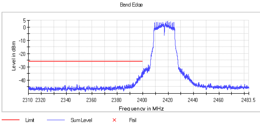
Graph 53: 2417 MHz Lower Band Edge Plot, Power Level 15
