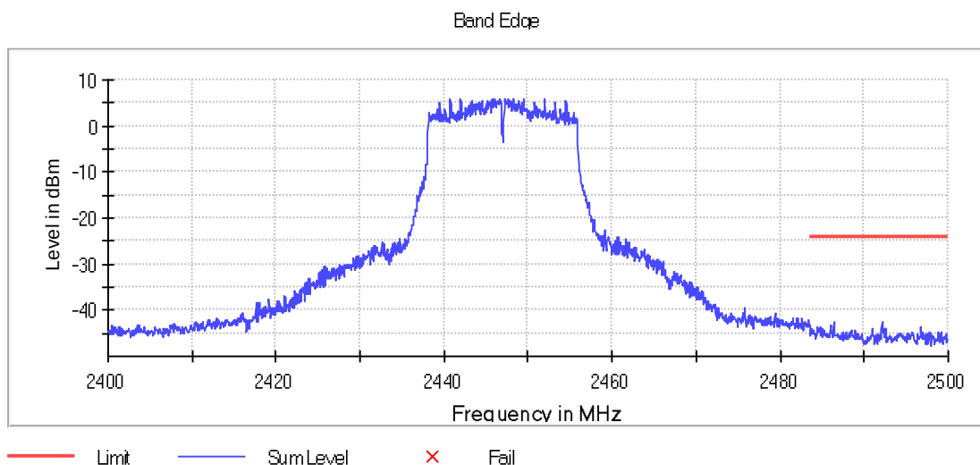
Graph 120: 2447 MHz Upper Band Edge Plot, Power Level 17
