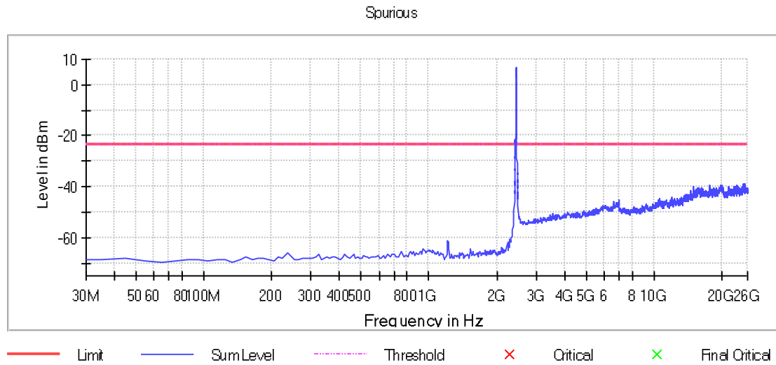
Graph 50: Transmitting on the Middle Channel, Power Level 20
