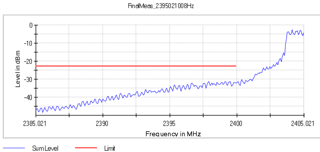
Graph 49: Critical Point (2395.021 MHz) Transmitting on the Lowest Channel, Power Level 20
