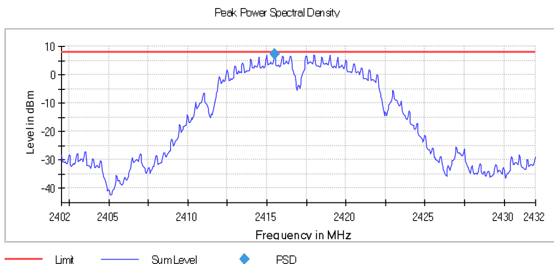
Graph 29: 2417 MHz 100 kHz PSD Plot
