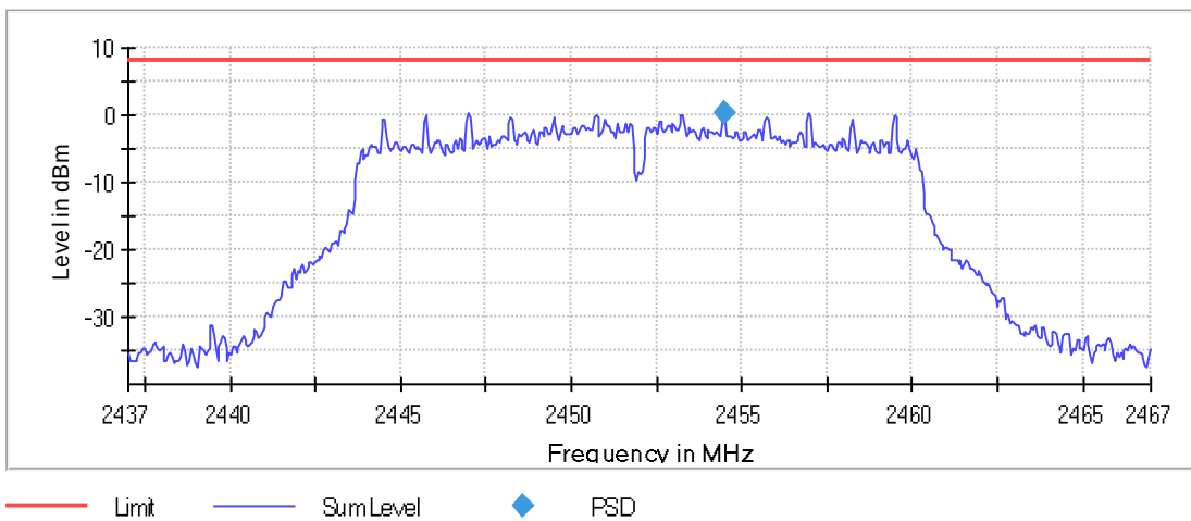
Graph 92: 2452 MHz 100 kHz PSD Plot
