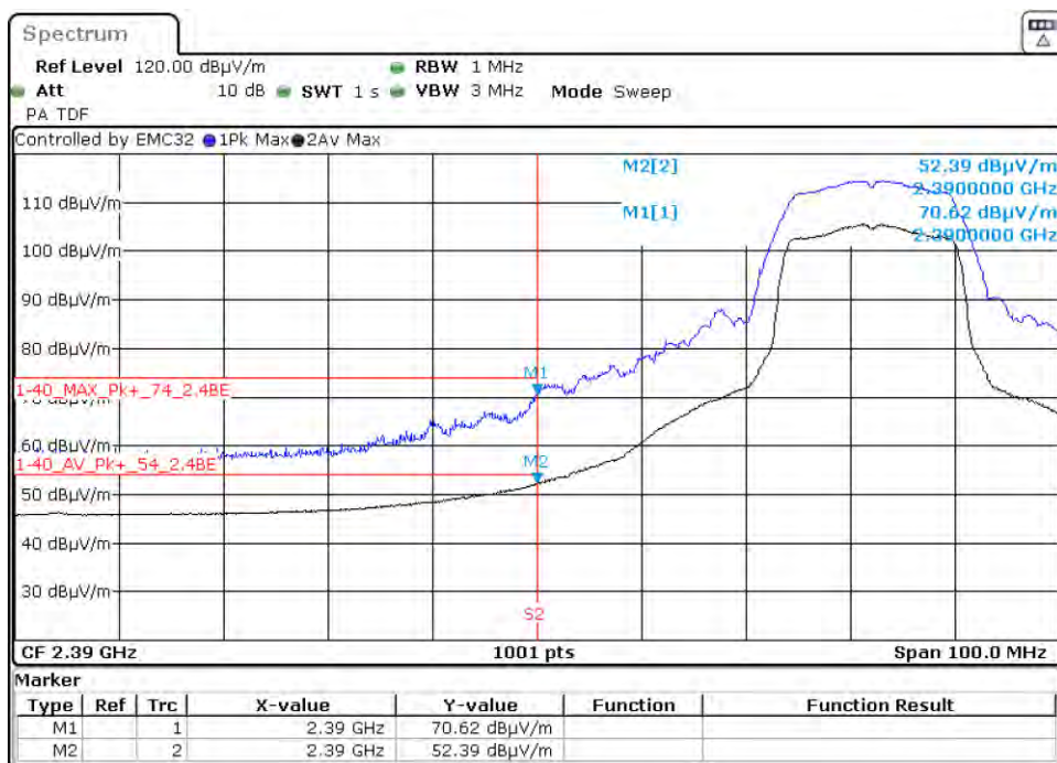
Graph 75: 2422 MHz Radiated Lower Band Edge Plot, Power Level 16 (C4-T5IW11)
