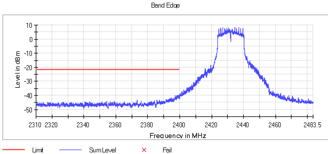
Graph 56: 2432 MHz Lower Band Edge Plot, Power Level 20
