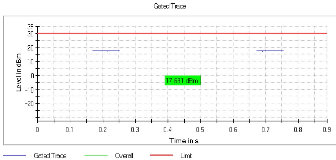
Graph 102: 2432 MHz Output Power Plot
