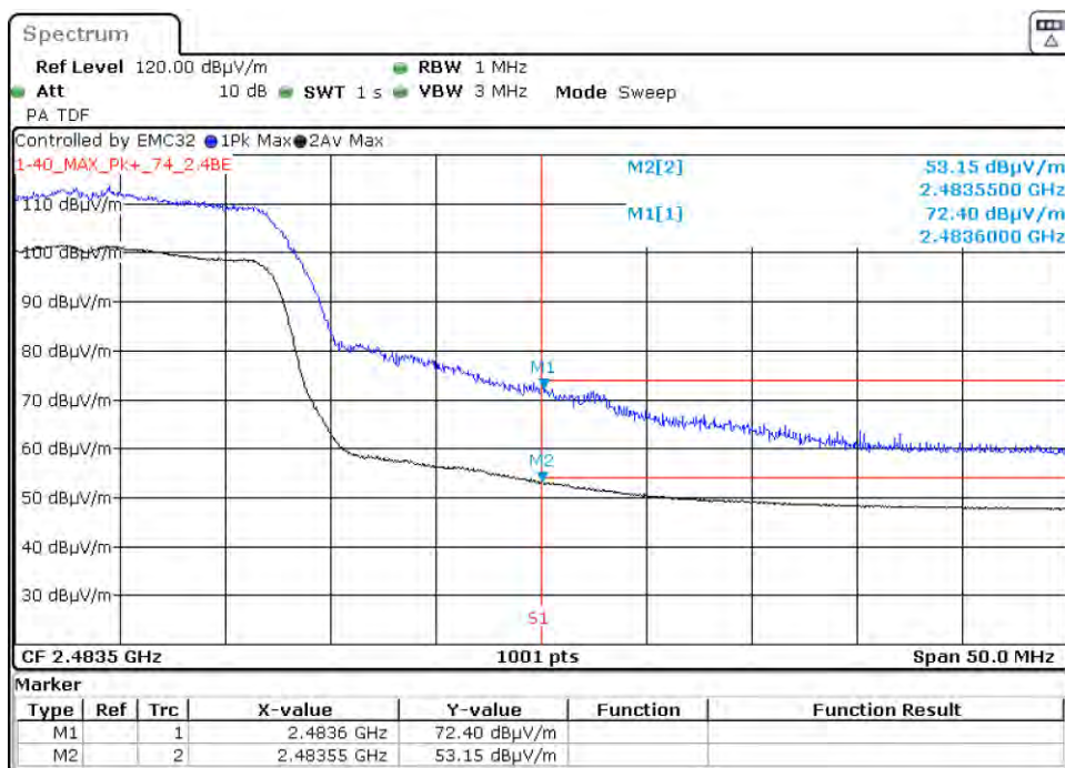
Graph 144: 2462 MHz Radiated Upper Band Edge Plot, Power Level 14 (C4-T5IW11)
