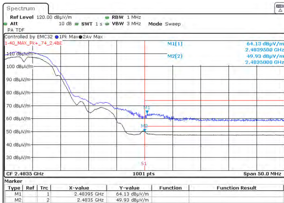
Graph 27: 2462 MHz Radiated Upper Band Edge Plot, Power Level 16 (C4-T5IW11)
