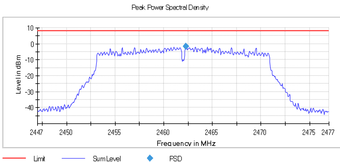
Graph 155: 2462 MHz 100 kHz PSD Plot
