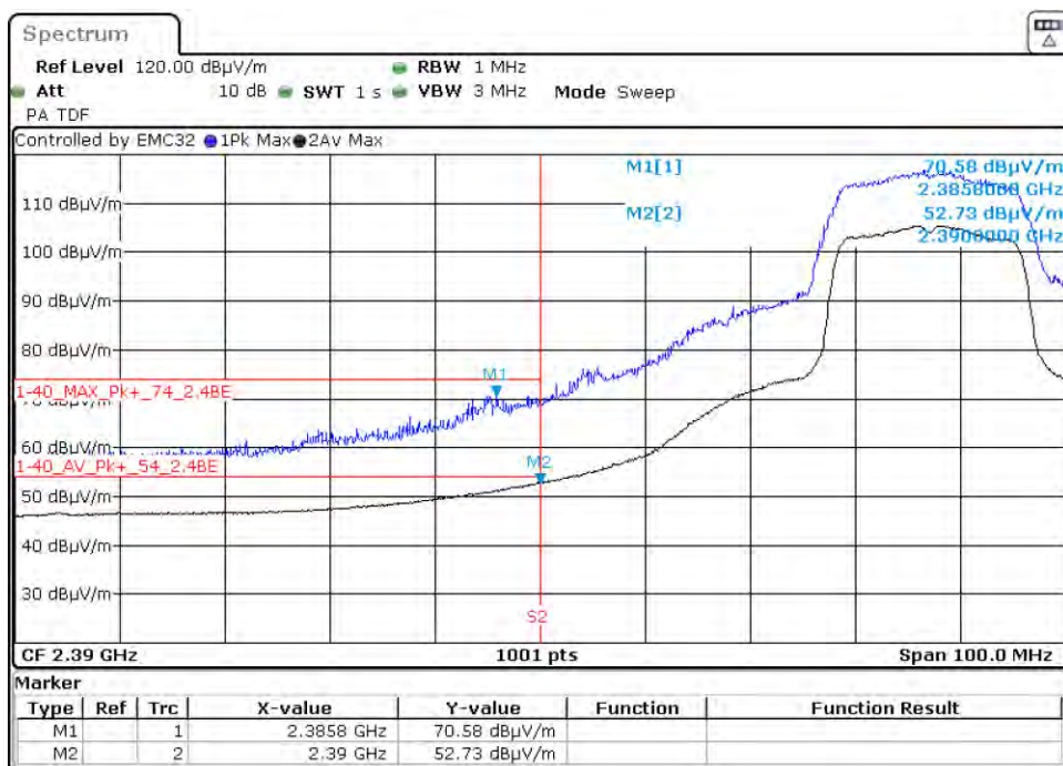
Graph 127: 2427 MHz Radiated Lower Band Edge Plot, Power Level 18 (C4-T5IW8)
