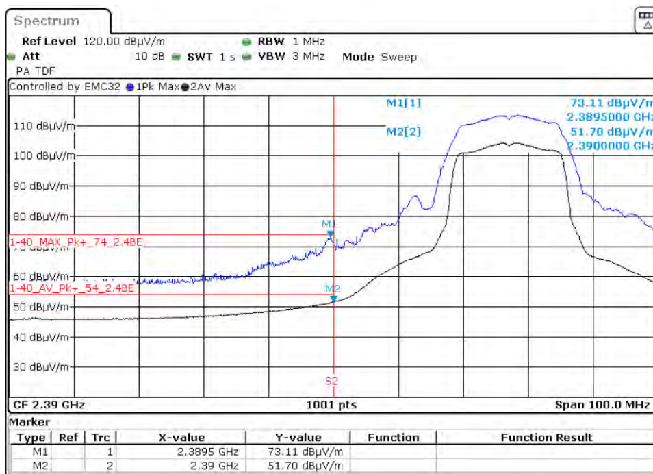
Graph 74: 2417 MHz Radiated Lower Band Edge Plot, Power Level 15 (C4-T5IW11)
