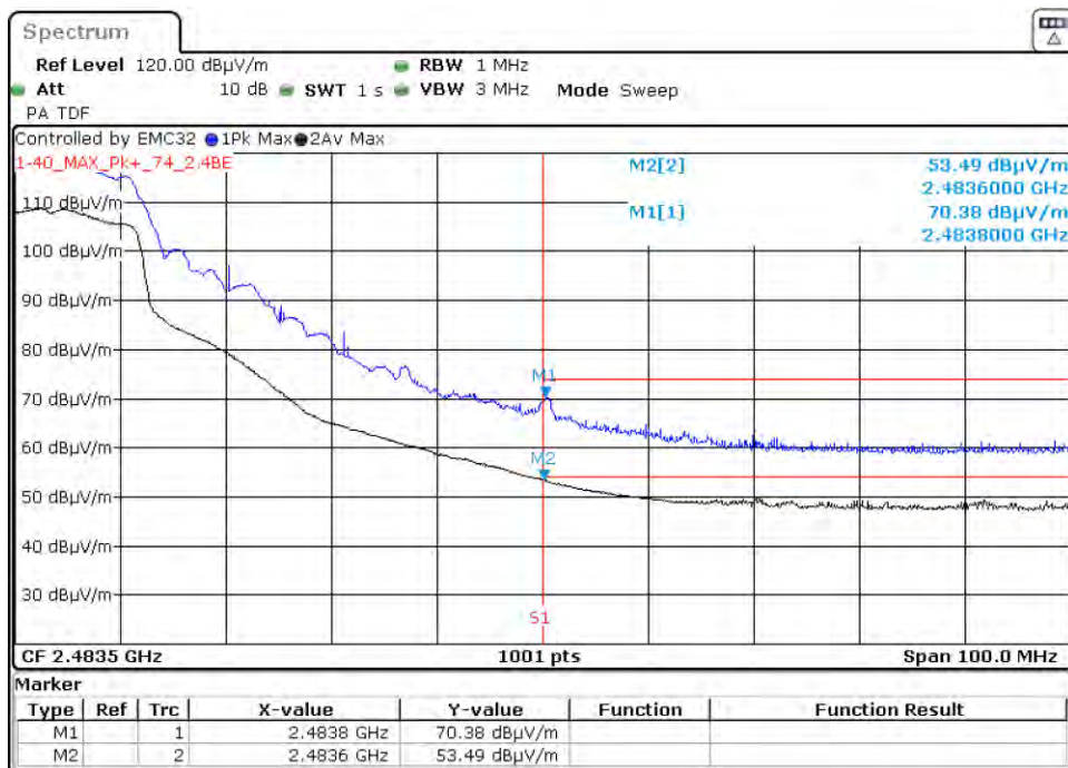
Graph 78: 2437 MHz Radiated Upper Band Edge Plot, Power Level 20 (C4-T5IW11)
