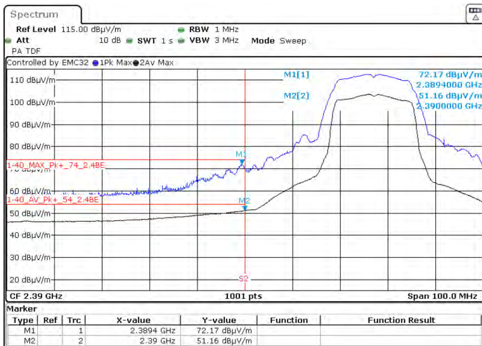
Graph 64: 2417 MHz Radiated Lower Band Edge Plot, Power Level 15 (C4-T5IW8)
