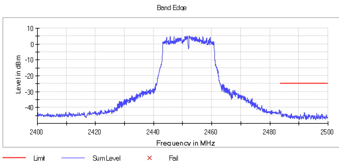
Graph 121: 2452 MHz Upper Band Edge Plot, Power Level 16
