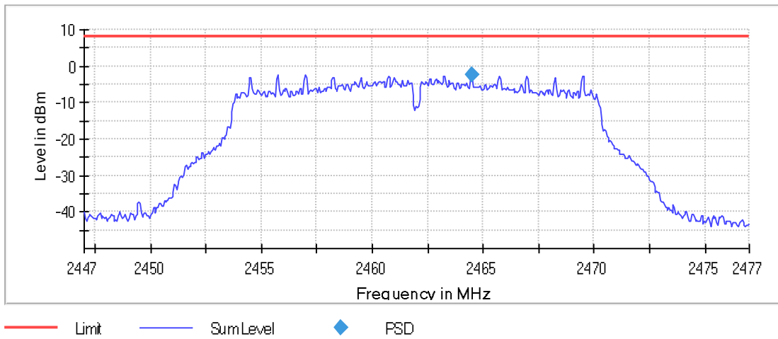
Graph 94: 2462 MHz 100 kHz PSD Plot
