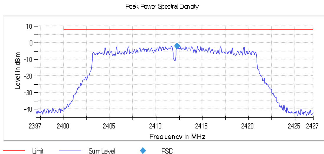
Graph 145: 2412 MHz 100 kHz PSD Plot
