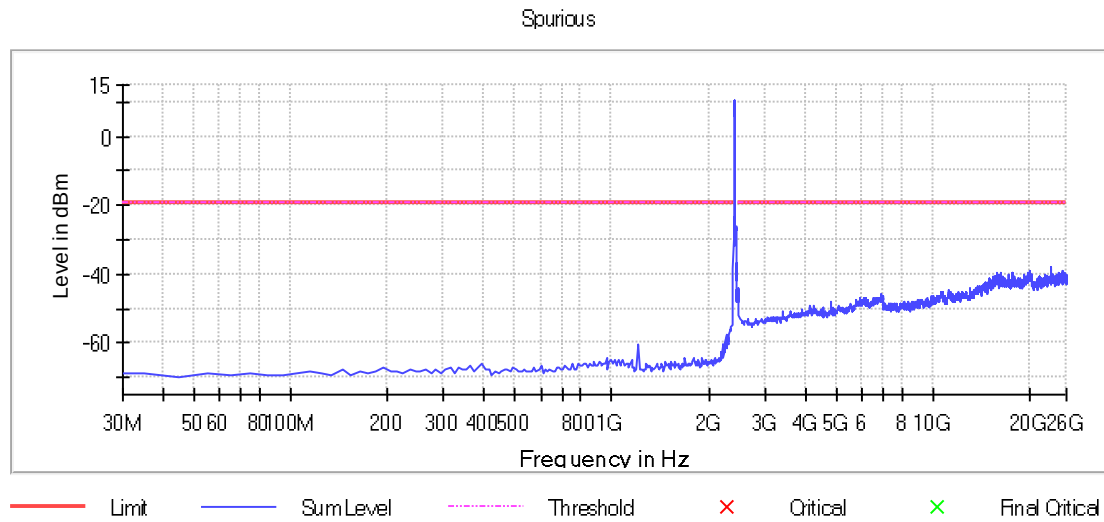
Graph 10: Transmitting on the Lowest Channel, Power Level 20
