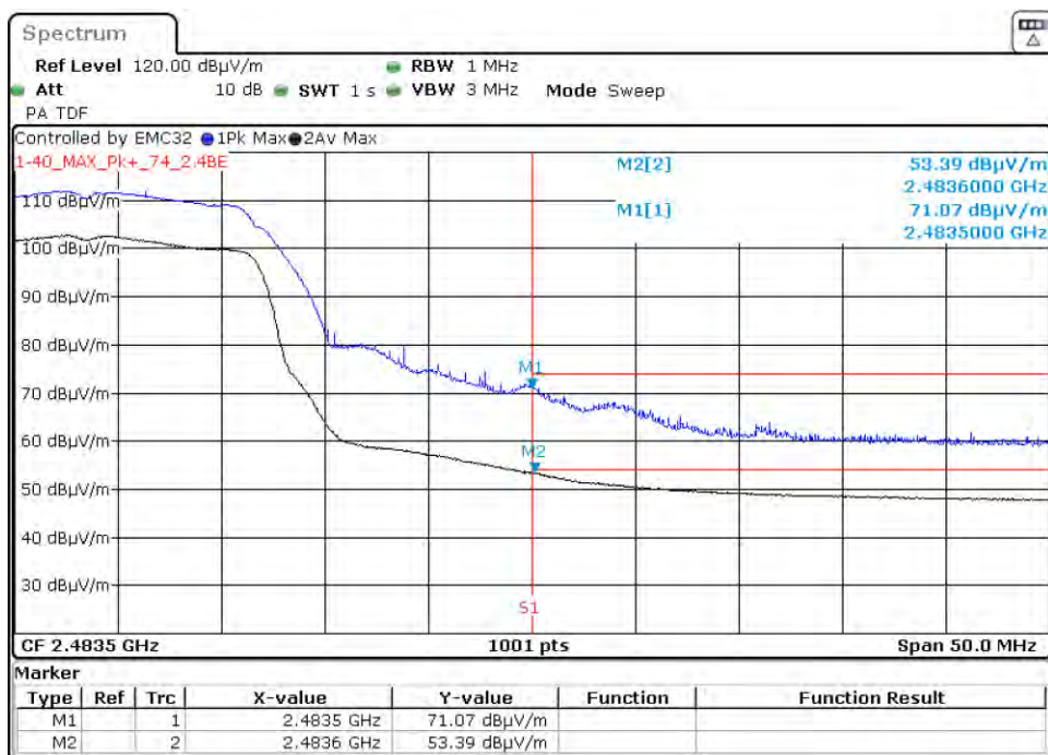
Graph 83: 2462 MHz Radiated Upper Band Edge Plot, Power Level 13 (C4-T5IW11)
