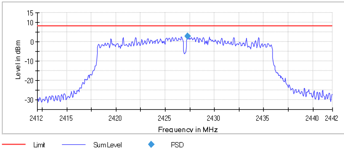
Graph 148: 2427 MHz 100 kHz PSD Plot
