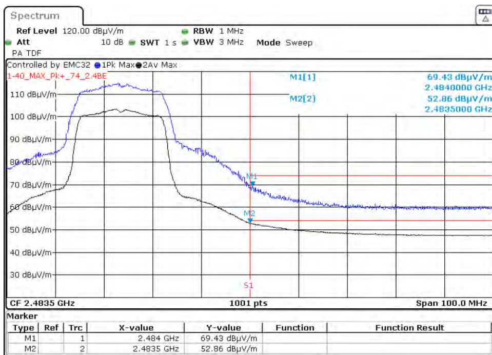
Graph 132: 2457 MHz Radiated Upper Band Edge Plot, Power Level 16 (C4-T5IW8)
