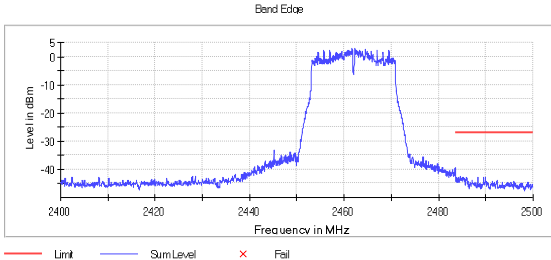
Graph 123: 2462 MHz Upper Band Edge Plot, Power Level 13
