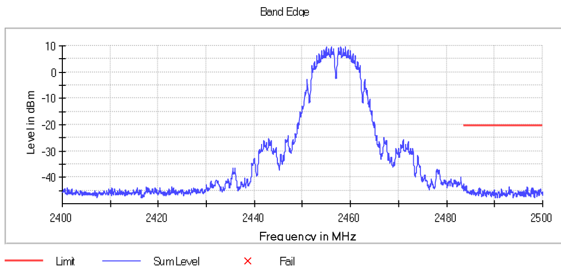
Graph 16: 2457 MHz Upper Band Edge Plot, Power Level 18
