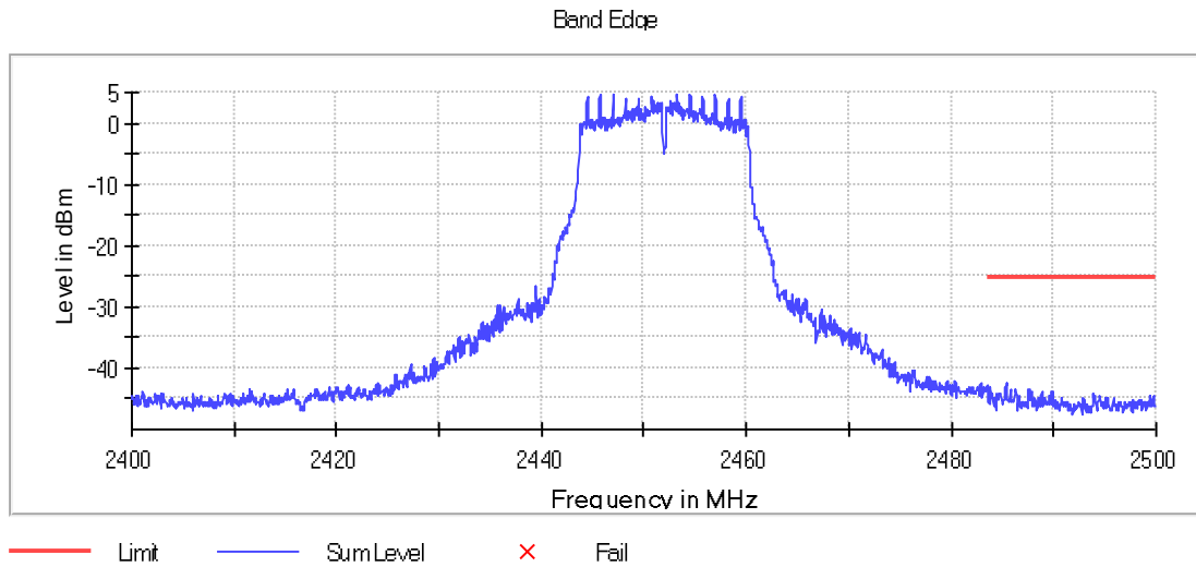
Graph 60: 2452 MHz Upper Band Edge Plot, Power Level 16
