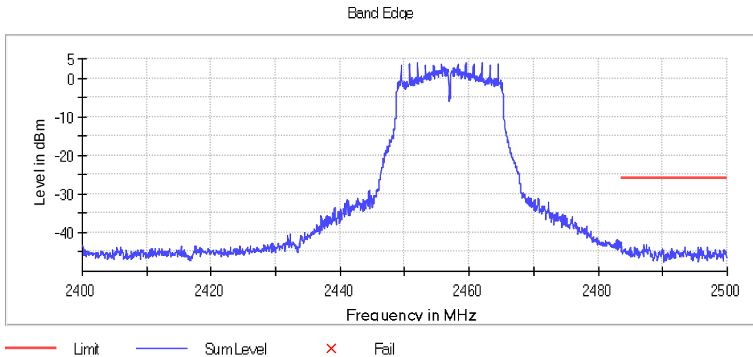
Graph 61: 2457 MHz Upper Band Edge Plot, Power Level 15
