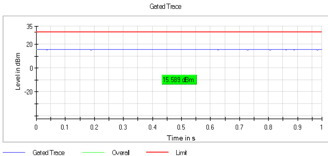
Graph 44: 2447 MHz Output Power Plot
