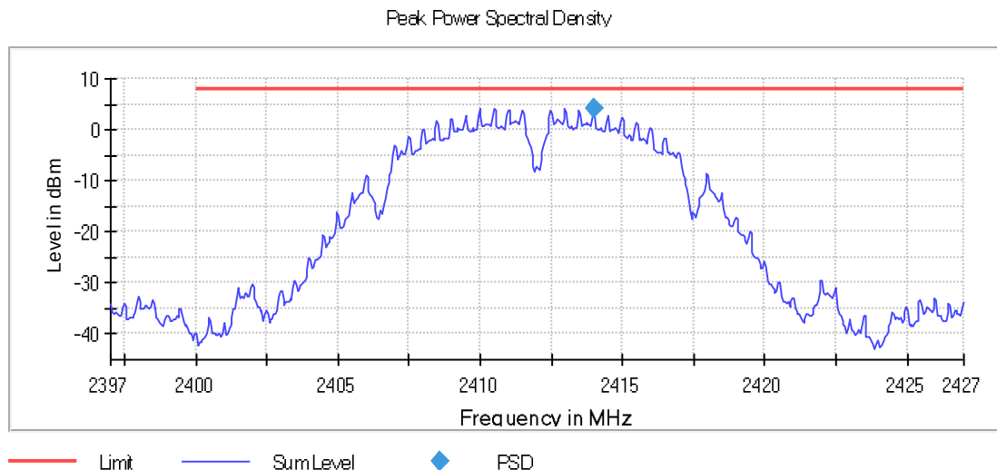
Graph 28: 2412 MHz 100 kHz PSD Plot
