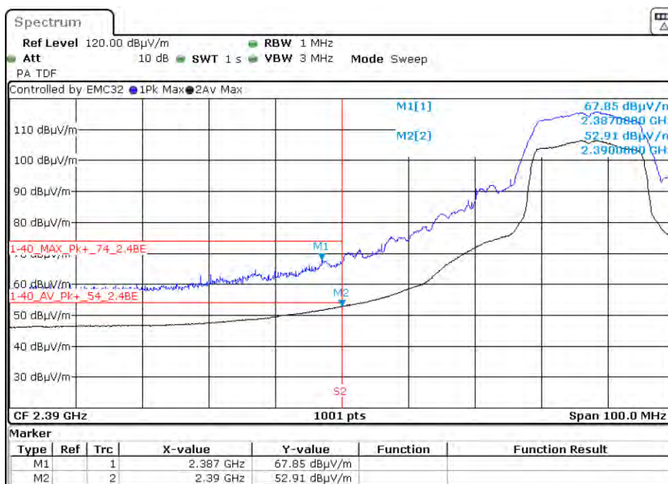
Graph 66: 2427 MHz Radiated Lower Band Edge Plot, Power Level 17 (C4-T5IW8)
