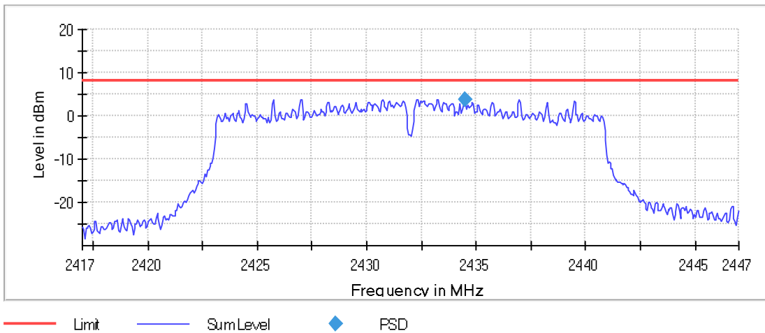
Graph 149: 2432 MHz 100 kHz PSD Plot
