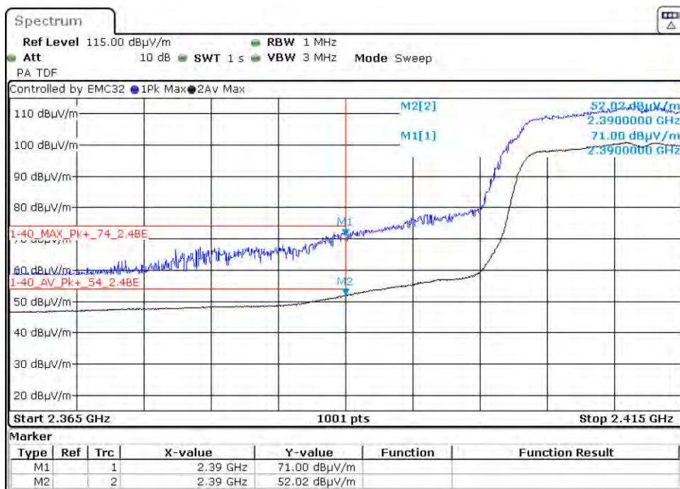
Graph 124: 2412 MHz Radiated Lower Band Edge Plot, Power Level 13 (C4-T5IW8)
