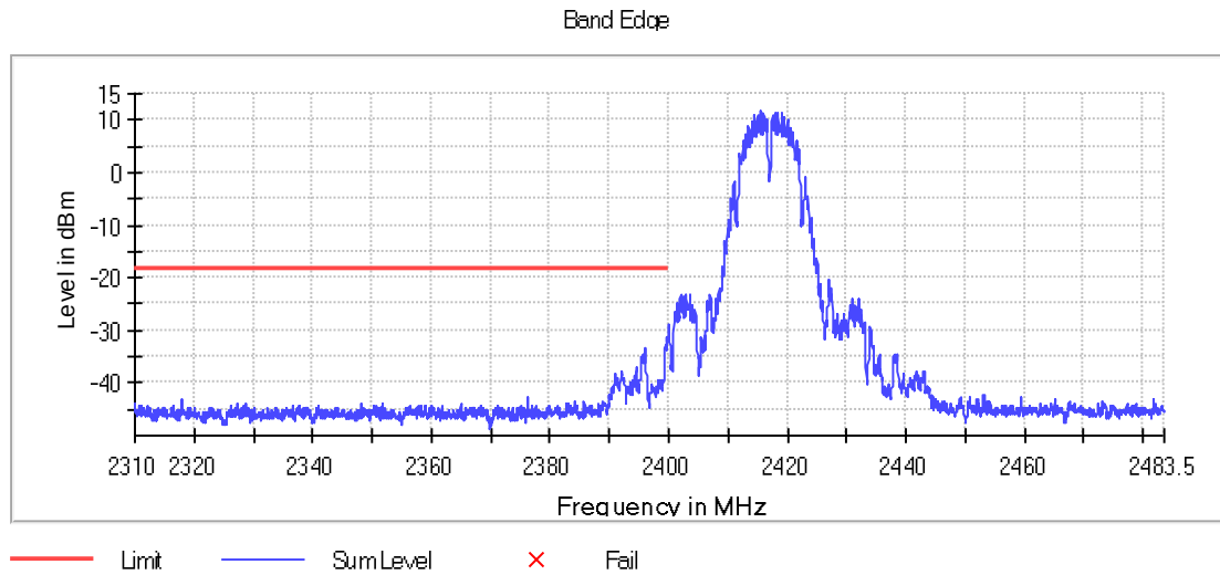
Graph 14: 2417 MHz Lower Band Edge Plot, Power Level 20
