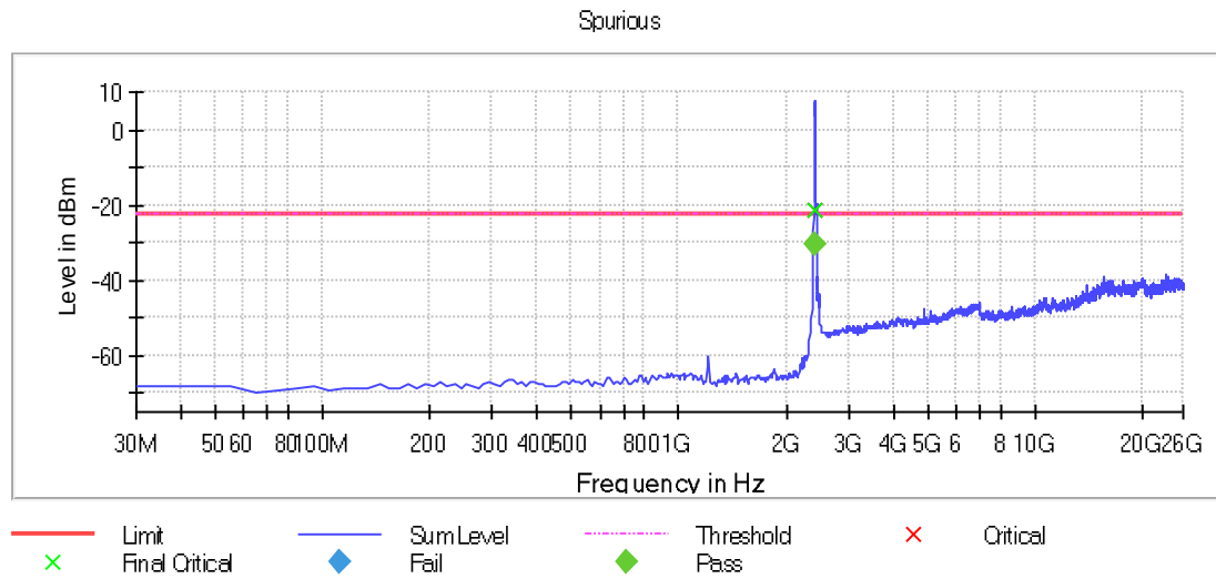
Graph 109: Transmitting on the Lowest Channel, Power Level 20
