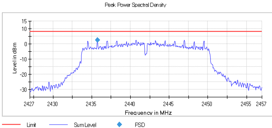
Graph 90: 2442 MHz 100 kHz PSD Plot
