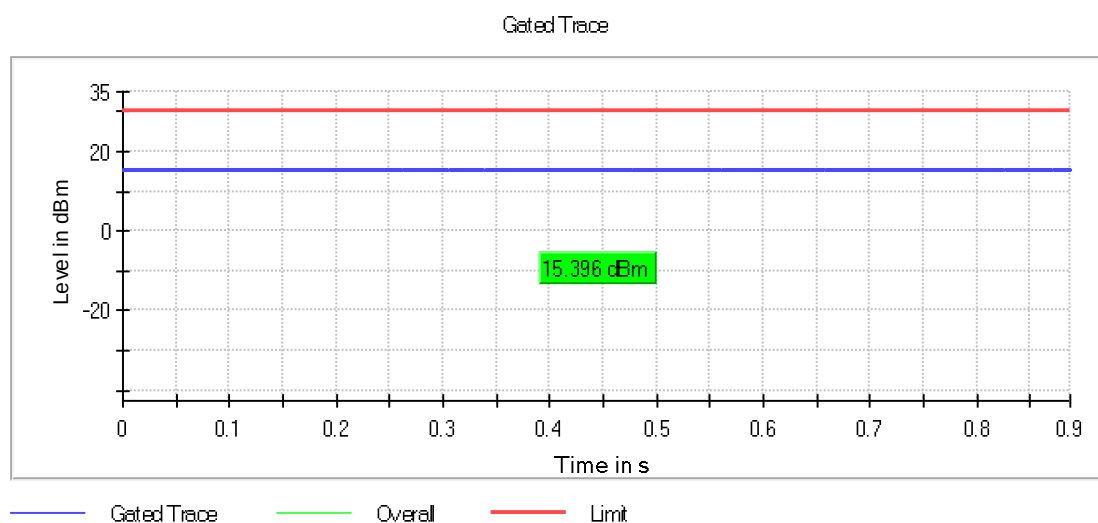
Graph 105: 2447 MHz Output Power Plot
