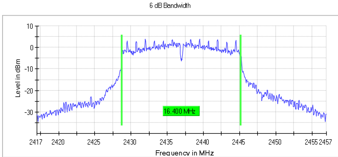
Graph 35: Middle Channel Bandwidth
