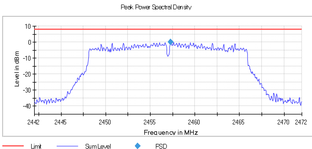
Graph 154: 2457 MHz 100 kHz PSD Plot
