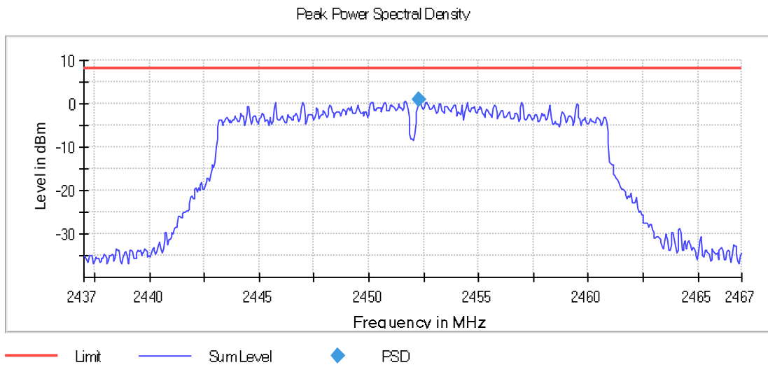
Graph 153: 2452 MHz 100 kHz PSD Plot
