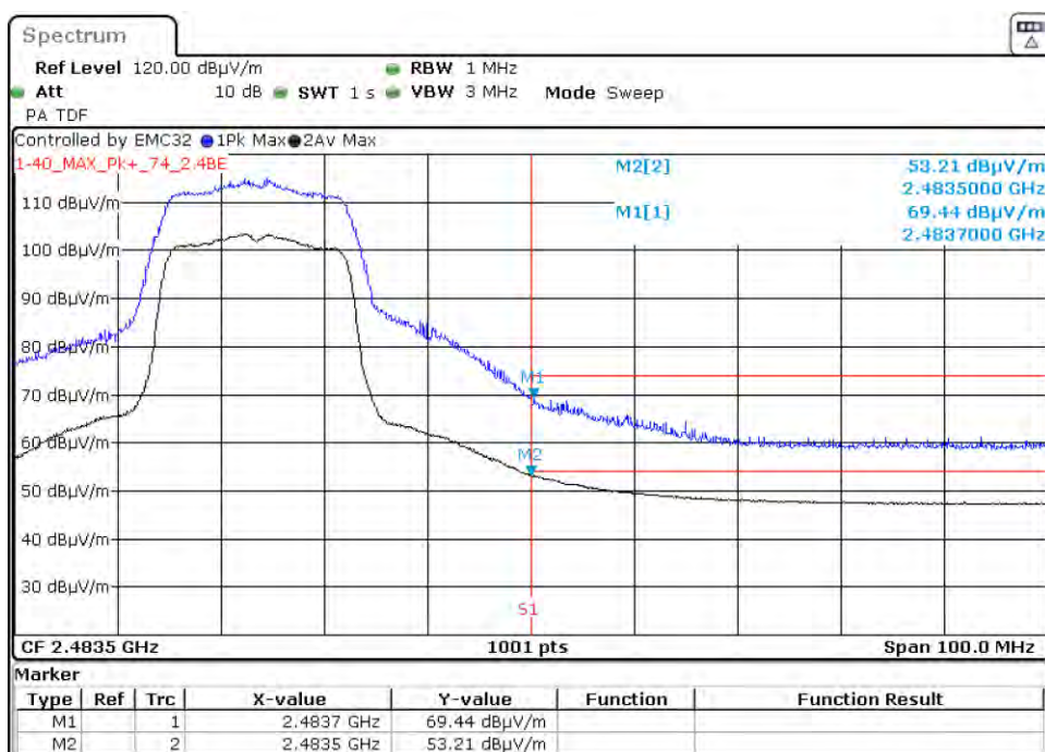
Graph 143: 2457 MHz Radiated Upper Band Edge Plot, Power Level 15 (C4-T5IW11)
