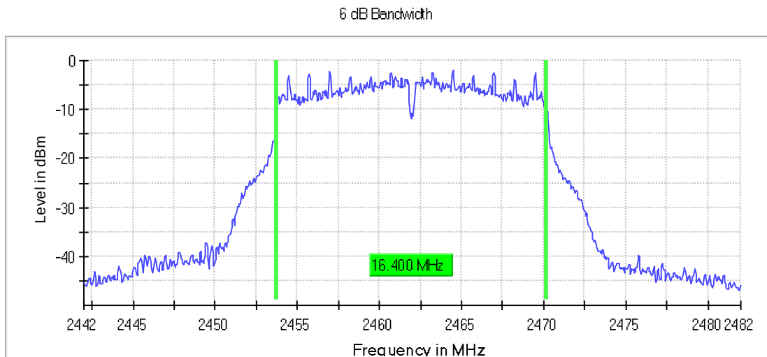
Graph 36: Highest Channel Bandwidth
