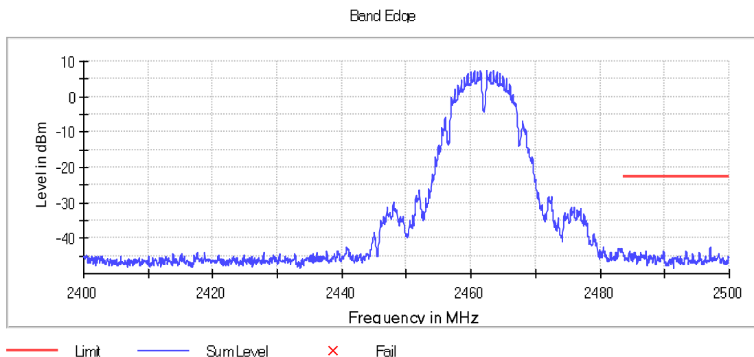
Graph 17: 2462 MHz Upper Band Edge Plot, Power Level 16
