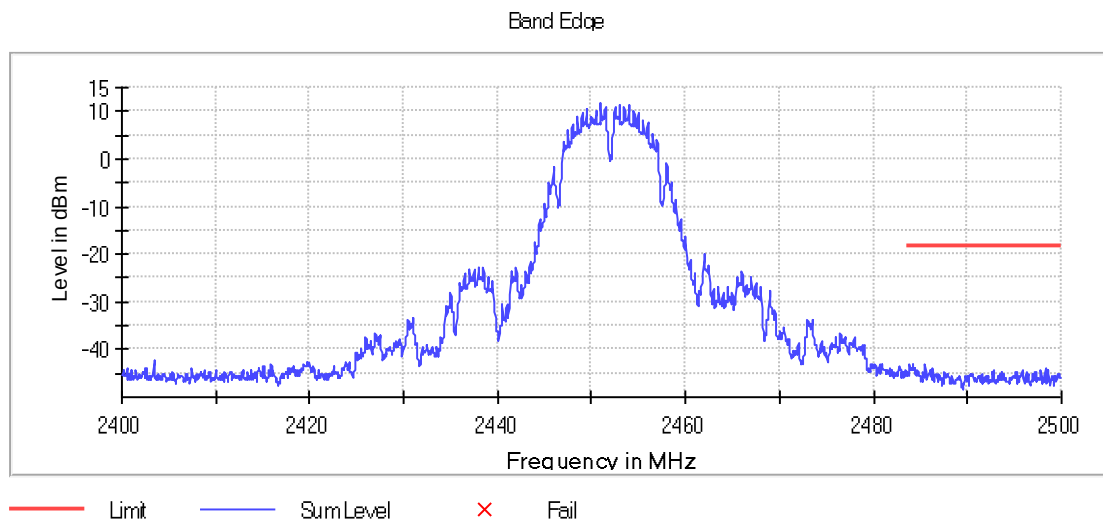
Graph 15: 2452 MHz Upper Band Edge Plot, Power Level 20
