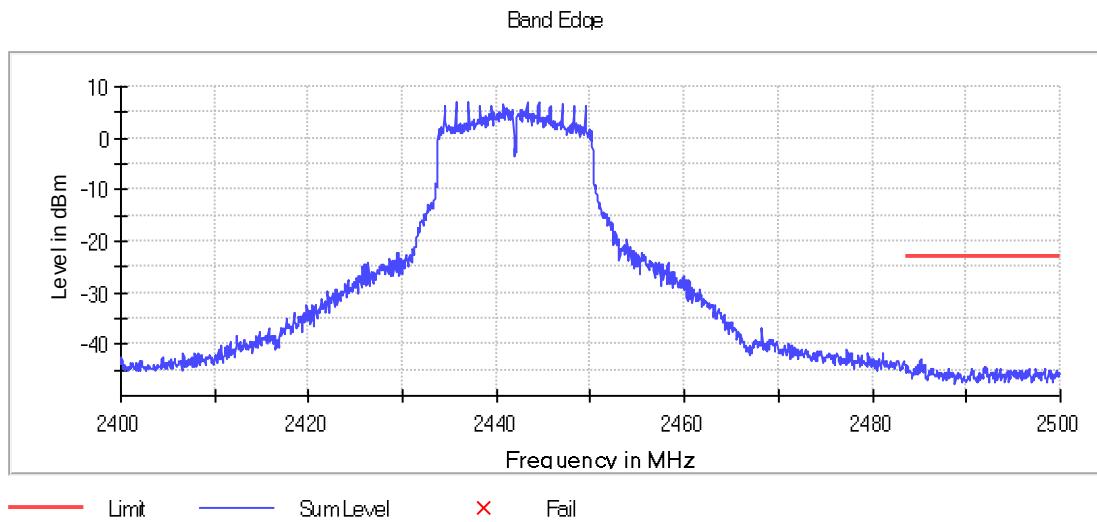
Graph 58: 2442 MHz Upper Band Edge Plot, Power Level 18
