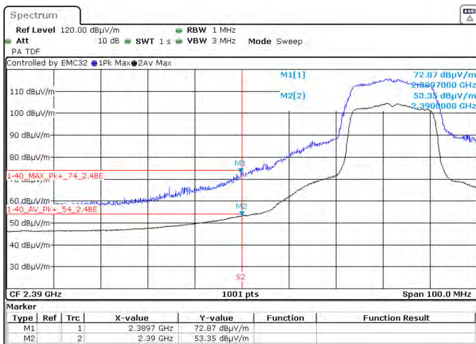
Graph 126: 2422 MHz Radiated Lower Band Edge Plot, Power Level 17 (C4-T5IW8)
