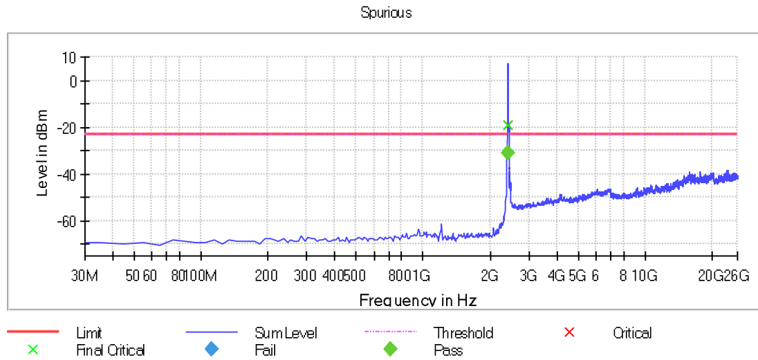
Graph 48: Transmitting on the Lowest Channel, Power Level 20
