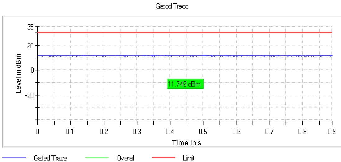
Graph 108: 2462 MHz Output Power Plot
