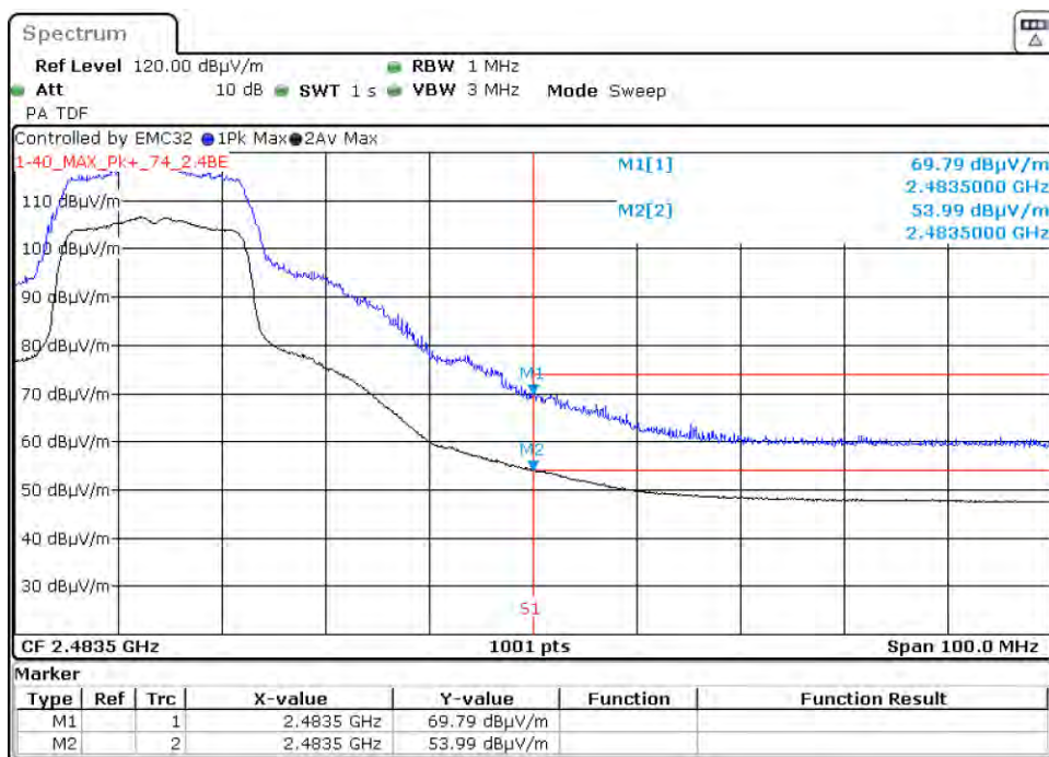
Graph 130: 2447 MHz Radiated Upper Band Edge Plot, Power Level 19 (C4-T5IW8)
