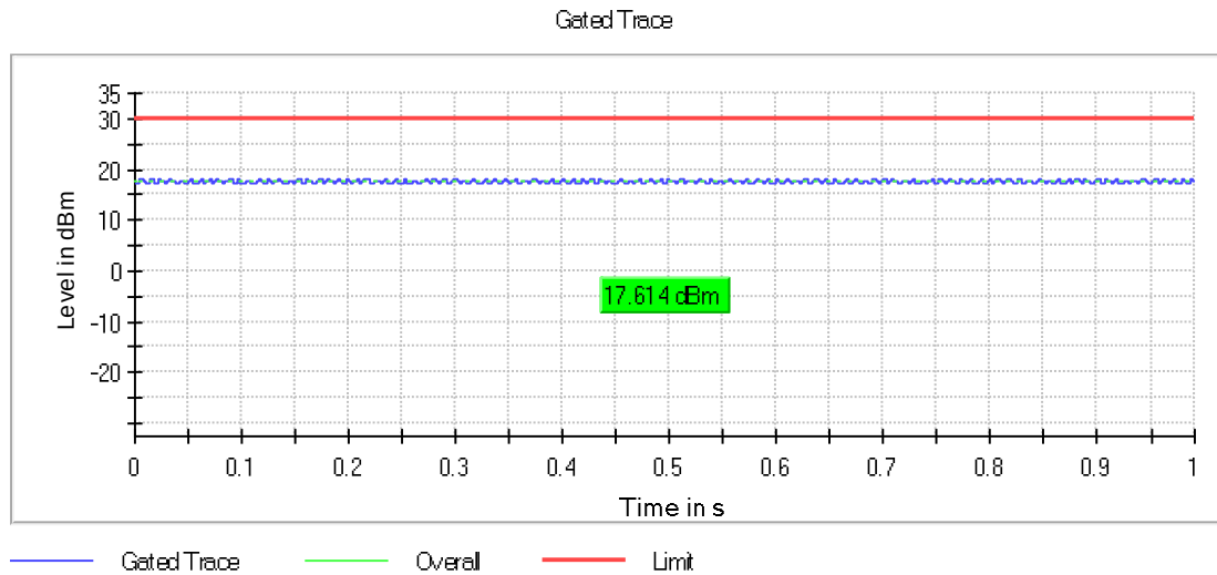
Graph 7: 2452 MHz Output Power Plot
