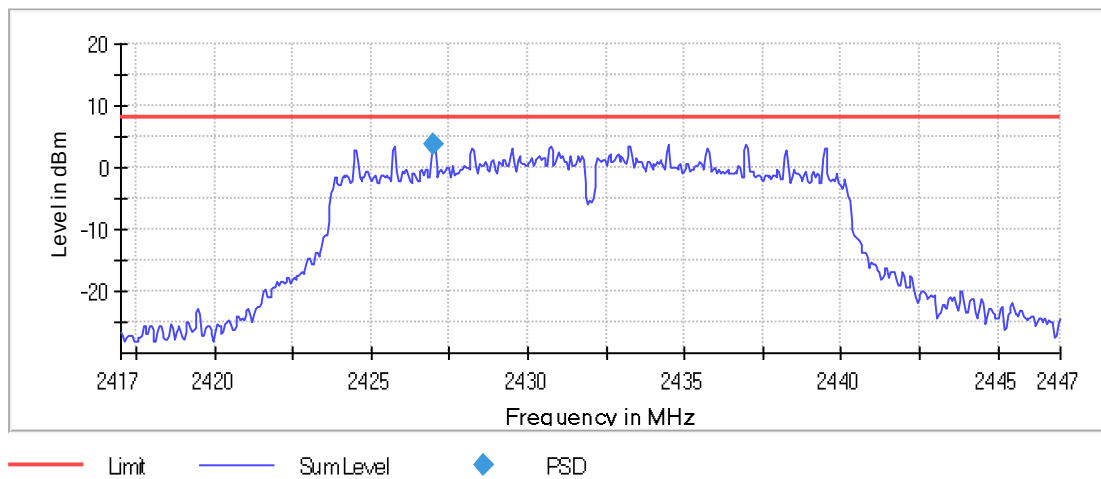
Graph 88: 2432 MHz 100 kHz PSD Plot
