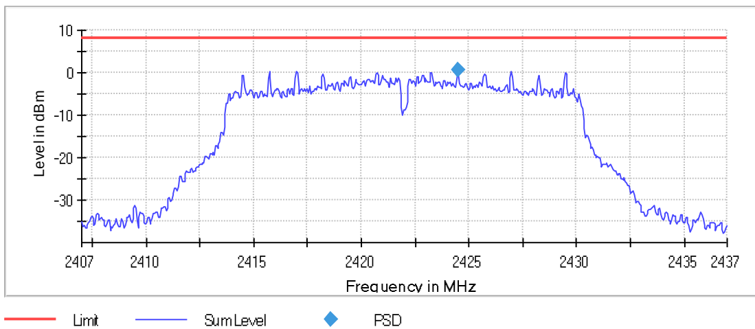
Graph 86: 2422 MHz 100 kHz PSD Plot
