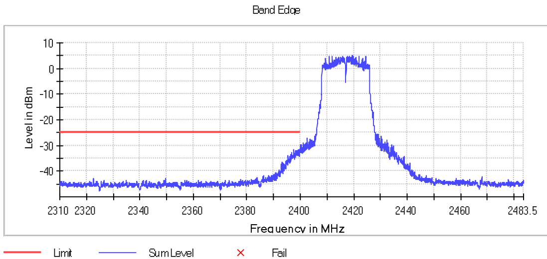
Graph 114: 2417 MHz Lower Band Edge Plot, Power Level 16
