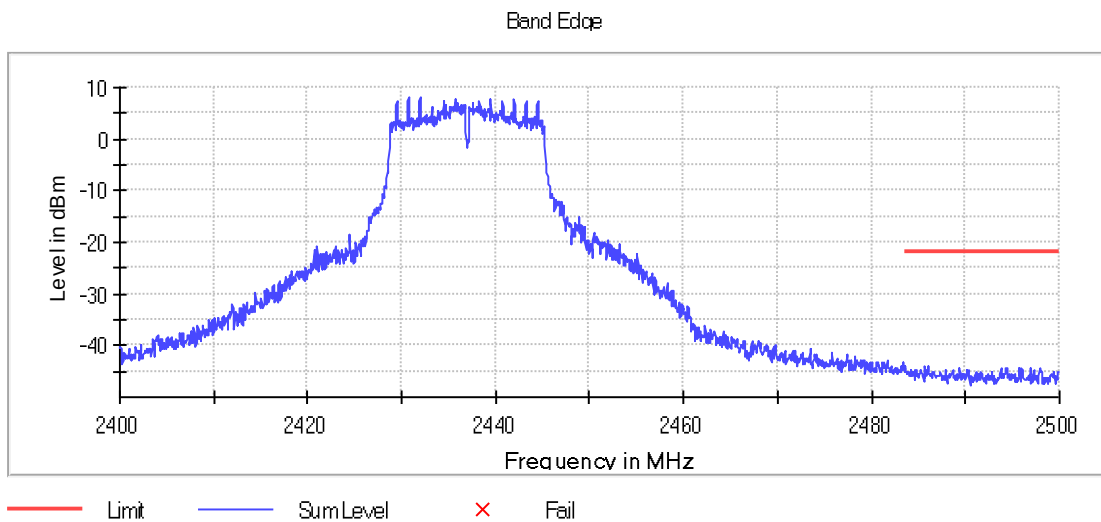
Graph 57: 2437 MHz Upper Band Edge Plot, Power Level 20
