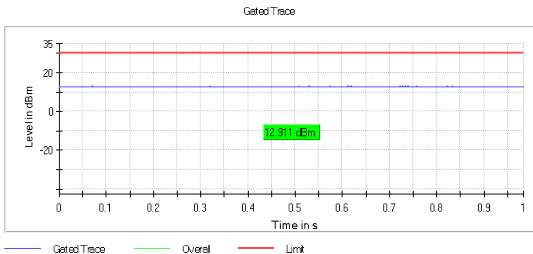
Graph 37: 2412 MHz Output Power Plot
