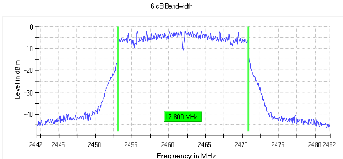
Graph 97: Highest Channel Bandwidth
