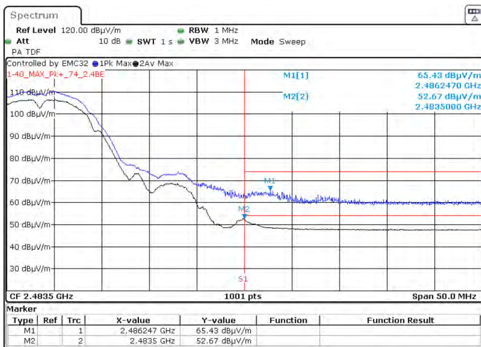
Graph 22: 2462 MHz Radiated Upper Band Edge Plot, Power Level 16 (C4-T5IW8)
