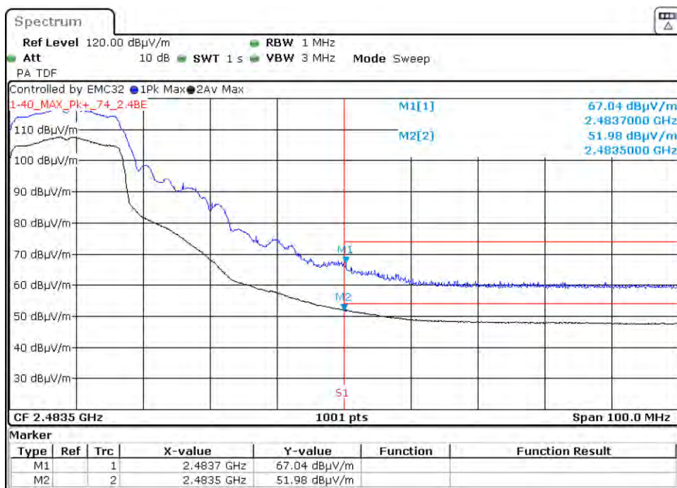
Graph 68: 2442 MHz Radiated Upper Band Edge Plot, Power Level 20 (C4-T5IW8)
