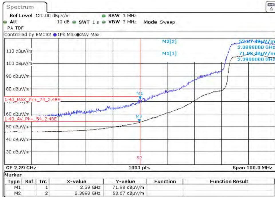
Graph 138: 2432 MHz Radiated Lower Band Edge Plot, Power Level 20 (C4-T5IW11)
