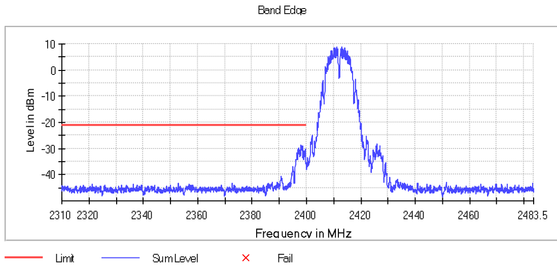
Graph 13: 2412 MHz Lower Band Edge Plot, Power Level 17
