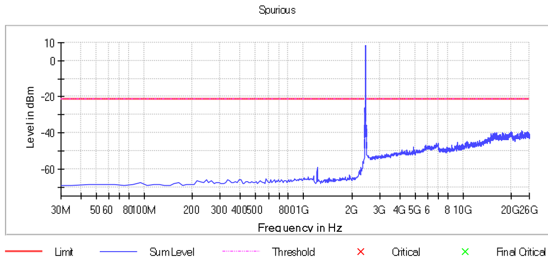
Graph 11: Transmitting on the Middle Channel, Power Level 20
