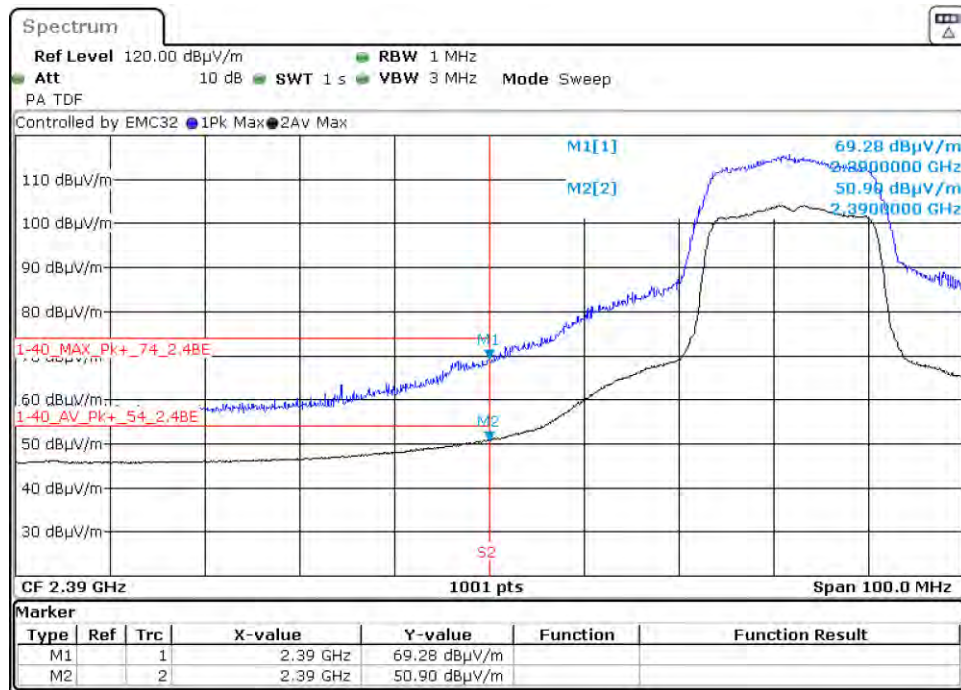
Graph 136: 2422 MHz Radiated Lower Band Edge Plot, Power Level 16 (C4-T5IW11)
