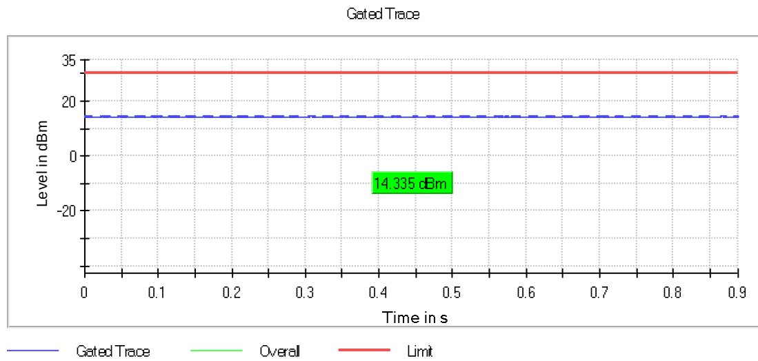
Graph 100: 2422 MHz Output Power Plot
