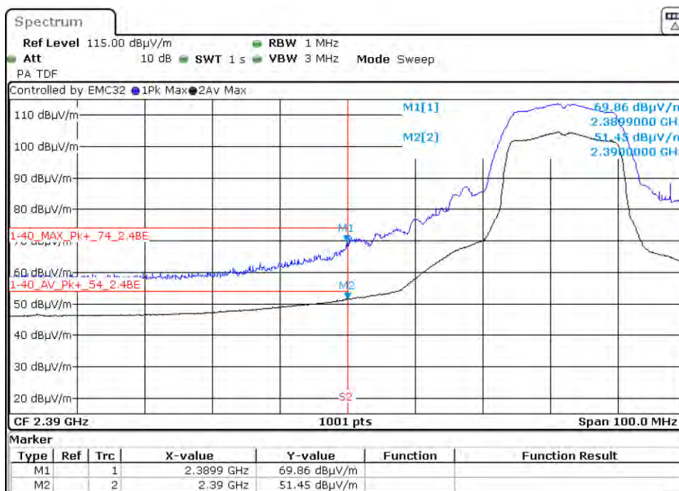
Graph 65: 2422 MHz Radiated Lower Band Edge Plot, Power Level 16 (C4-T5IW8)
