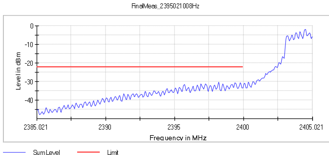
Graph 110: Critical Point (2395.021 MHz) Transmitting on the Lowest Channel, Power Level 20
