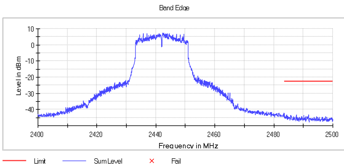
Graph 119: 2442 MHz Upper Band Edge Plot, Power Level 18
