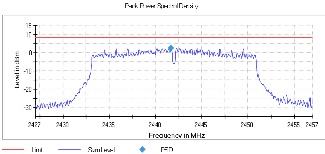
Graph 151: 2442 MHz 100 kHz PSD Plot
