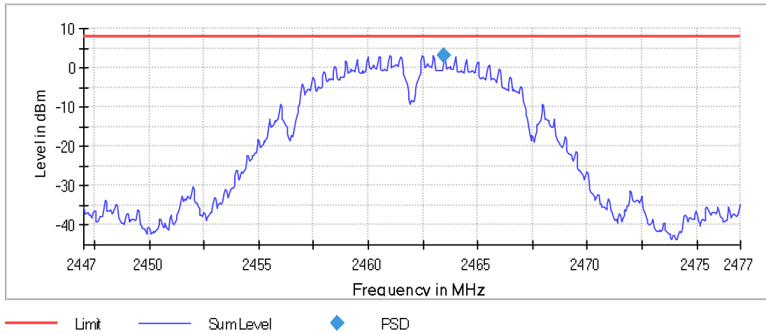
Graph 33: 2462 MHz Output 100 kHz PSD Plot
