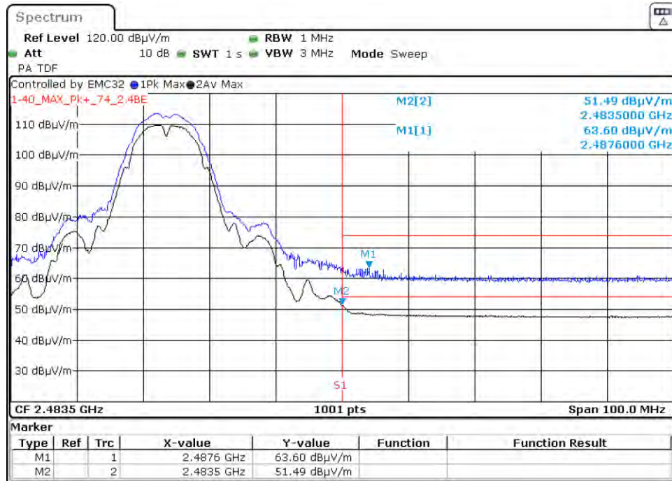
Graph 26: 2457 MHz Radiated Upper Band Edge Plot, Power Level 18 (C4-T5IW11)
