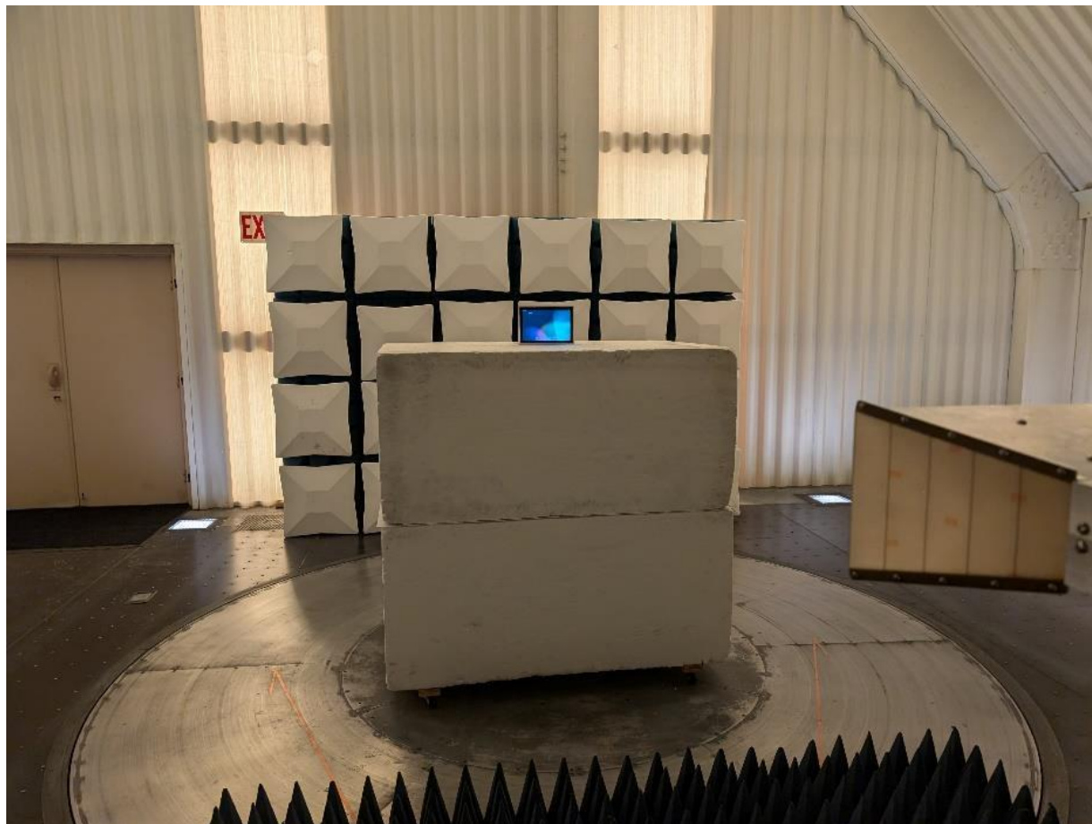
Photograph 1: Front View Radiated Emissions Worst Case Configuration, T5IW11
