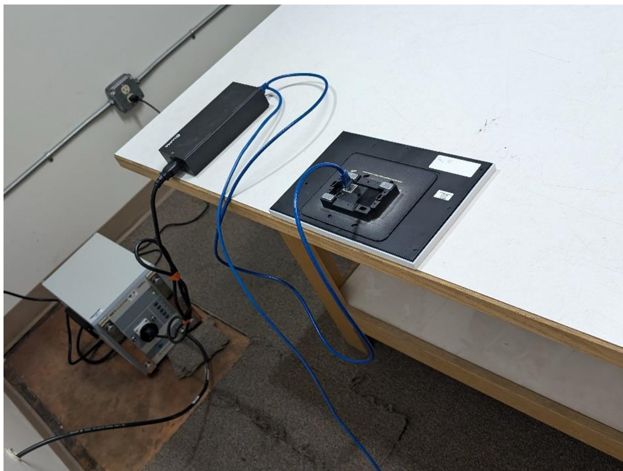
Photograph 4: Back View Conducted Emissions Worst-Case Configuration, T5IW11
