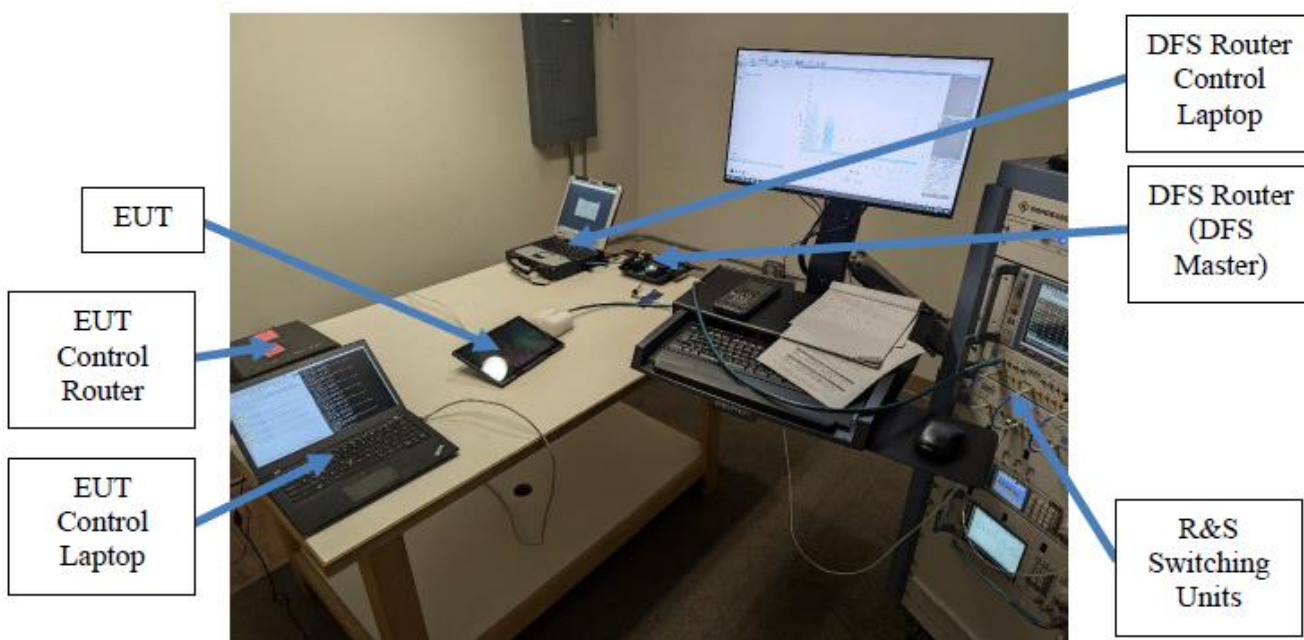
Photograph 6: DFS Test Setup, T5IW11
