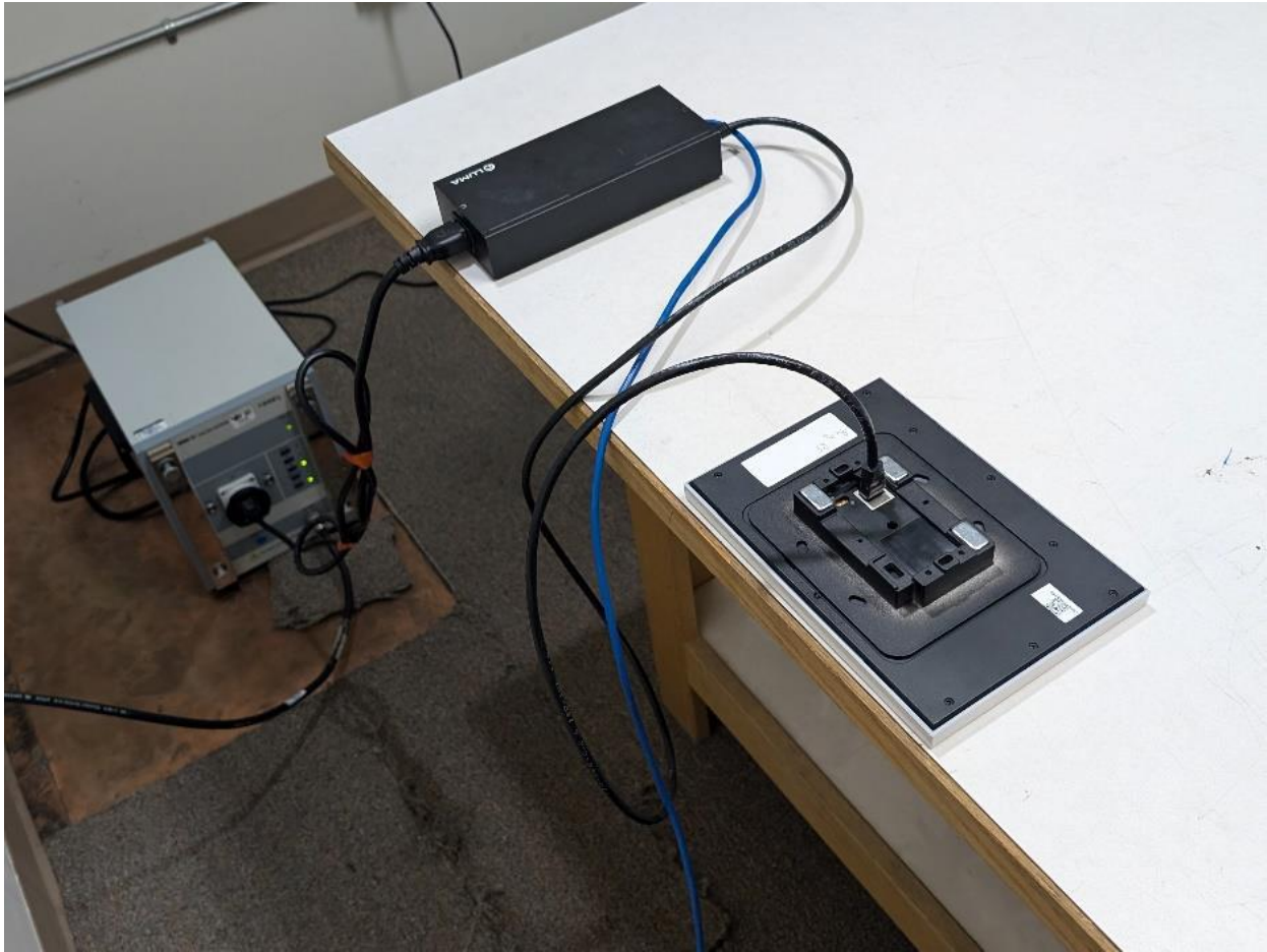
Photograph 4: Back View Conducted Emissions Worst-Case Configuration, T5IW8
