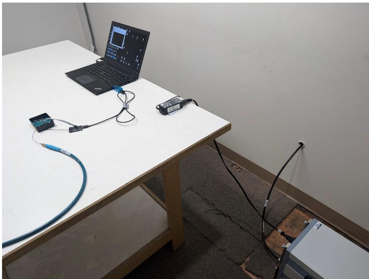
Photograph 7: Front View Conducted Emissions Worst-Case Configuration, C4-Z2C-V3
