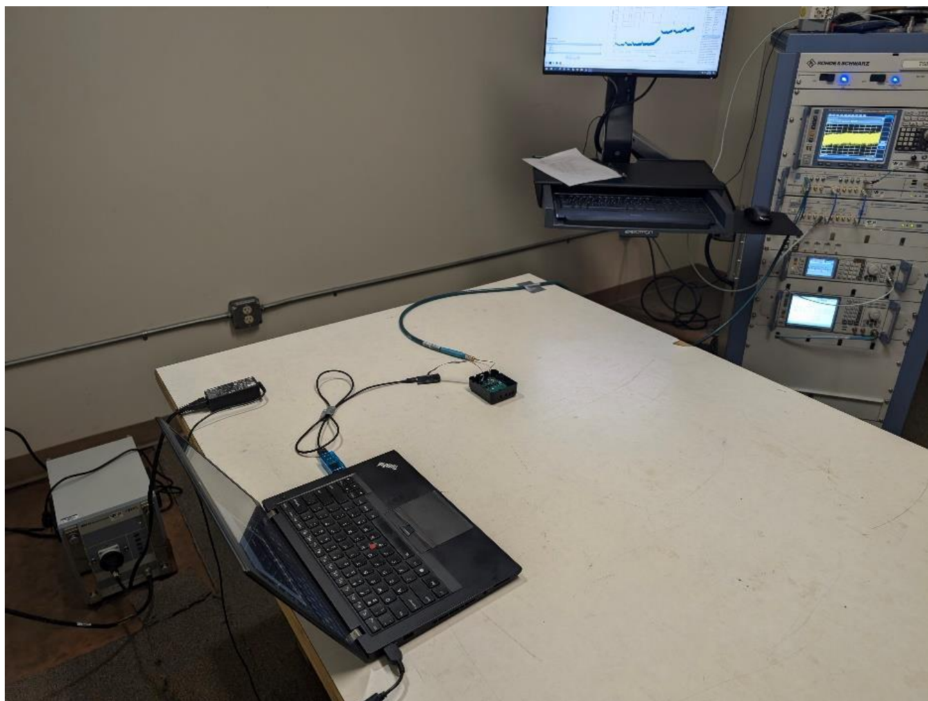
Photograph 6: View of Antenna Port Test Setup, C4-Z2C-V3
