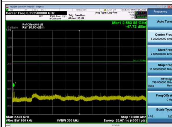
8DPSK,2480MHz,3DH5,Plot 3,2505MHz~10000MHz
