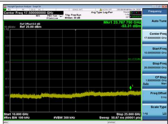
8DPSK,2480MHz,3DH5,Plot 4,10000MHz~25000MHz
