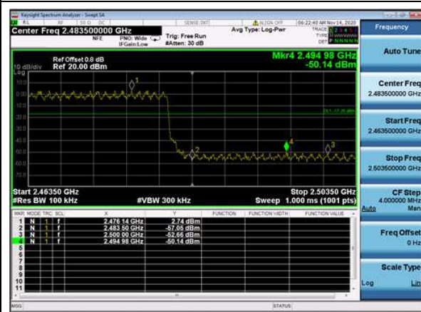
8DPSK,Hopping,3DH5,Band Edge HighRange
