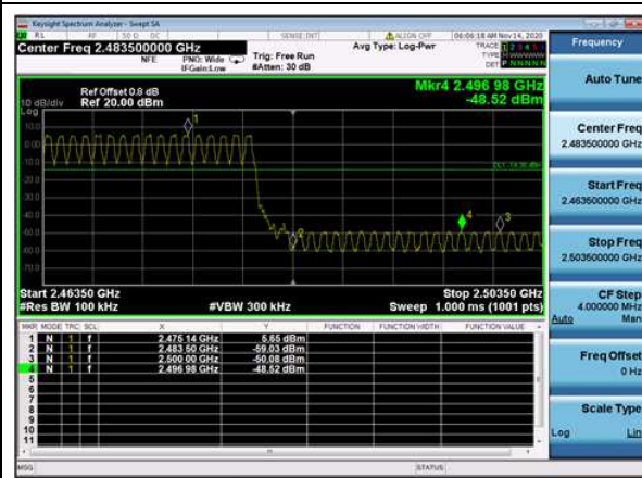
DQPSK,Hopping,2DH5,Band Edge HighRange
