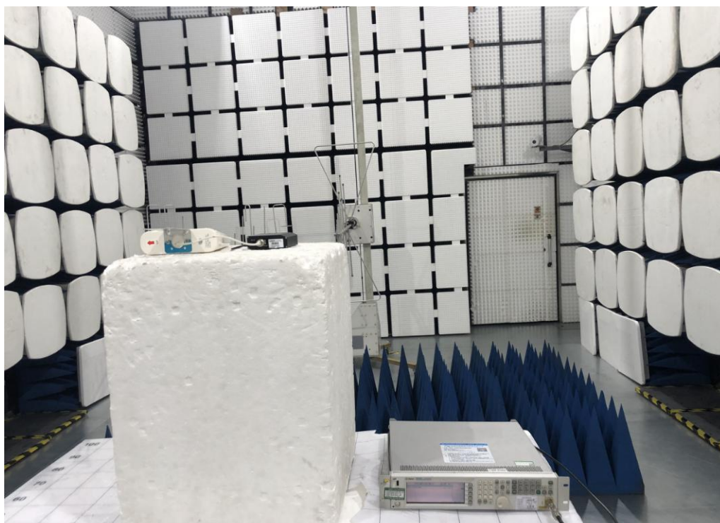
Fig. 1 (Below 1GHz)-SYN-BY-9D
