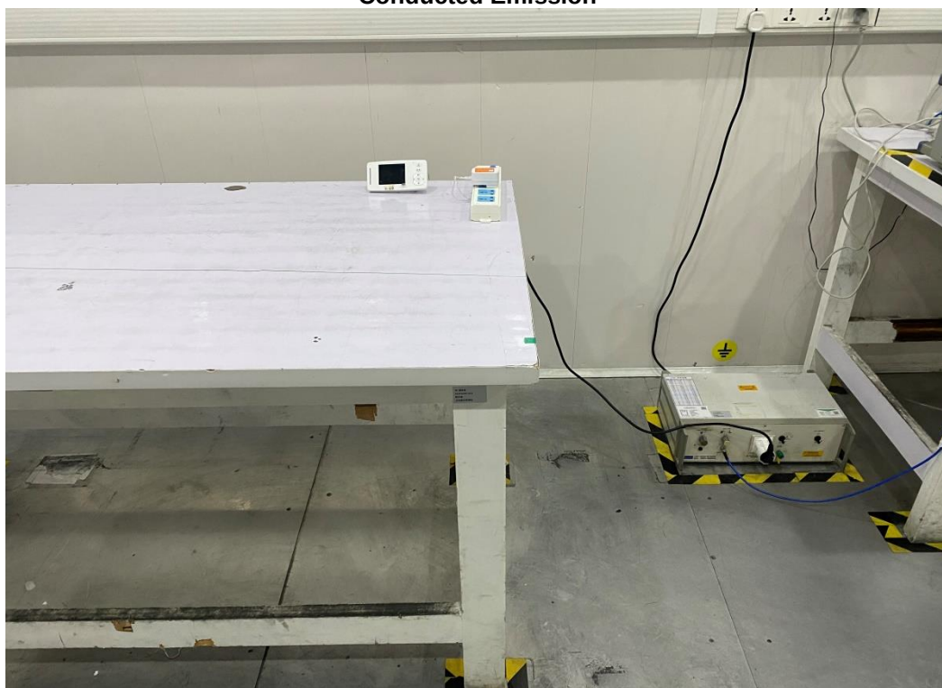
Conducted Emission
