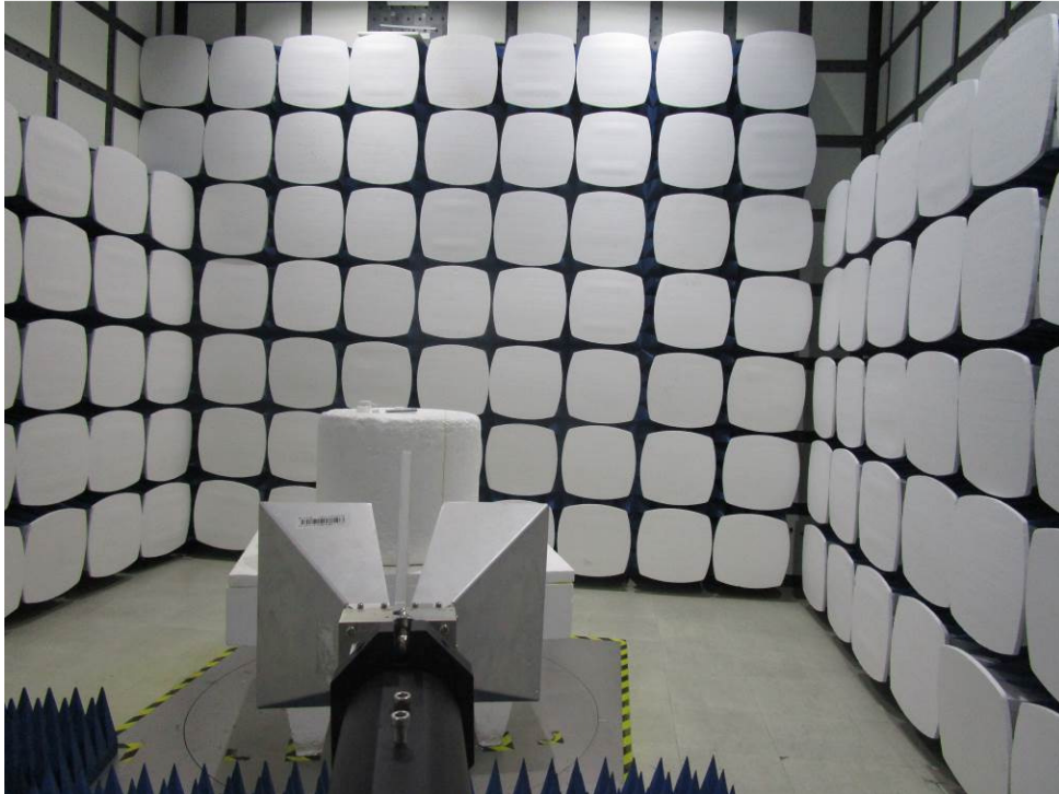
1.3 Radiated Emissions which fall in the restricted bands Test Setup
