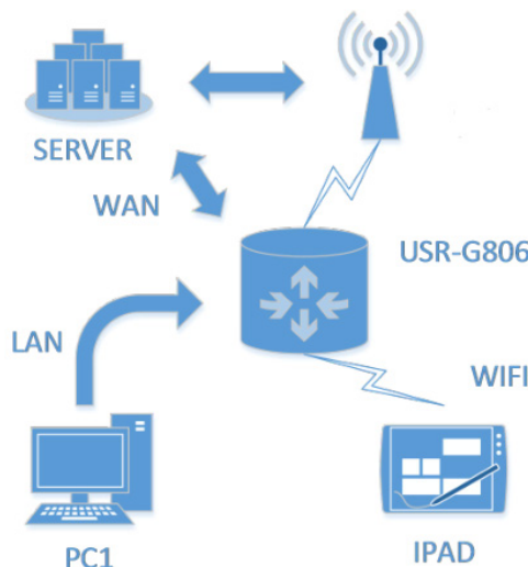
Figure 5 WAN+LAN+4G networking
