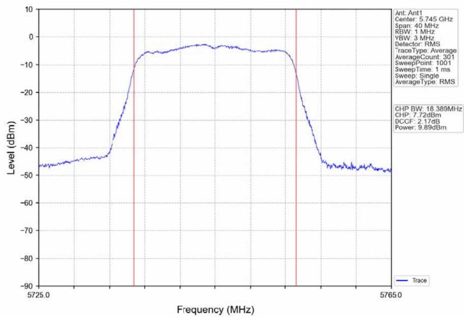
802.11ac(VHT20)_LCH_5745MHz_Ant1_NTNV
