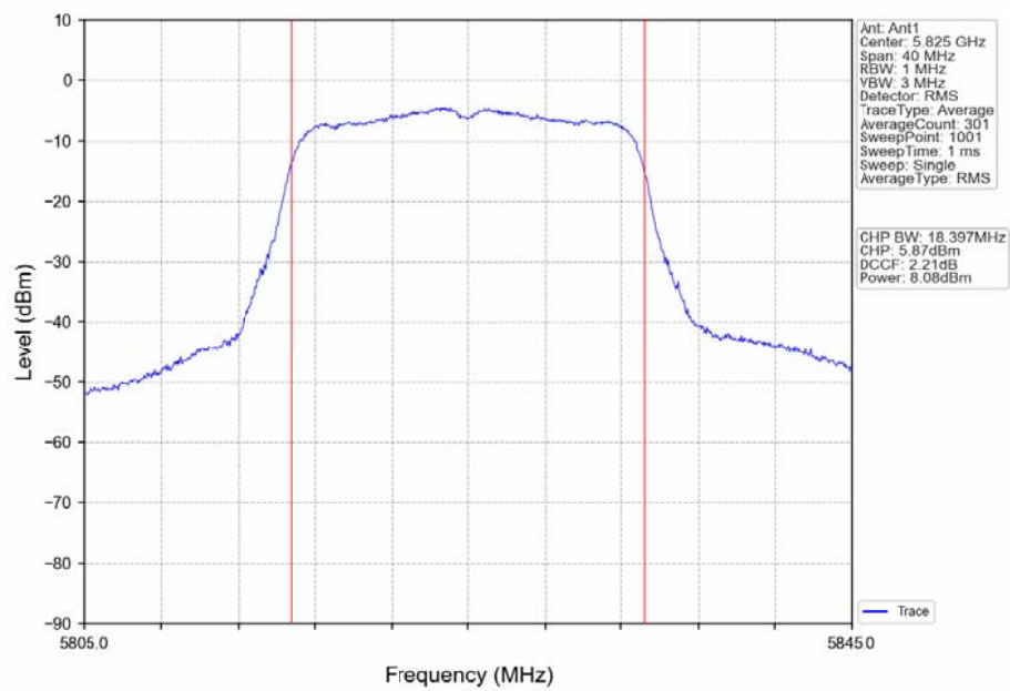
802.11ac(VHT20)_HCH_5825MHz_Ant1_NTNV
