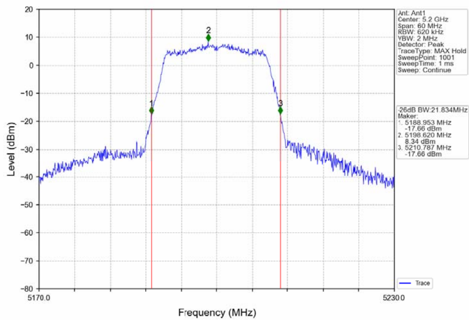
802.11ac(VHT20)_MCH_5200MHz_Ant1_NTNV
