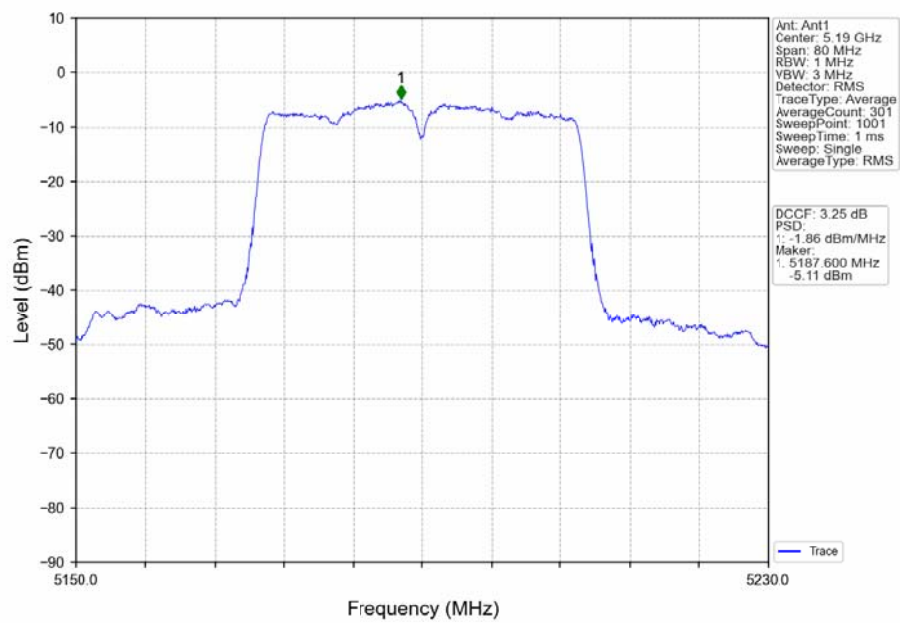
802.11ac(VHT40)_LCH_5190MHz_Ant1_NTNV
