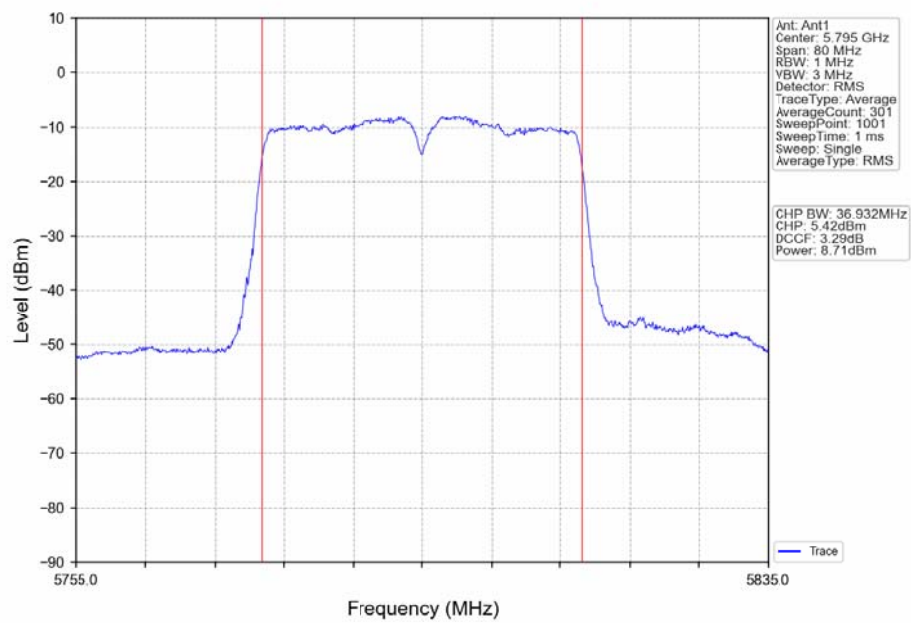
802.11ac(VHT40)_HCH_5795MHz_Ant1_NTNV
