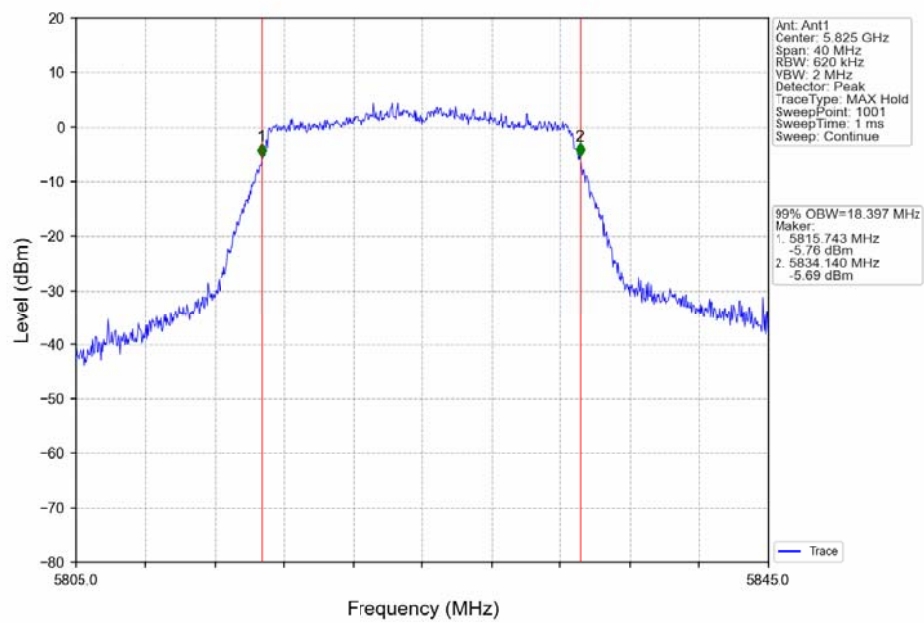
802.11ac(VHT20)_HCH_5825MHz_Ant1_NTNV
