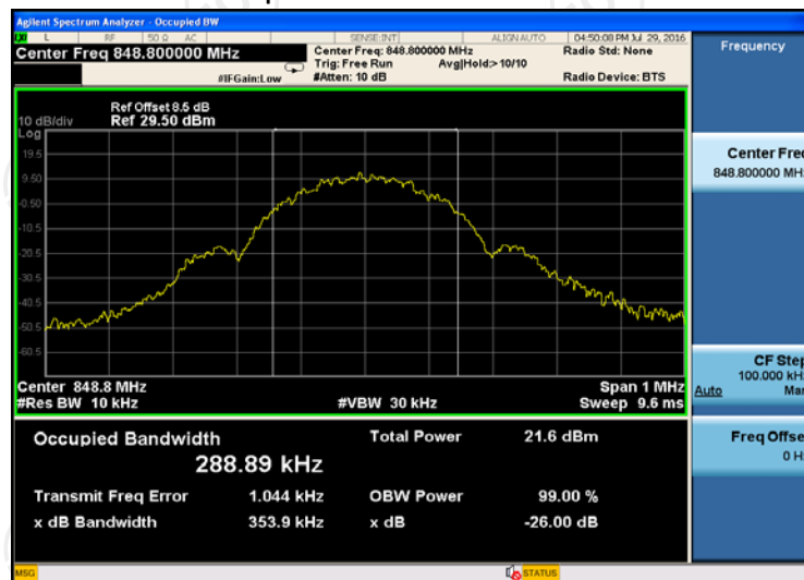
99%&26dB Occupied Bandwidth Plot on Channel 251
