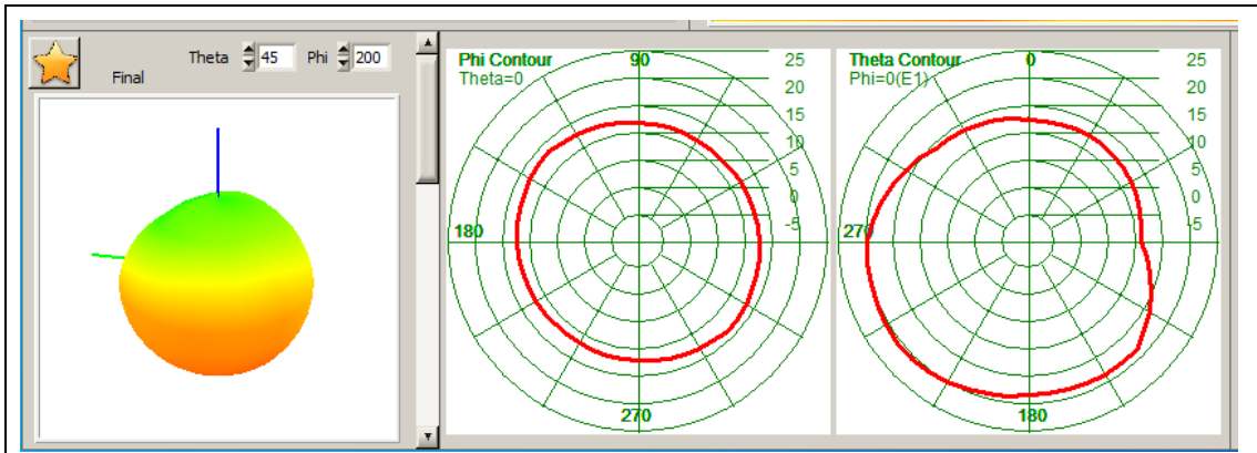
FDD-B28A
