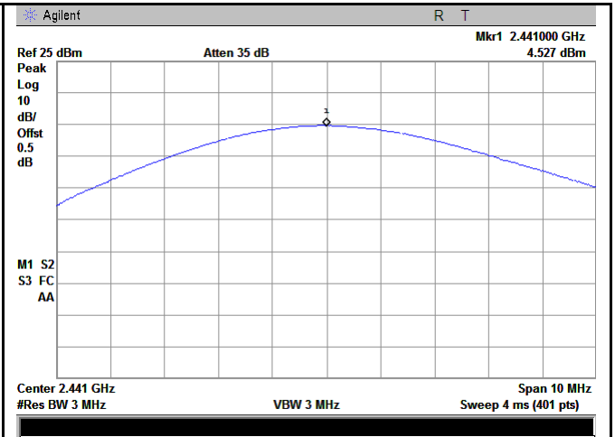
8DPSK Output power - Mid CH 2441
