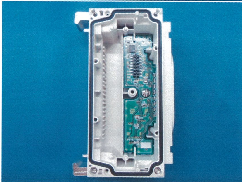
EX600-WSV1 Inside View
