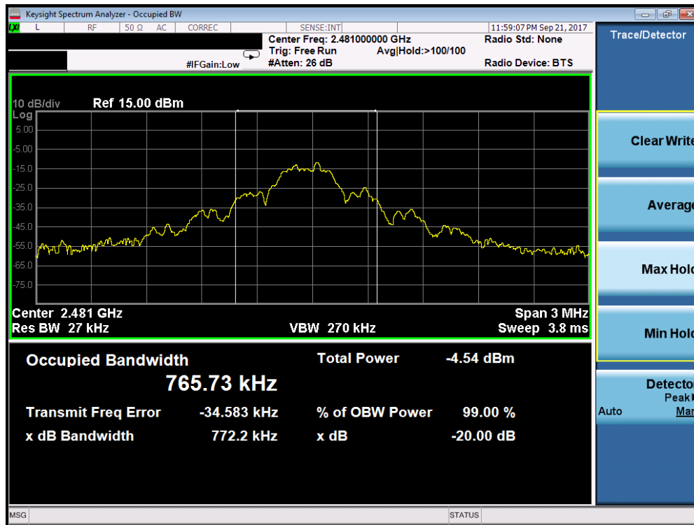
Plot 7-12. 20dB Bandwidth Plot (EX600-WSV2, Ch. 78)
