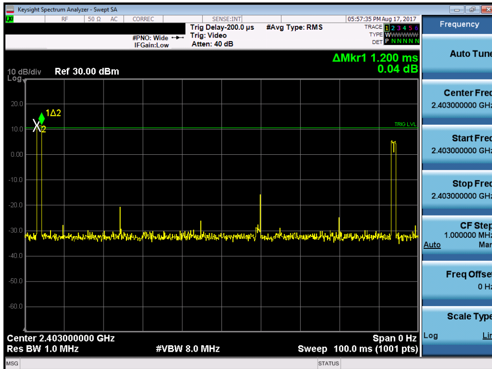
Plot 7-48. Time of Occupancy Plot (EX600-WSV2)
