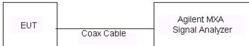
Figure 7-2. Test Instrument & Measurement Setup
