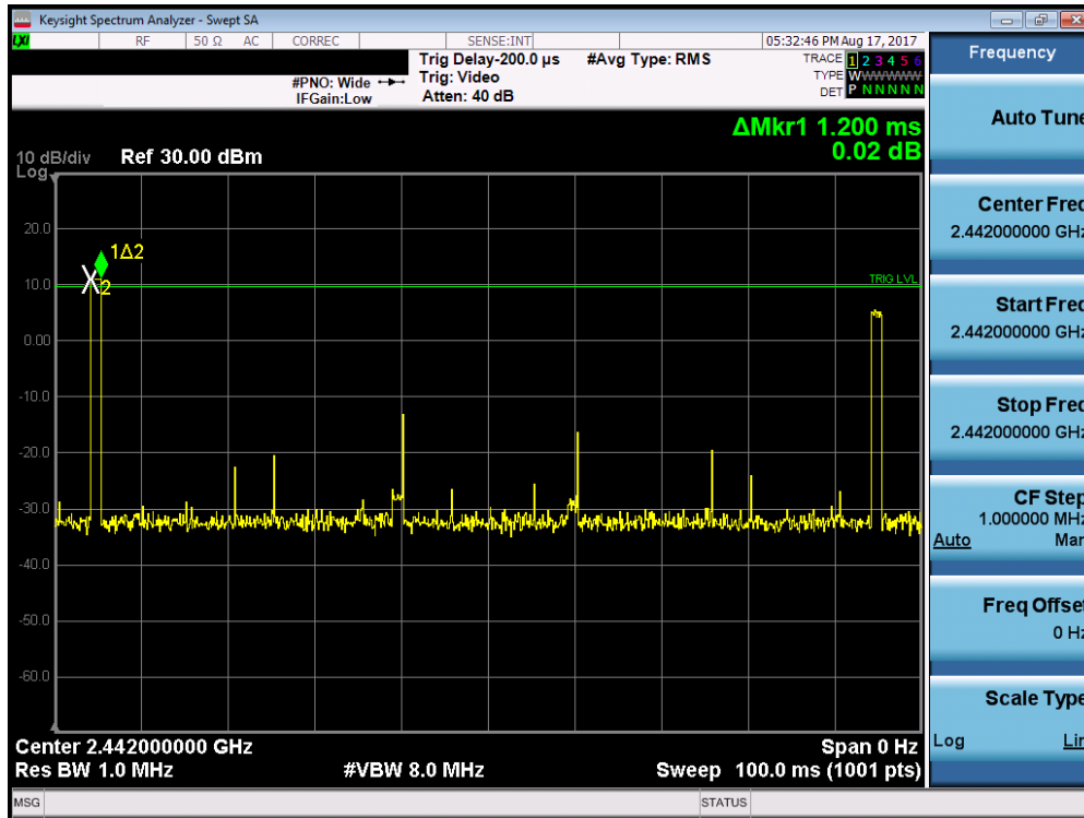
Plot 7-47. Time of Occupancy Plot (EX600-WSV1)
