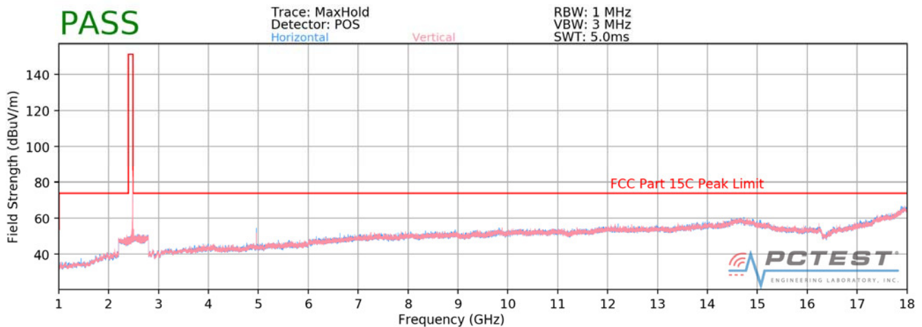
Plot 7-6. Radiated Spurious Plot above 1GHz (Ch. 78) – EX600-WPN2
