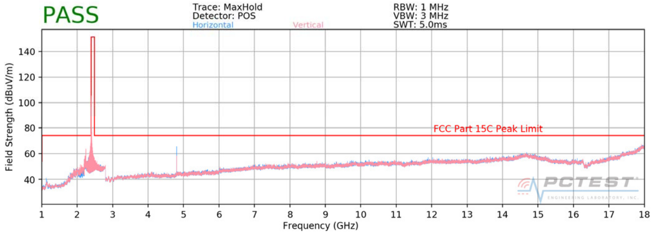
Plot 7-1. Radiated Spurious Plot above 1GHz (Ch. 0) – EX600-WPN1
