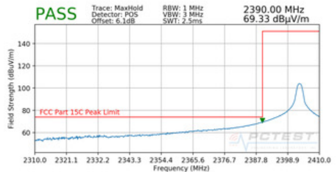
Plot 7-14. Radiated Restricted Lower Band Edge Measurement (Peak) – EX600-WPN2
