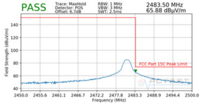
Plot 7-12. Radiated Restricted Upper Band Edge Measurement (Peak) – EX600-WPN1
