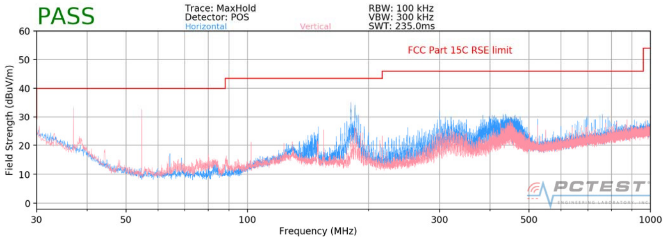
Plot 7-18. Radiated Spurious Plot below 1GHz (Pol. H) – EX600-WPN2
