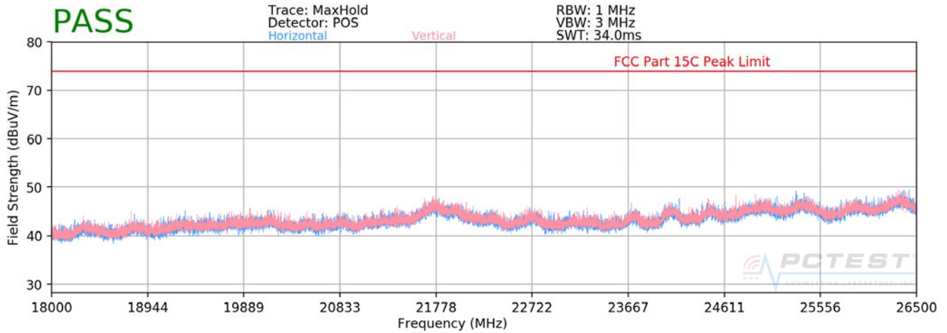
Plot 7-7. Radiated Spurious Plot above 18GHz – EX600-WPN1
