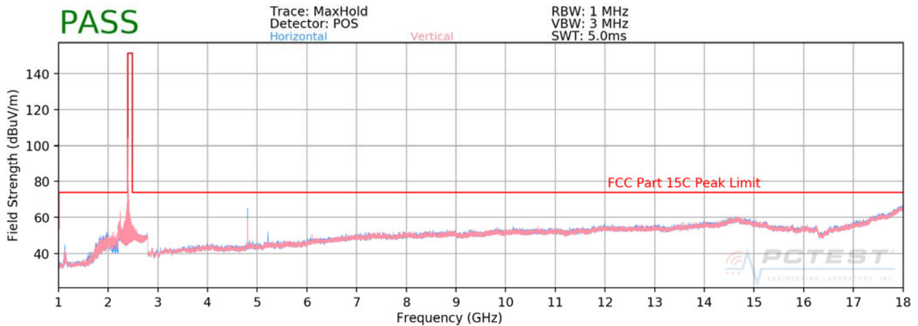
Plot 7-4. Radiated Spurious Plot above 1GHz (Ch. 0) – EX600-WPN2
