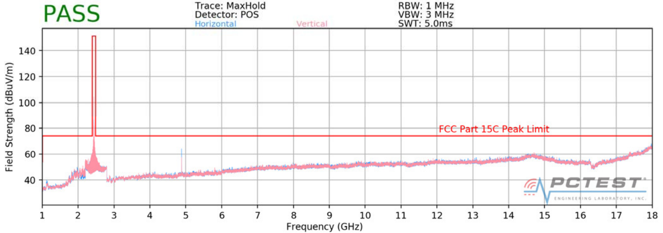
Plot 7-2. Radiated Spurious Plot above 1GHz (Ch. 39) – EX600-WPN1
