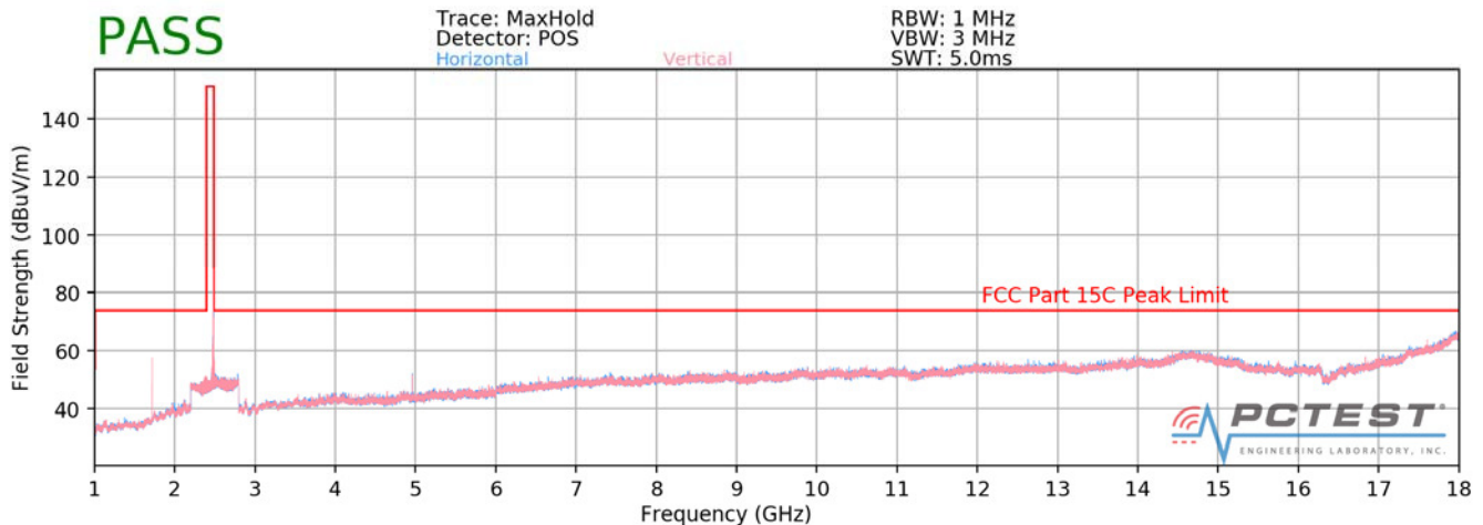
Plot 7-3. Radiated Spurious Plot above 1GHz (Ch. 78) – EX600-WPN1
