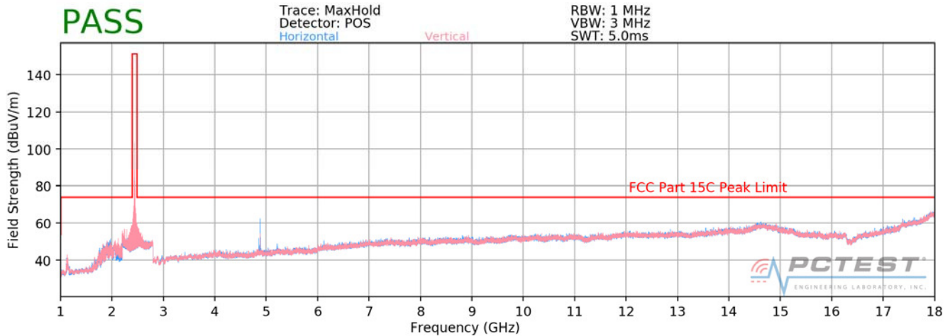
Plot 7-5. Radiated Spurious Plot above 1GHz (Ch. 39) – EX600-WPN2
