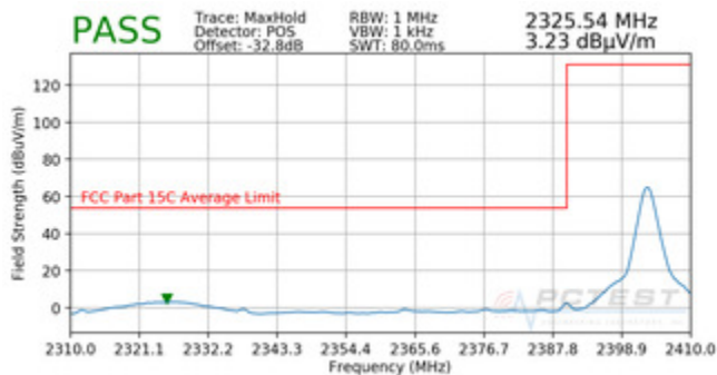
Plot 7-13. Radiated Restricted Lower Band Edge Measurement (Average) – EX600-WPN2
