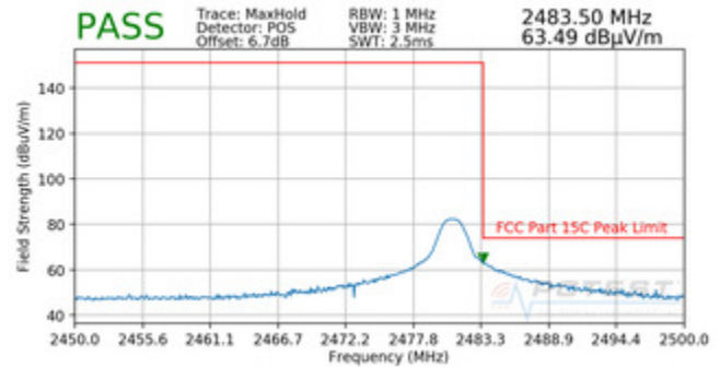
Plot 7-16. Radiated Restricted Upper Band Edge Measurement (Peak) – EX600-WPN2
