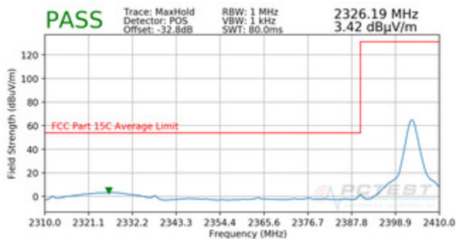
Plot 7-9. Radiated Restricted Lower Band Edge Measurement (Average) – EX600-WPN1
