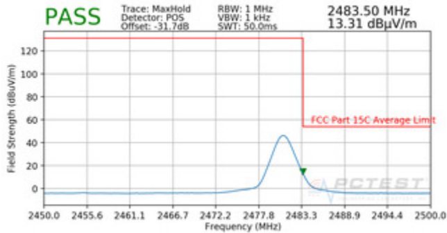
Plot 7-11. Radiated Restricted Upper Band Edge Measurement (Average) – EX600-WPN1
