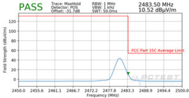
Plot 7-15. Radiated Restricted Upper Band Edge Measurement (Average) – EX600-WPN2
