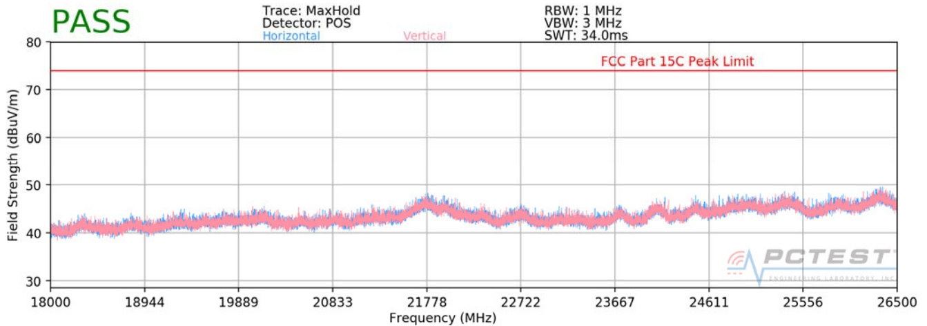
Plot 7-8. Radiated Spurious Plot above 18GHz – EX600-WPN2
