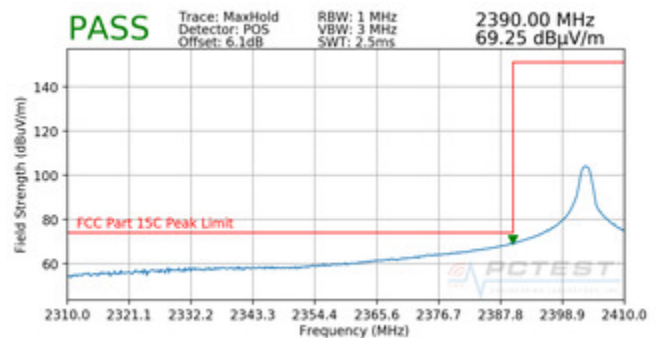
Plot 7-10. Radiated Restricted Lower Band Edge Measurement (Peak) – EX600-WPN1
