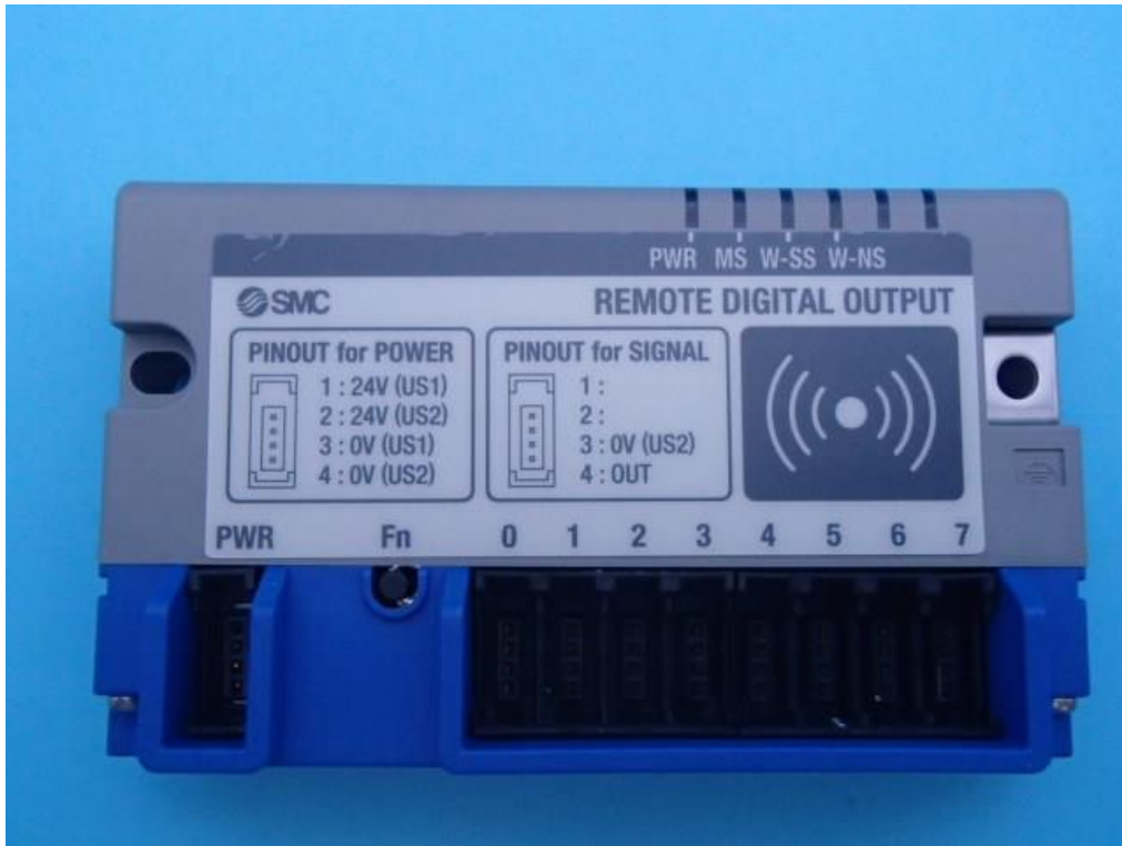
EX600-WDYE1 Front side
