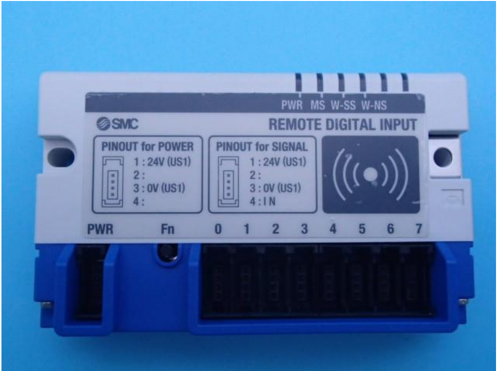
EX600-WDXE1 Front side
