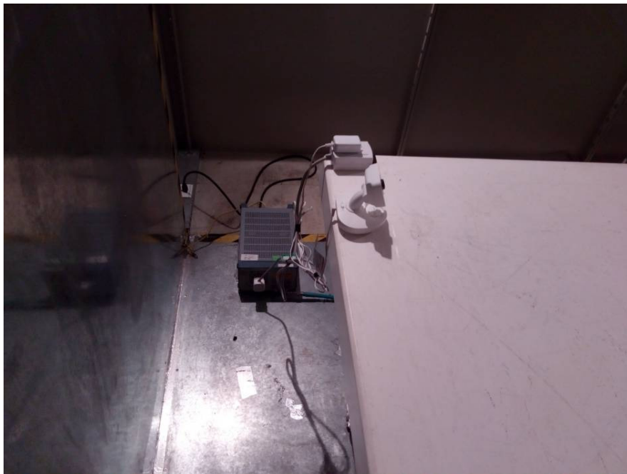
Conducted Emissions - Side View (Transmitting)
