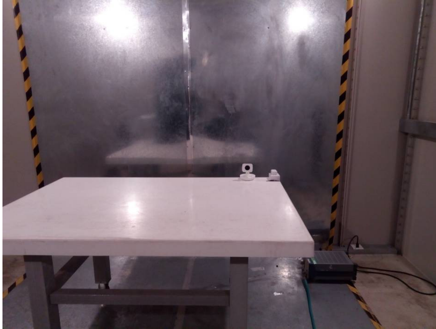
Conducted Emissions - Front View (Transmitting)
