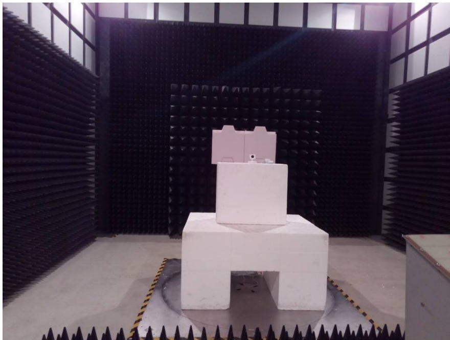
Radiated Emissions Tested View (Above 1GHz, Transmitting)
