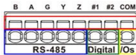
Figure 3: Maestro Router LAN Panel I/O connector
