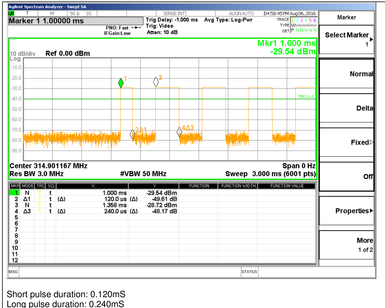
Figure 7 Pulse Train Graphs for 314.9MHz (ASK modulation)
