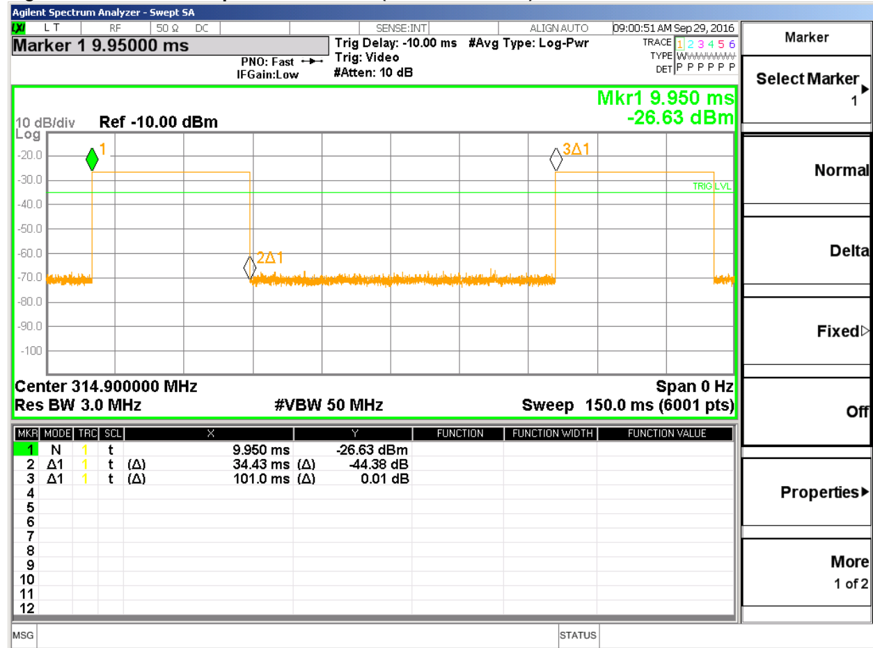
Figure 8 Pulse Train Graphs for 314.9MHz (FSK modulation)
