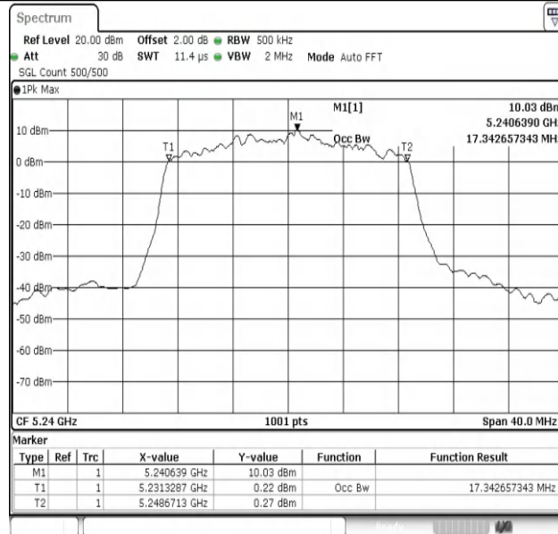
11N20SISO-Ant1-5240
