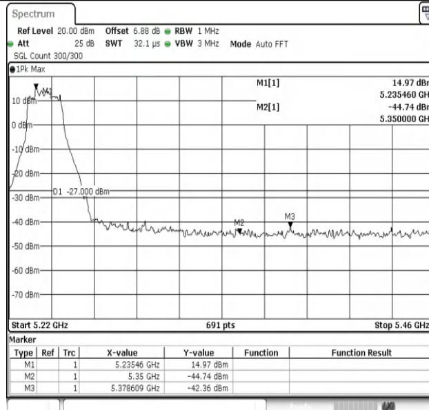
11AC20SISO-Ant1-5240-PASS
