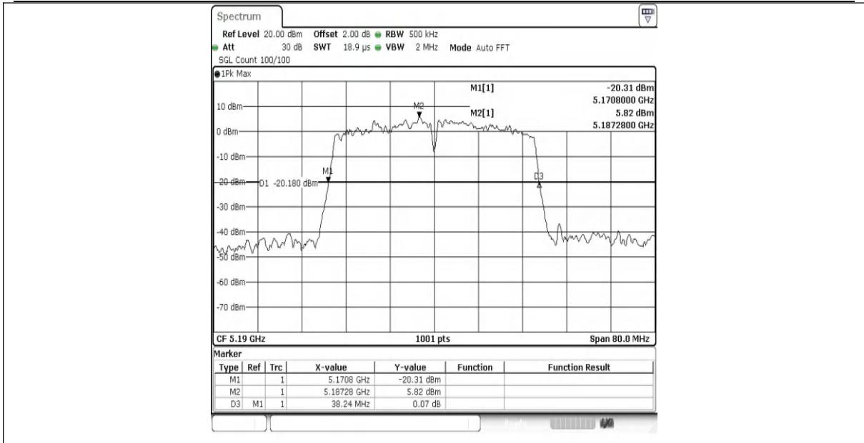
11N40SISO-Ant1-5190
