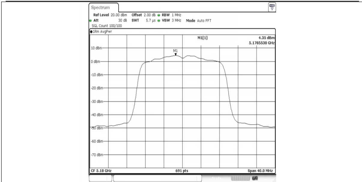
11AC20SISO-Ant1-5180-PASS
