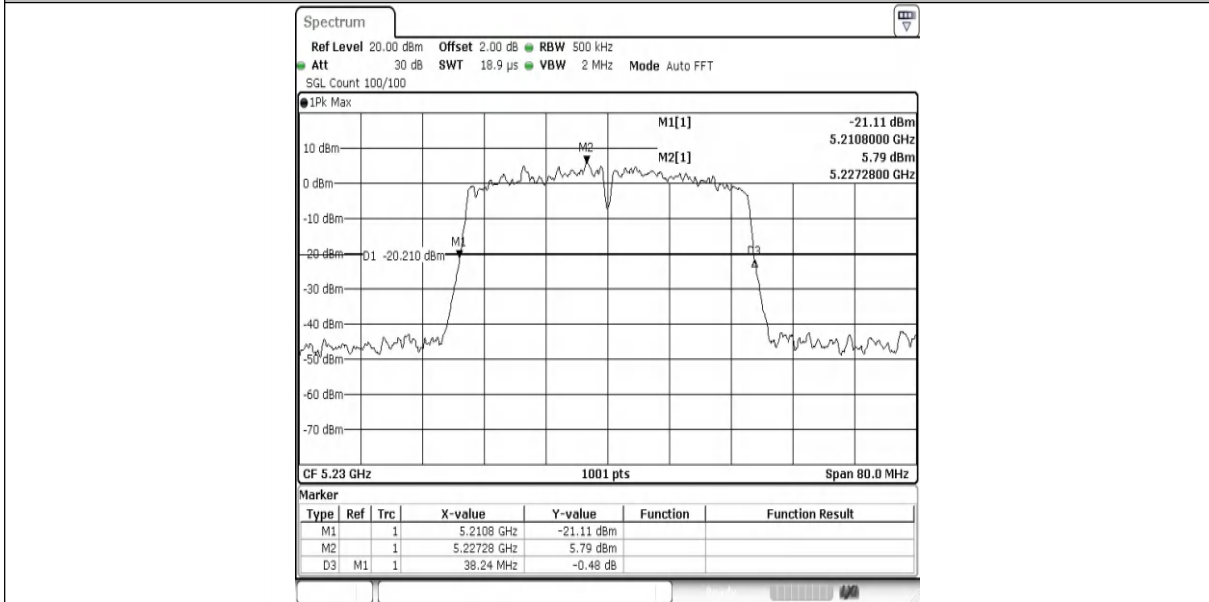
11N40SISO-Ant1-5230
