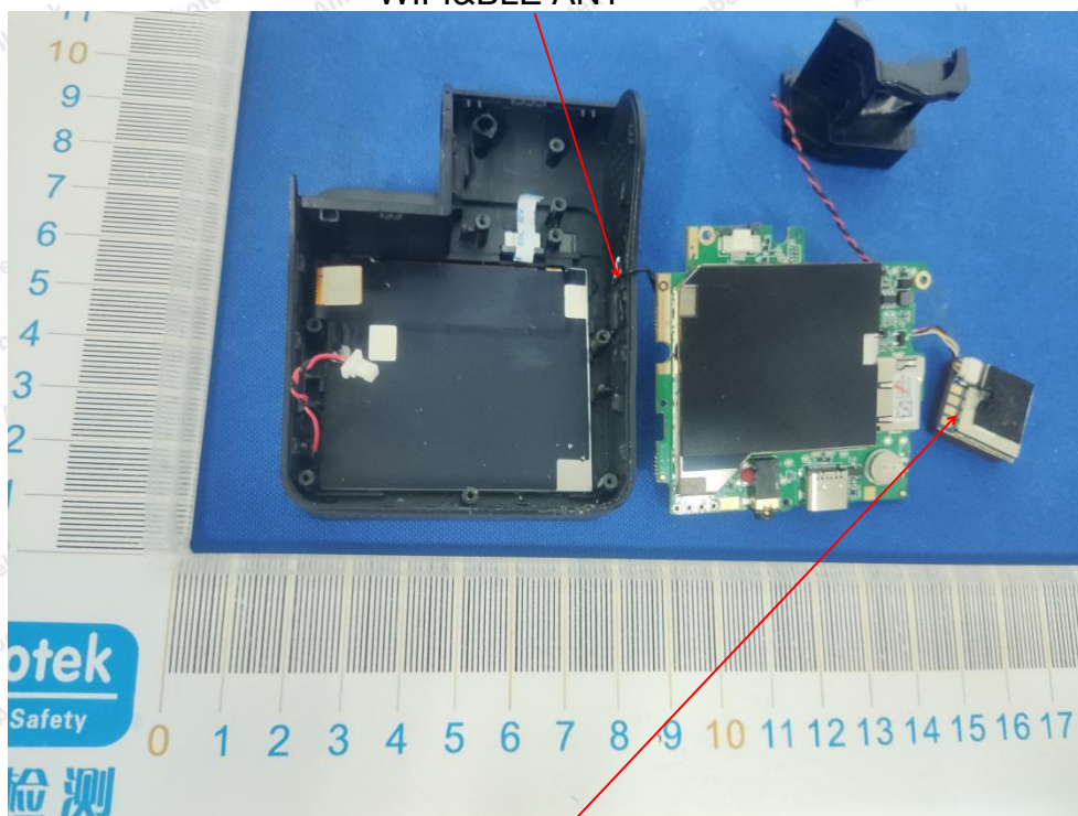
WIFI&BLE ANT
