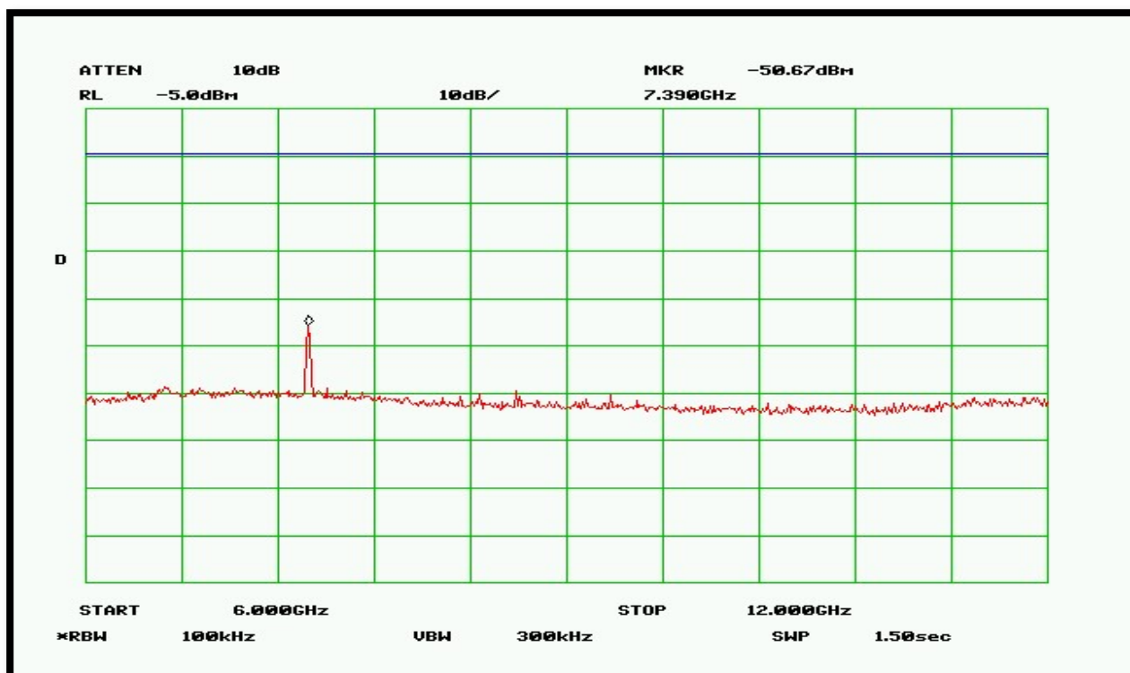
Plot 45 – 802.11n (20 MHz) Highest Channel – 6GHz to 12GHz
