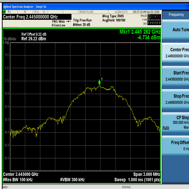
SRD-Ant1-2445-0~Reference-PASS
