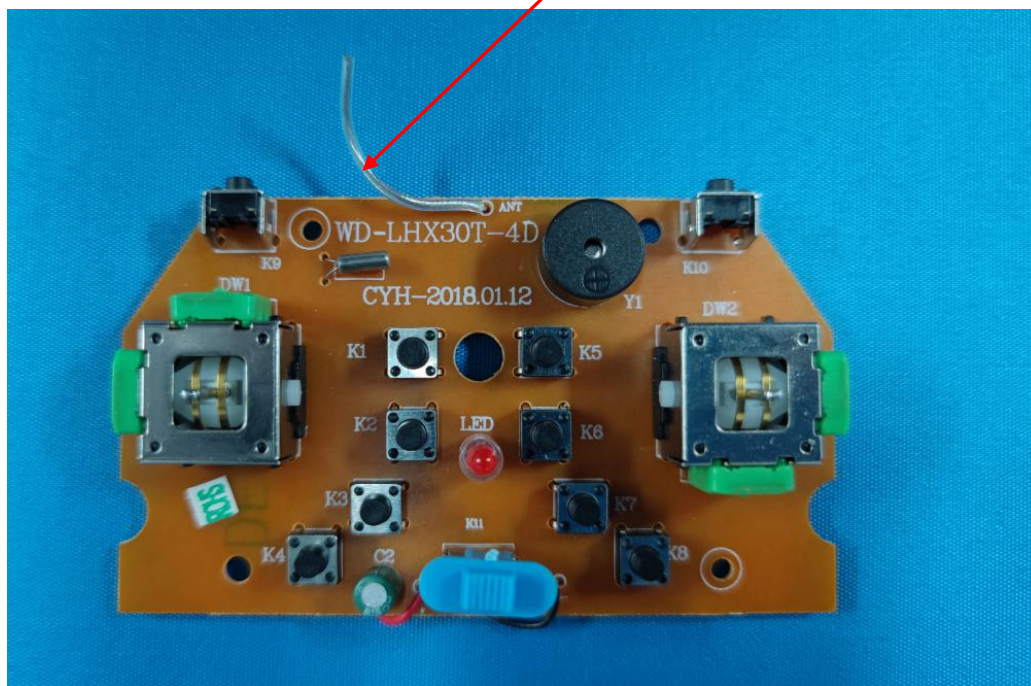
Extension line Antenna
