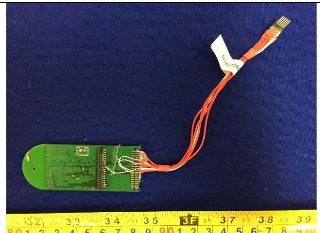
Interface board Bottom View
