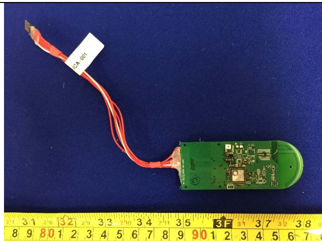
Interface board Top View
