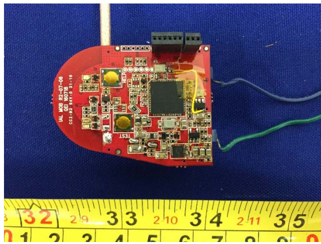
PCB Top View
