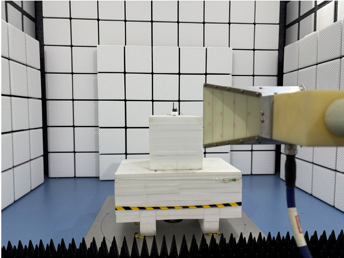
Radiation Emission_ Above 18GHz - Front View
