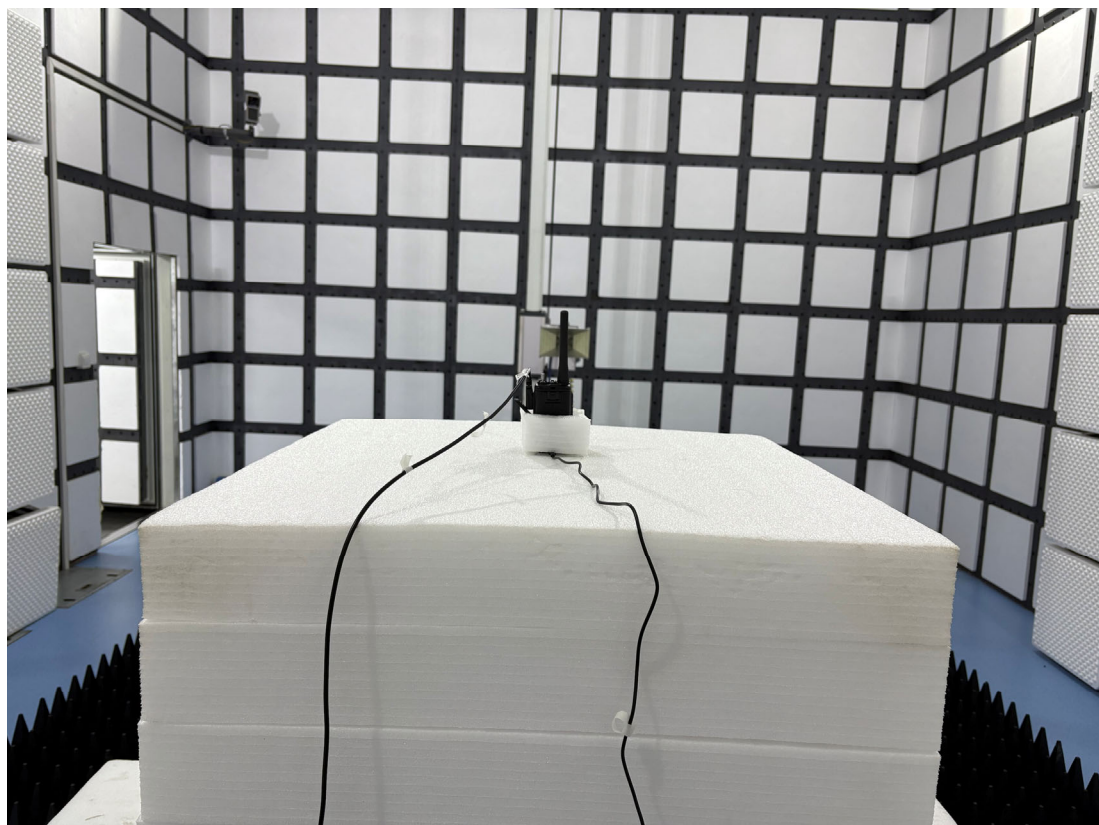
Radiation Emission_1GHz-18GHz - Front View
