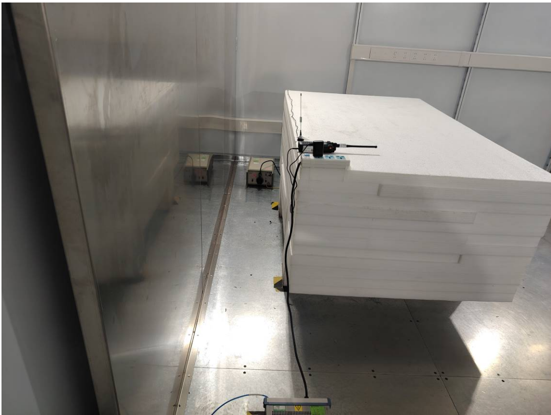
Conducted Emission_Side View(Mode 2)
