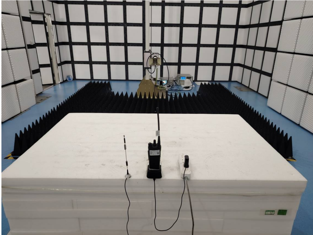
Radiation Emission_ Above 1GHz - Rear View (Mode 3)
