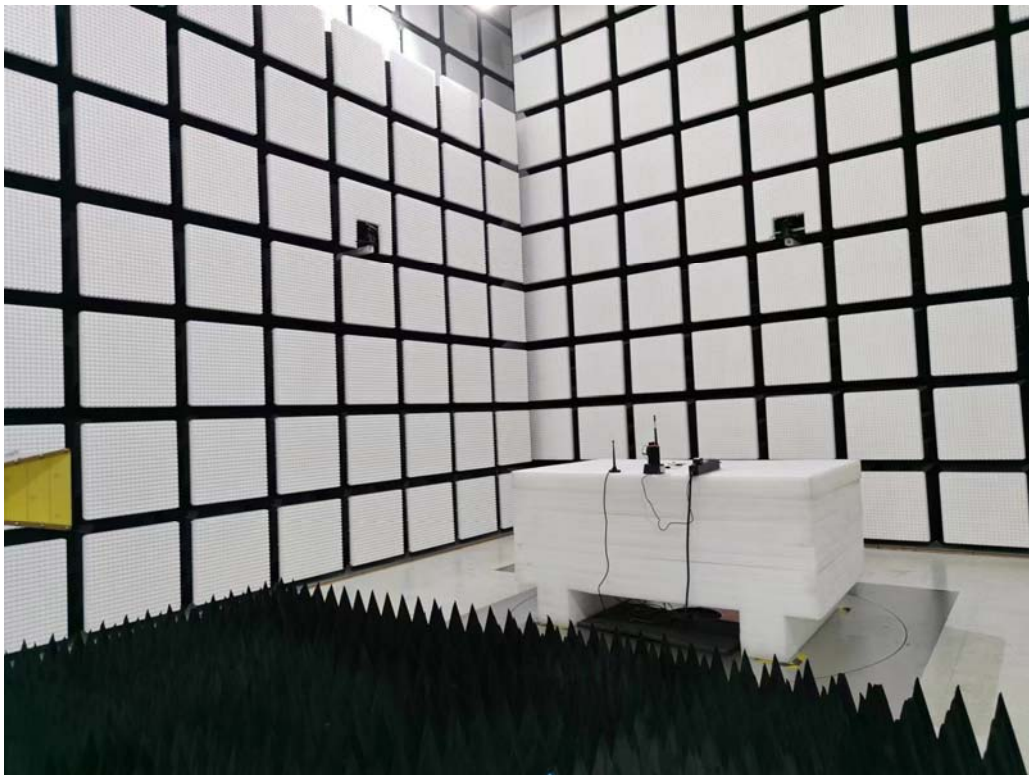
Radiated Emission Above 1GHz Rear View M1,M3,M4
