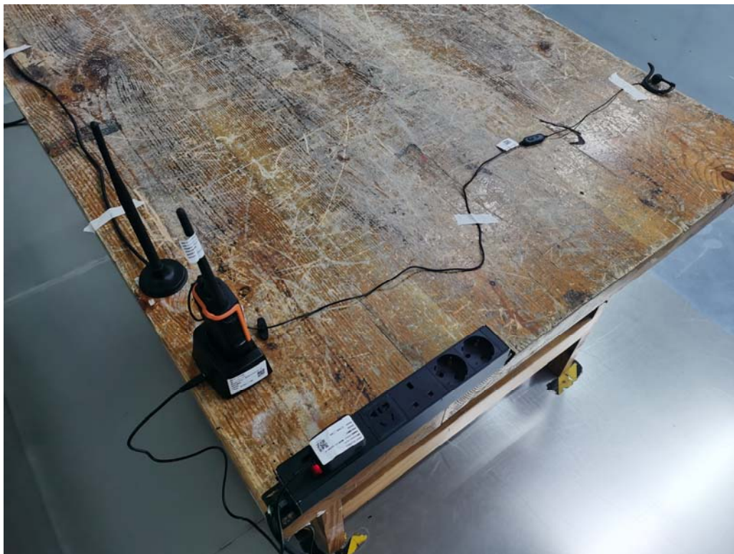
Conducted Emissions Side View M1,M3,M4
