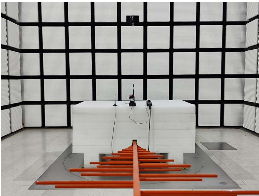
Radiated Emission Below 1GHz Rear View M1,M3,M4
